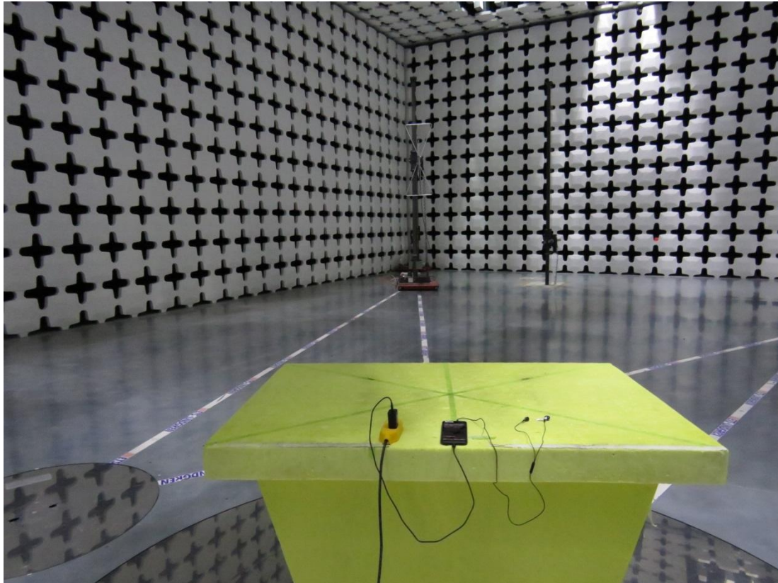
30MHz-1GHz
