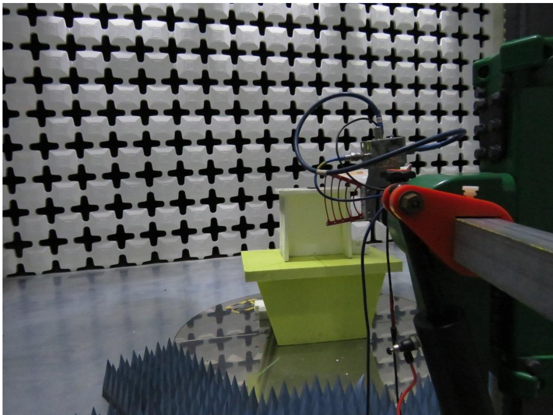
Above 1GHz
