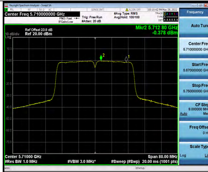
11AC40SISO_Ant1_5710_UNII-3
