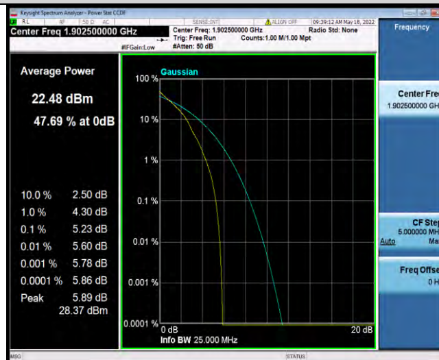
Band2-15MHz-QPSK-19125-75RB#0
