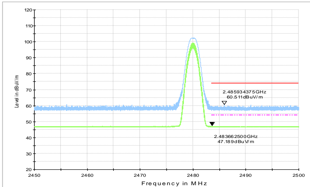
Fig.4. Frequency Band Edges: BLE GFSK, 2480 MHz, Hopping Off , 2.45 GHz - 2.50GHz
