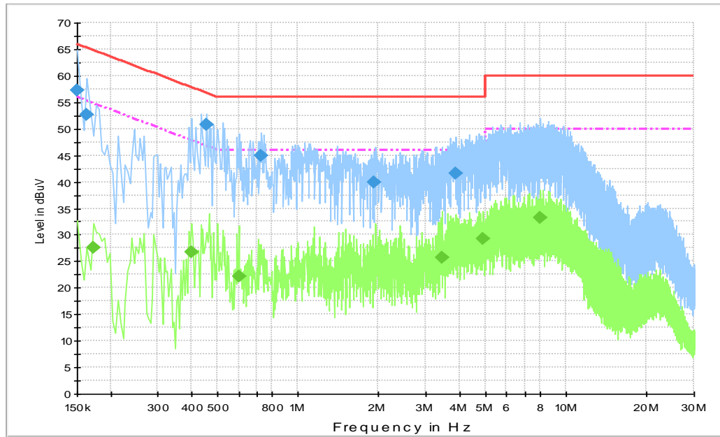
Fig.B.9.1 AC Powerline Conducted Emission- Bluetooth BLE
