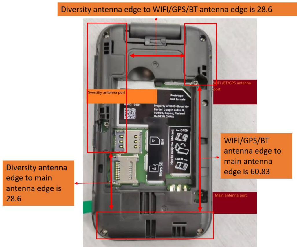
Picture 19: Antenna location
