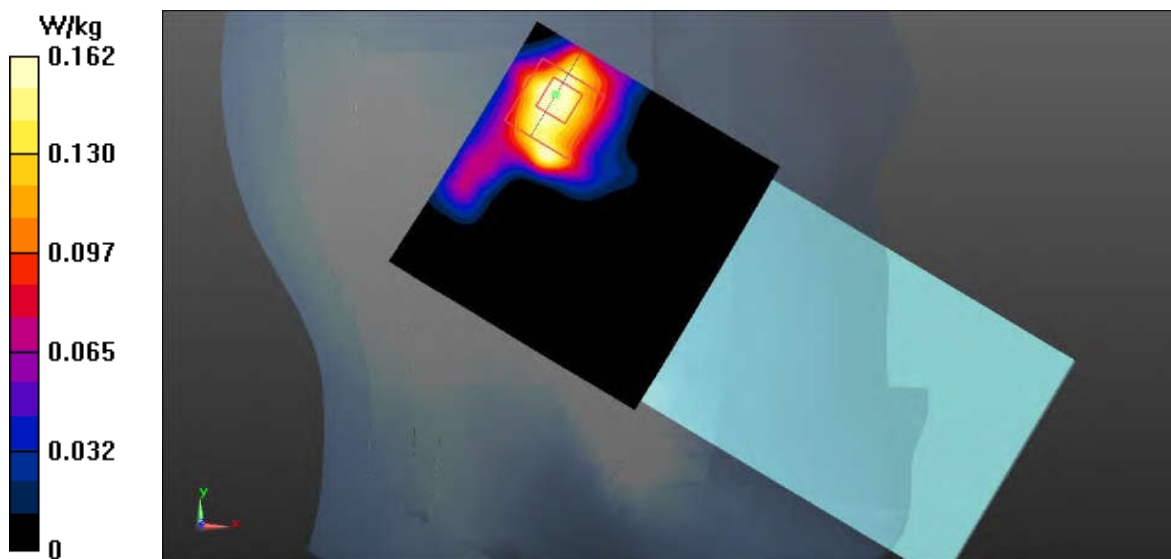
Fig.29 WLAN 5GHz Head
