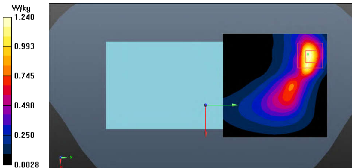
Fig.16 LTE Band 7 Body
