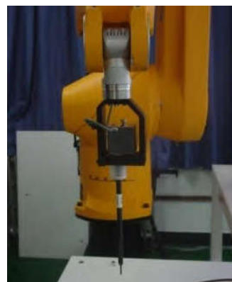
Picture C.3 E-field Probe
