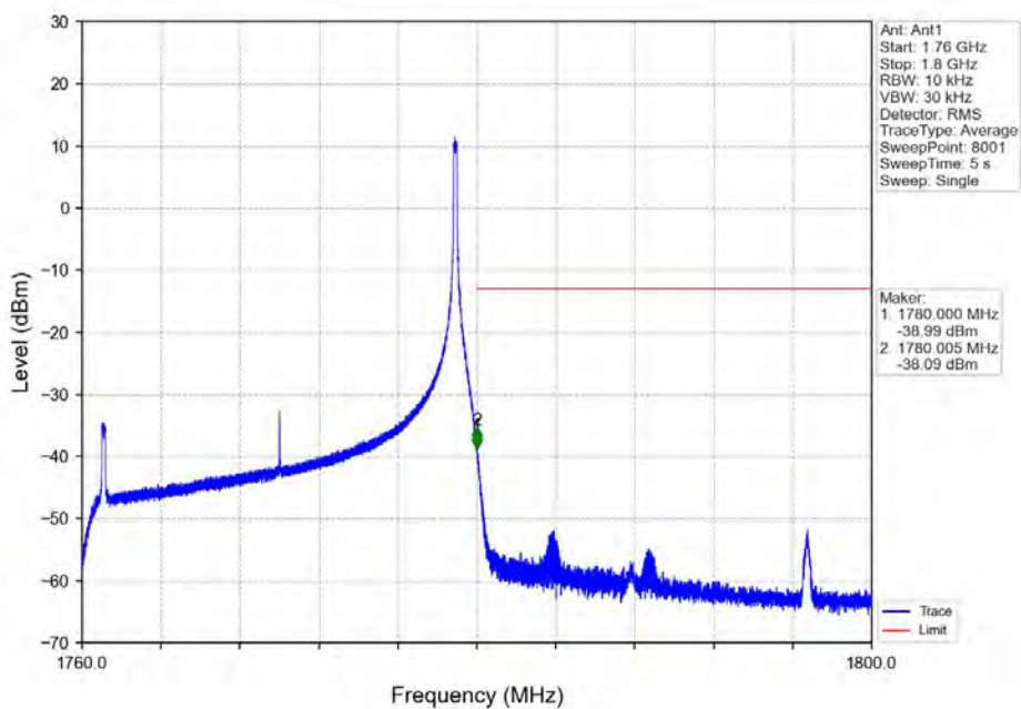
Band66_20MHz_16QAM_HCH_1770MHz_RB_100_0_NTNV
