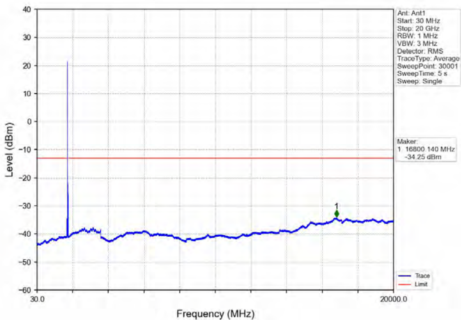
Band66_20MHz_64QAM_MCH_1745MHz_RB_1_0_NTNV
