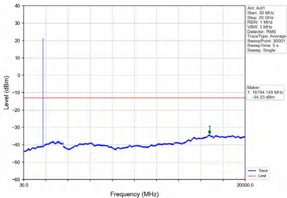
Band66_1.4MHz_16QAM_HCH_1779.3MHz_RB_1_0_NTNV
