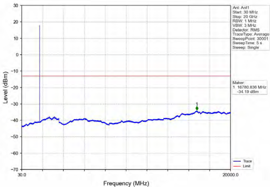
Band66_1.4MHz_64QAM_MCH_1745MHz_RB_1_0_NTNV
