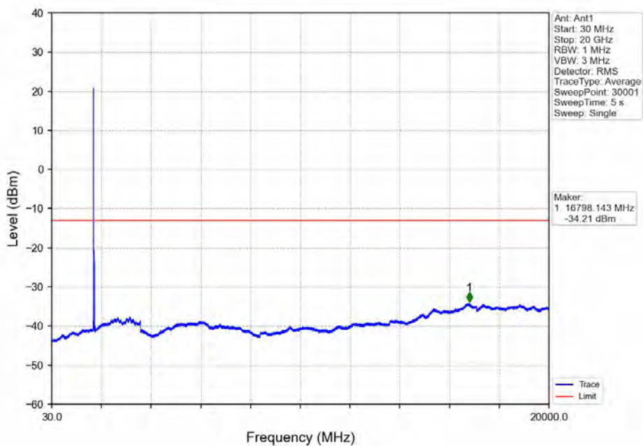
Band66_20MHz_64QAM_LCH_1720MHz_RB_1_0_NTNV
