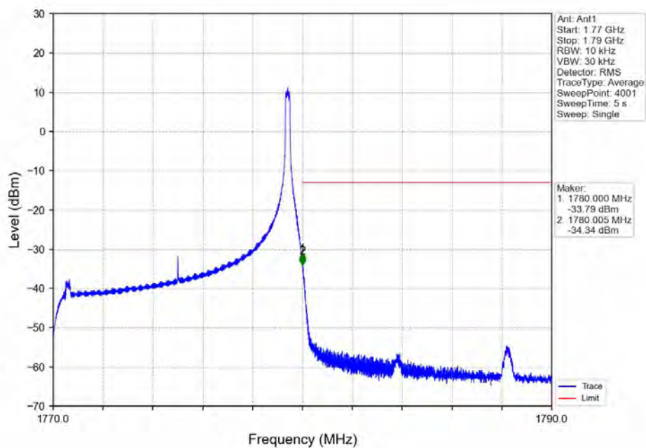
Band66_10MHz_16QAM_HCH_1775MHz_RB_50_0_NTNV
