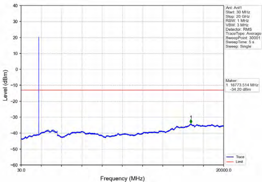
Band66_5MHz_64QAM_HCH_1777.5MHz_RB_1_24_NTNV
