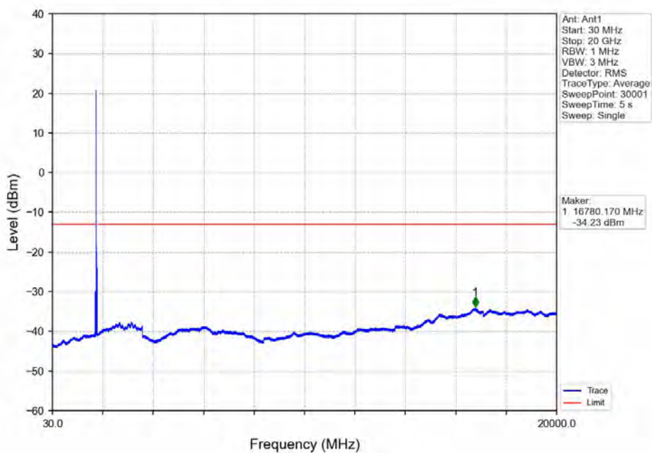
Band66_20MHz_64QAM_HCH_1770MHz_RB_1_99_NTNV
