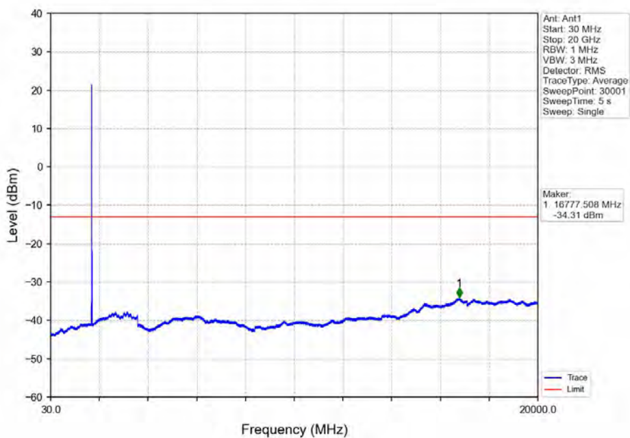
Band66_10MHz_16QAM_LCH_1715MHz_RB_50_0_NTNV
