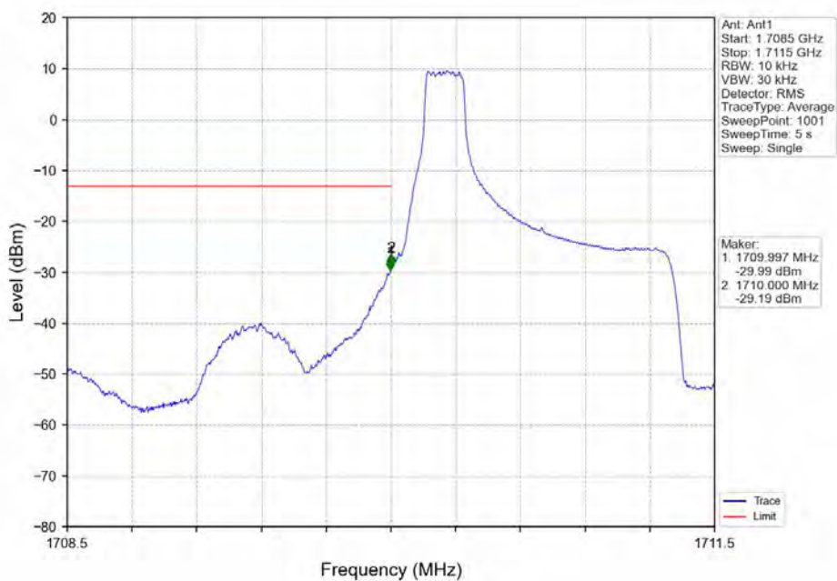
Band66_1.4MHz_64QAM_LCH_1710.7MHz_RB_1_0_NTNV
