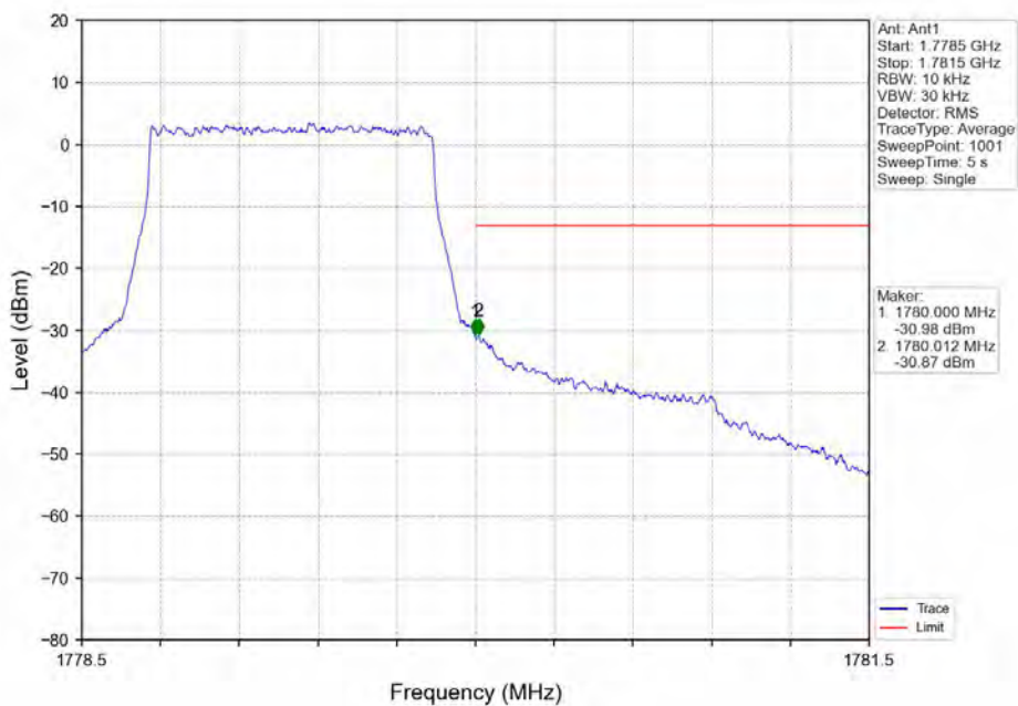
Band66_1.4MHz_64QAM_HCH_1779.3MHz_RB_1_5_NTNV
