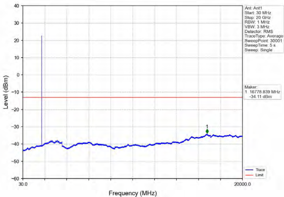
Band66_1.4MHz_QPSK_MCH_1745MHz_RB_1_0_NTNV
