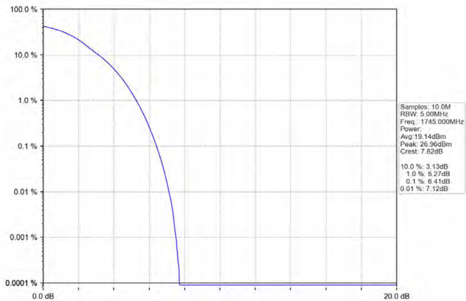
Band66_10MHz_64QAM_MCH_1745MHz_RB_50_0_NTNV
