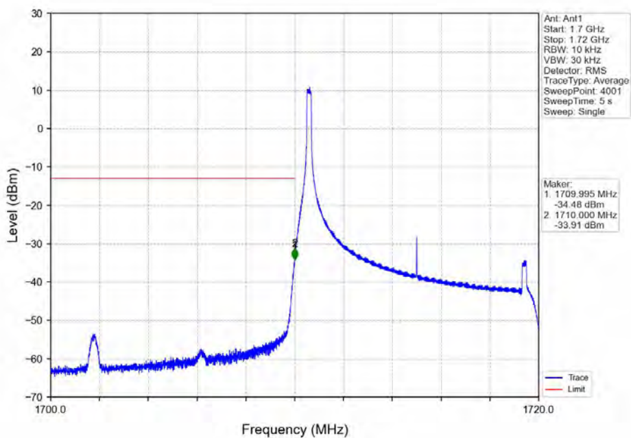
Band66_10MHz_64QAM_LCH_1715MHz_RB_1_0_NTNV
