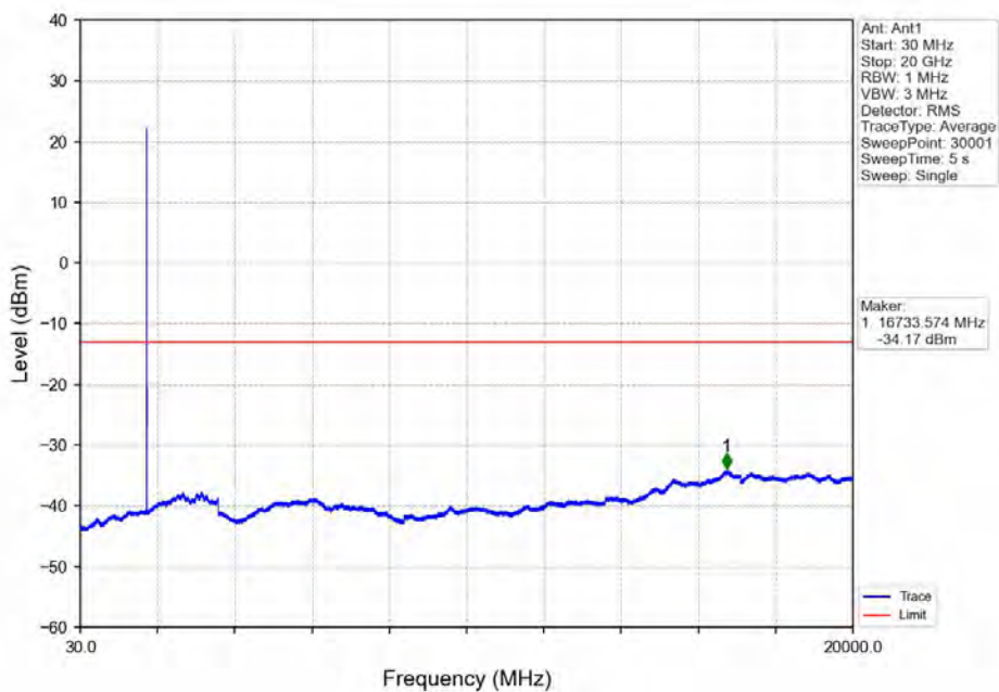
Band66_3MHz_QPSK_MCH_1745MHz_RB_1_0_NTNV
