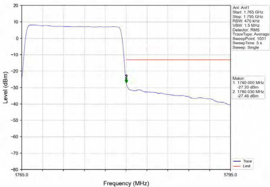
Band66_15MHz_16QAM_HCH_1772.5MHz_RB_75_0_NTNV
