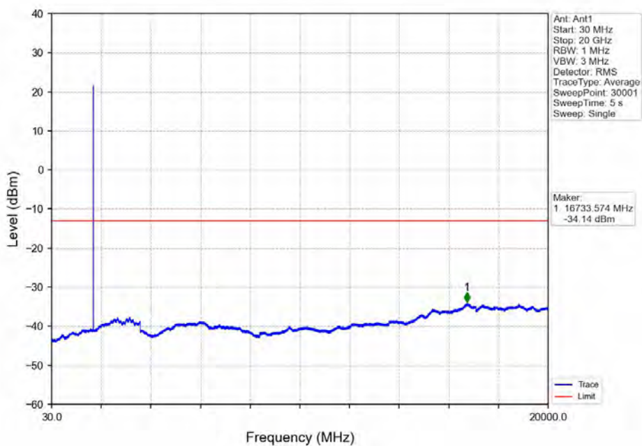
Band66_1.4MHz_16QAM_LCH_1710.7MHz_RB_6_0_NTNV
