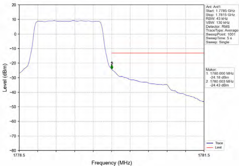
Band66_1.4MHz_16QAM_HCH_1779.3MHz_RB_6_0_NTNV
