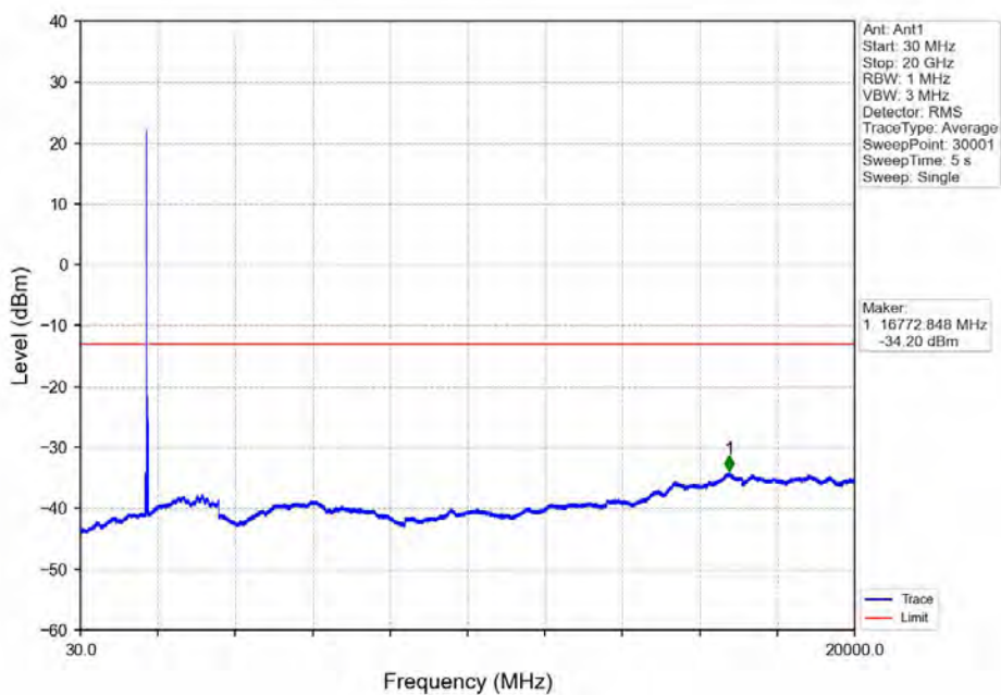
Band66_20MHz_16QAM_HCH_1770MHz_RB_1_0_NTNV
