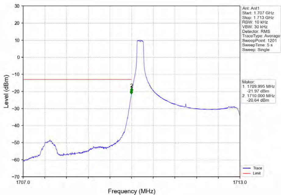
Band66_3MHz_64QAM_LCH_1711.5MHz_RB_1_0_NTNV
