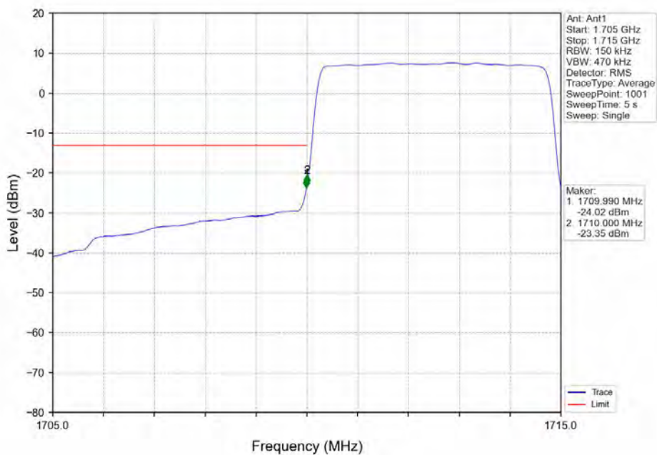
Band66_5MHz_16QAM_LCH_1712.5MHz_RB_25_0_NTNV
