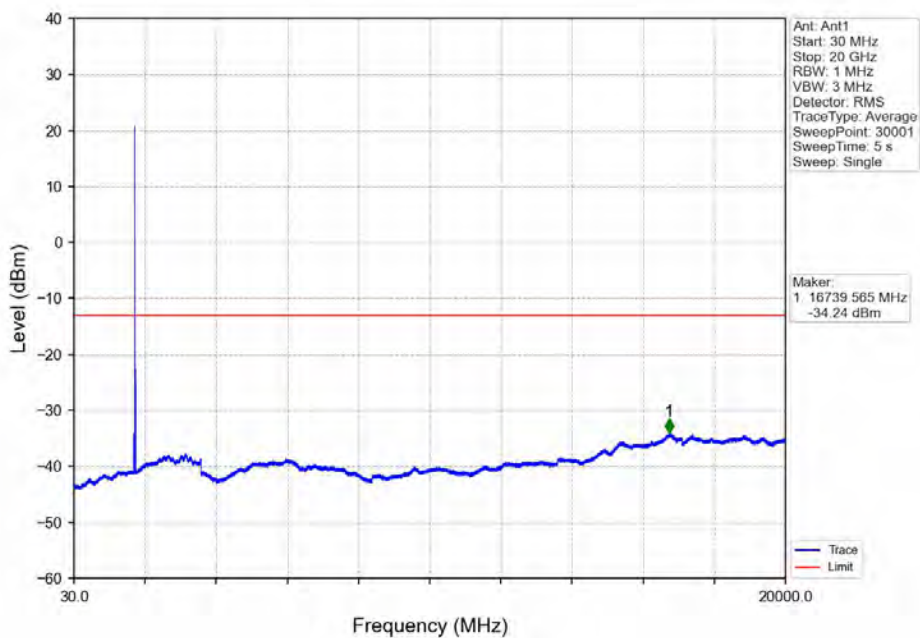
Band66_15MHz_64QAM_MCH_1745MHz_RB_1_0_NTNV
