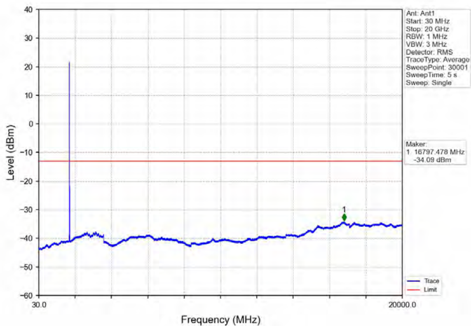
Band66_15MHz_64QAM_LCH_1717.5MHz_RB_1_0_NTNV
