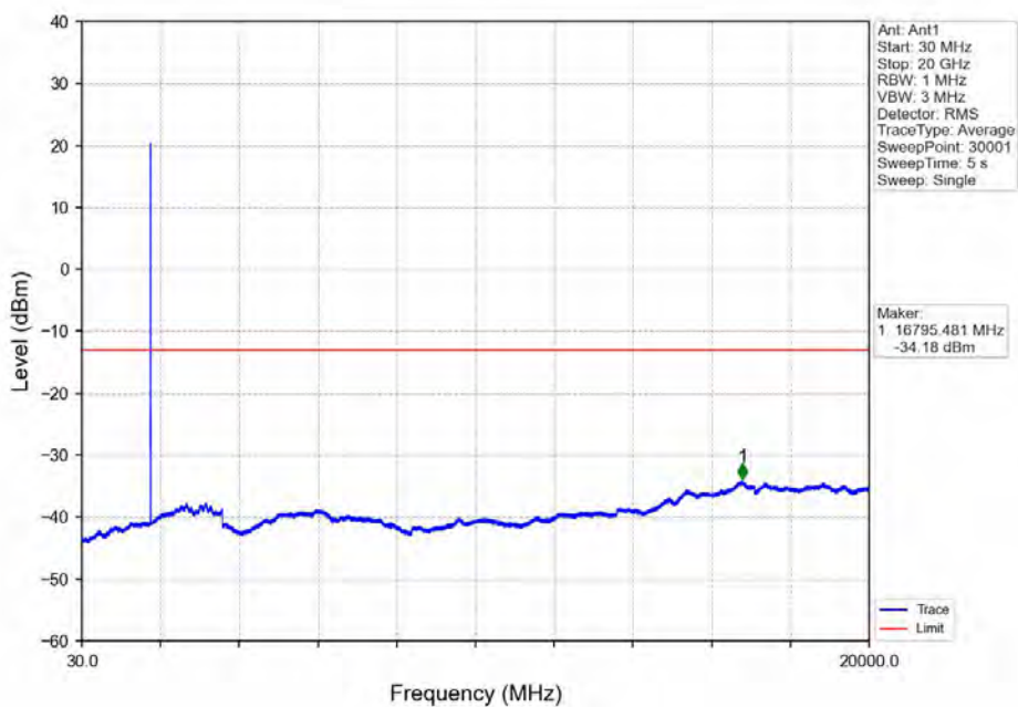
Band66_3MHz_64QAM_HCH_1778.5MHz_RB_1_14_NTNV
