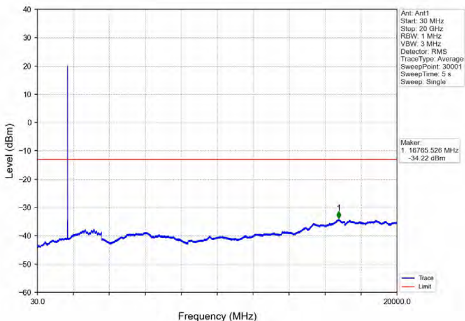
Band66_5MHz_64QAM_LCH_1712.5MHz_RB_1_0_NTNV
