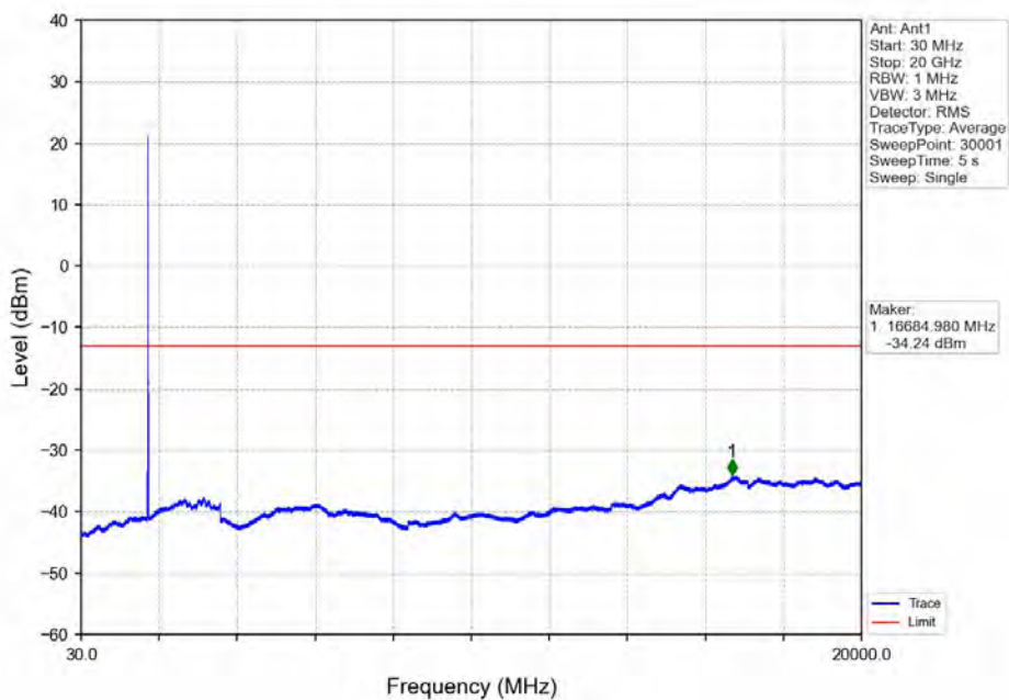
Band66_10MHz_64QAM_MCH_1745MHz_RB_1_0_NTNV
