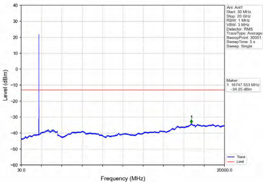
Band66_10MHz_16QAM_HCH_1775MHz_RB_1_0_NTNV
