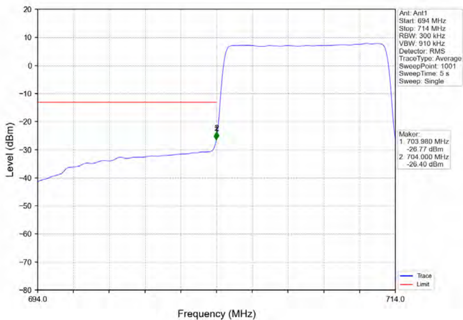
Band17_10MHz_16QAM_LCH_709MHz_RB_50_0_NTNV
