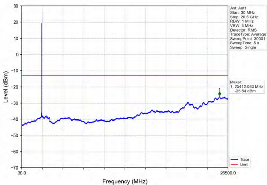
Band7_10MHz_64QAM_HCH_2565MHz_RB_1_49_NTNV
