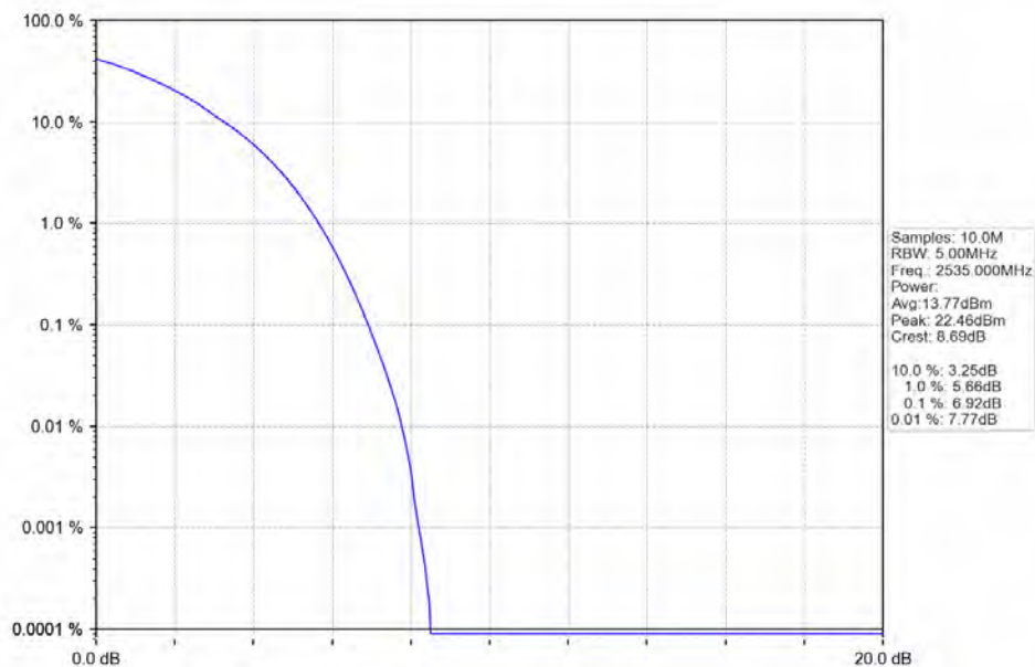
Band7 15MHz 64QAM MCH 2535MHz RB 75 0 NTV
