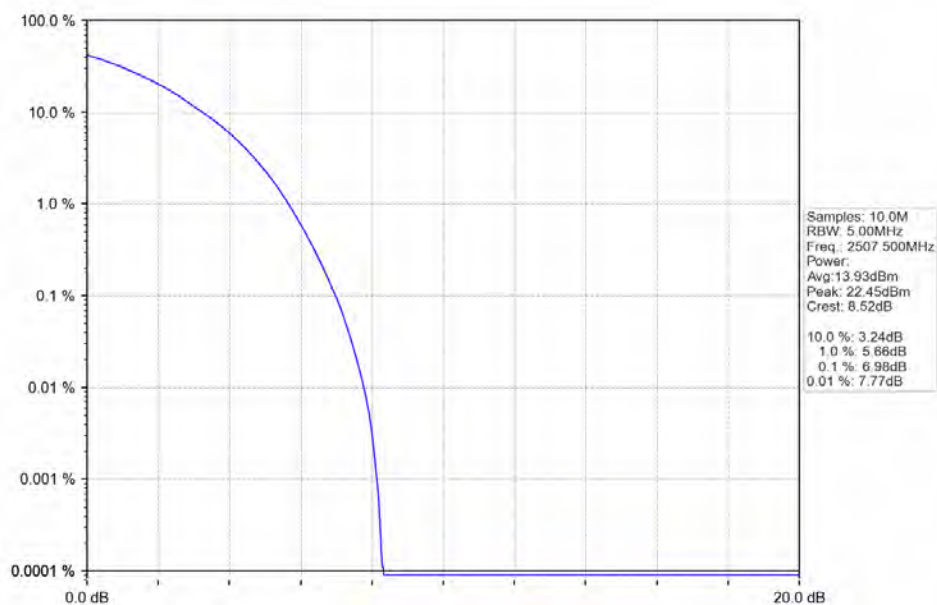
Band7 15MHz 64QAM LCH 2507.5MHz RB 75 0 NTV
