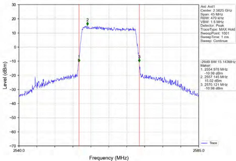
Band7 15MHz 16QAM HCH 2562.5MHz RB 75 0 NTVN
