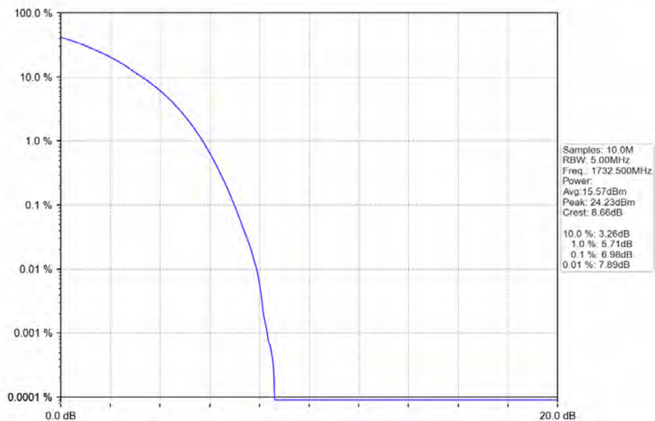
Band4 15MHz 64QAM MCH 1732.5MHz RB 75 0 NTN
