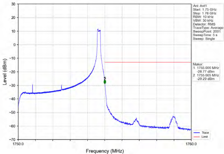
Band4_5MHz_QPSK_HCH_1752.5MHz_RB_1_24_NTNV
