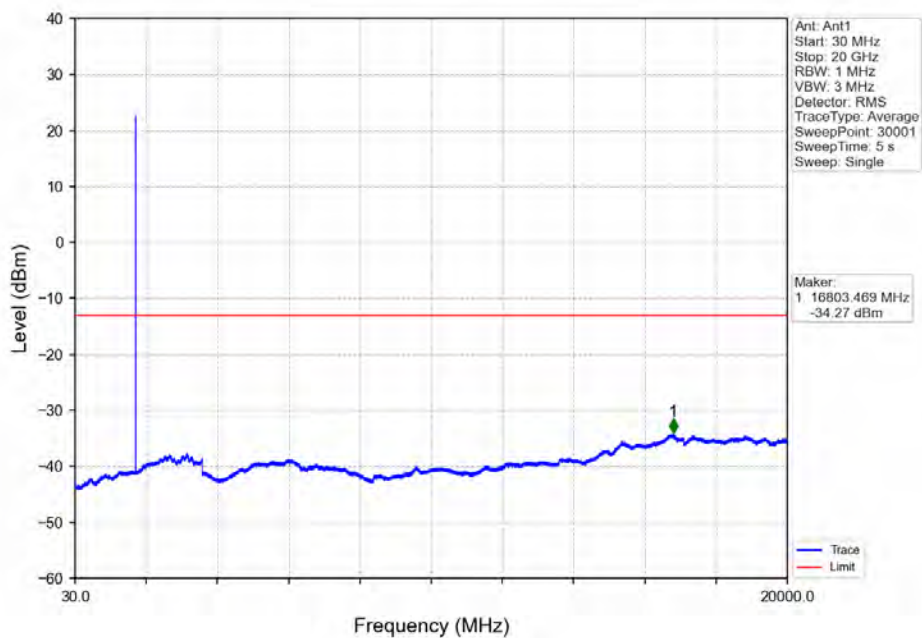
Band4_1.4MHz_QPSK_MCH_1732.5MHz_RB_1_0_NTNV
