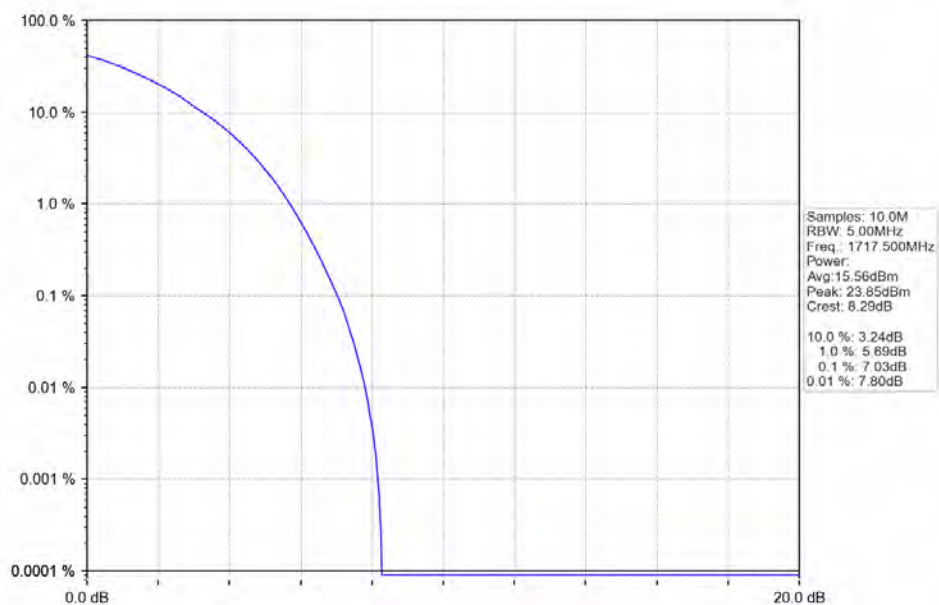
Band4 15MHz 64QAM LCH 1717.5MHz RB 75 0 NTN
