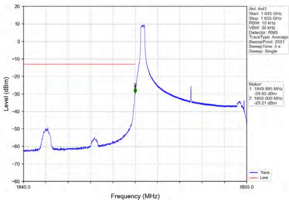
Band2_5MHz_64QAM_LCH_1852.5MHz_RB_1_0_NTNV
