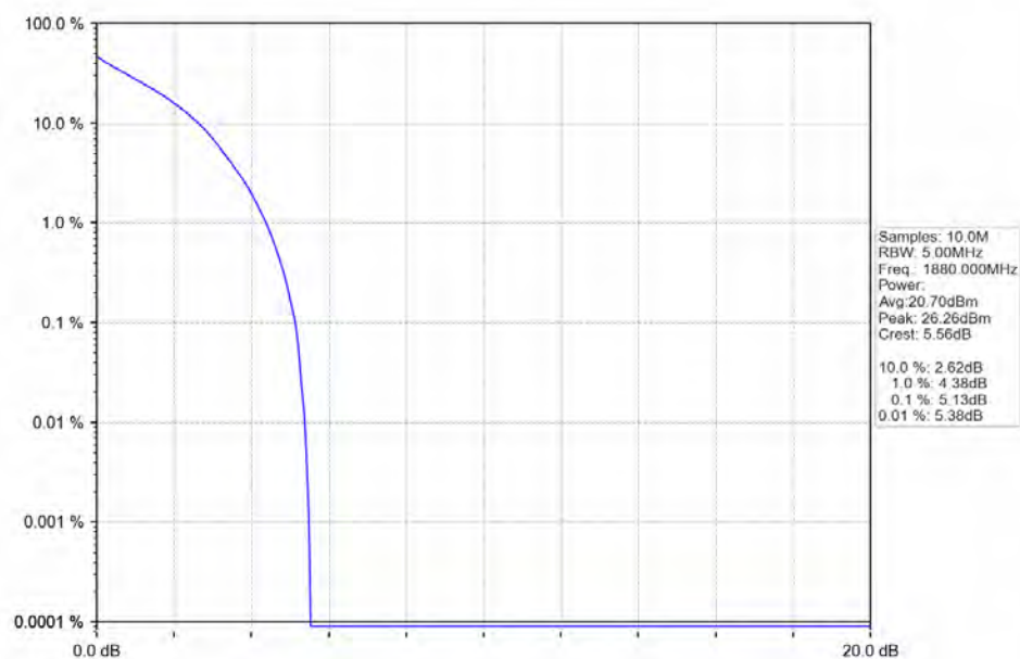
Band2_1.4MHz_QPSK_MCH_1880MHz_RB_6_0_NTNV
