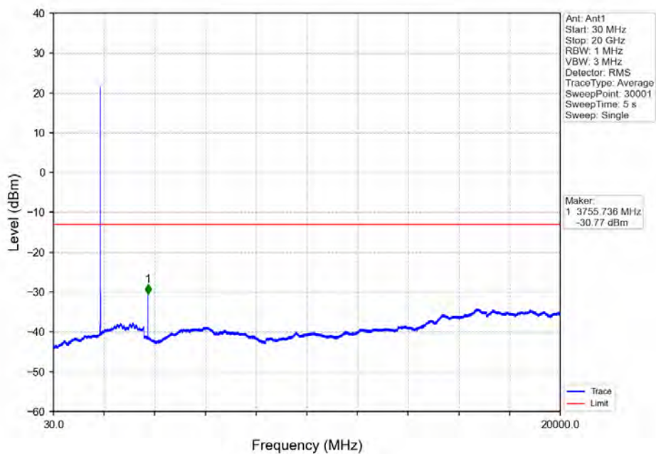
Band2_5MHz_64QAM_MCH_1880MHz_RB_1_0_NTNV
