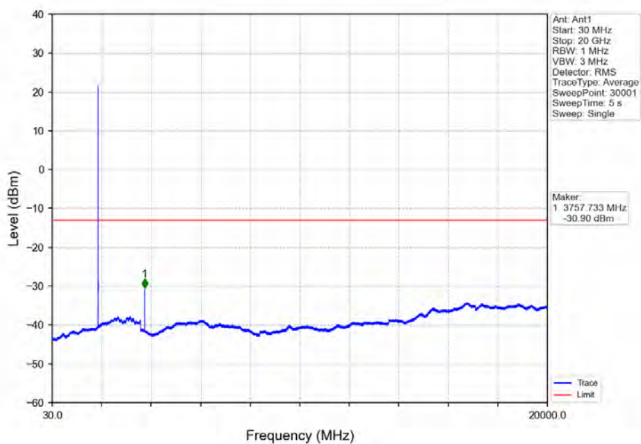
Band2_3MHz_16QAM_HCH_1908.5MHz_RB_1_0_NTNV
