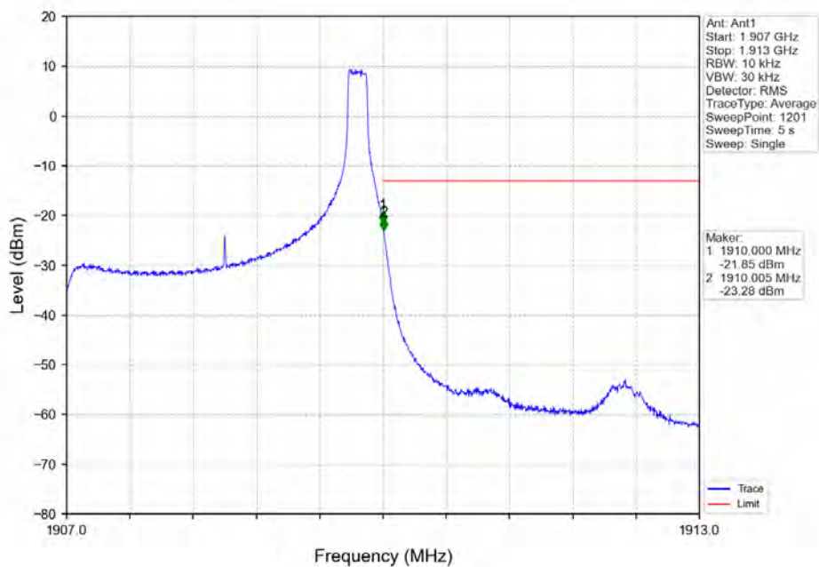
Band2_3MHz_64QAM_HCH_1908.5MHz_RB_1_14_NTNV
