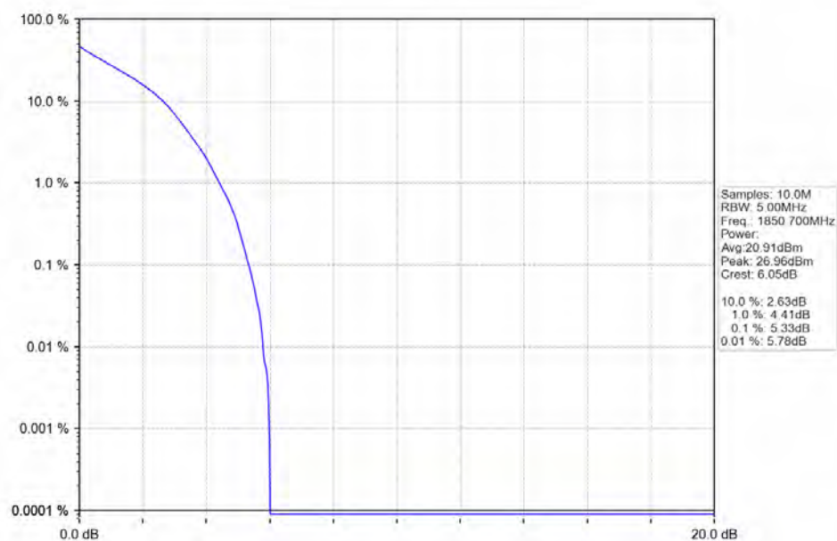
Band2_1.4MHz_QPSK_LCH_1850.7MHz_RB_6_0_NTNV
