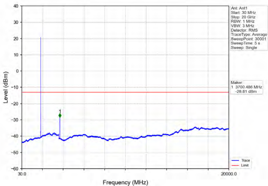
Band2_3MHz_16QAM_LCH_1851.5MHz_RB_15_0_NTNV
