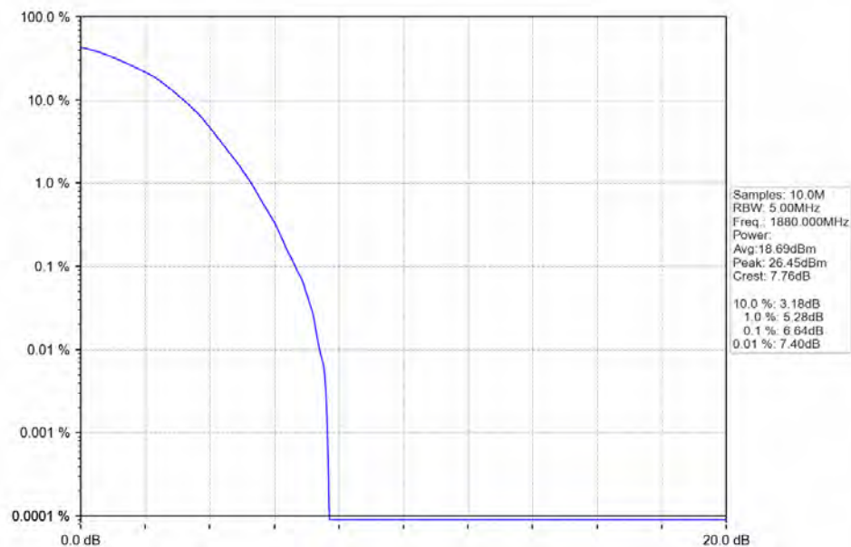
Band2 1.4MHz 64QAM MCH 1880MHz RB 6 0 NTV
