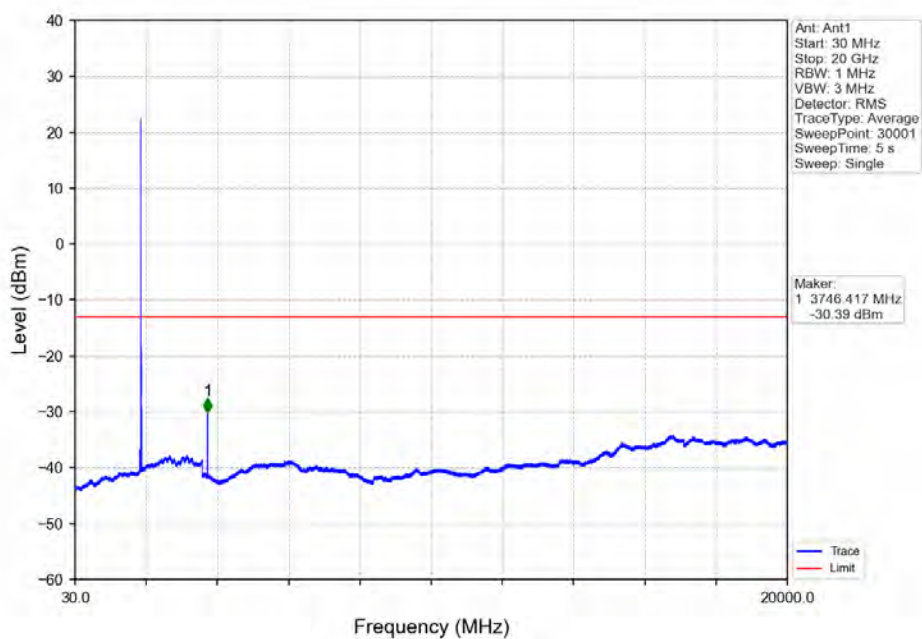
Band2_15MHz_16QAM_HCH_1902.5MHz_RB_1_0_NTNV
