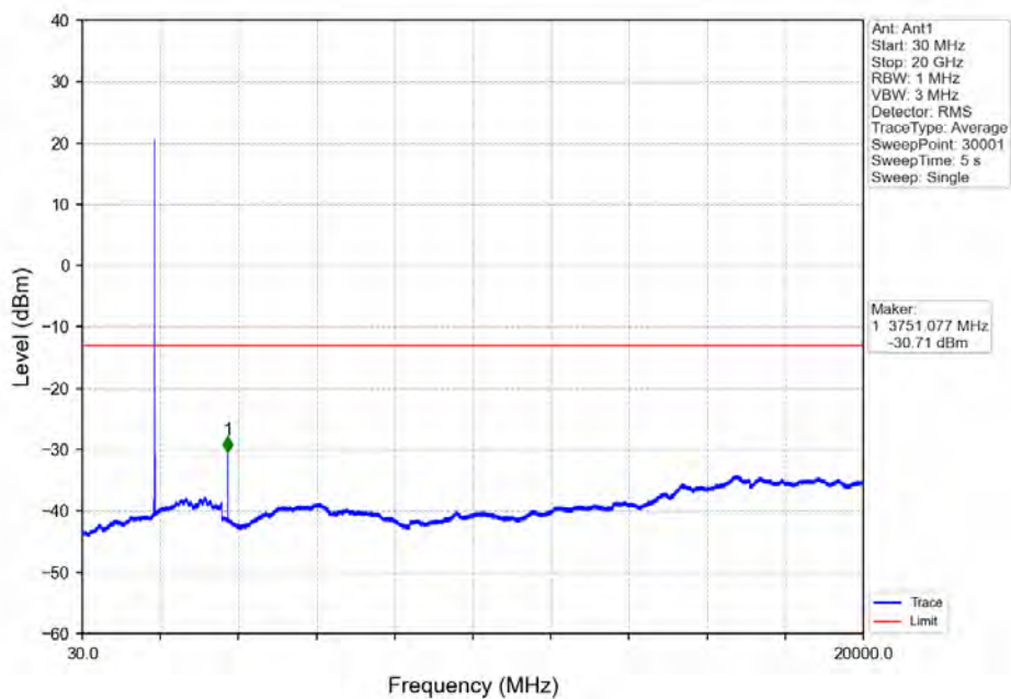
Band2_10MHz_64QAM_MCH_1880MHz_RB_1_0_NTNV
