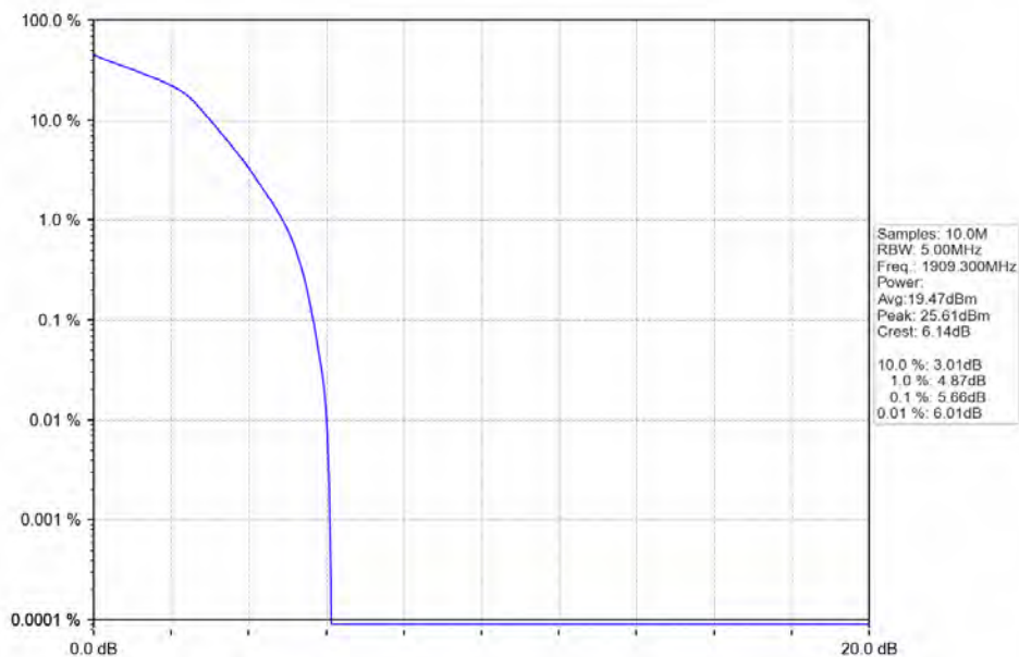
Band2 1.4MHz 16QAM HCH 1909.3MHz RB 6 0 NTN
