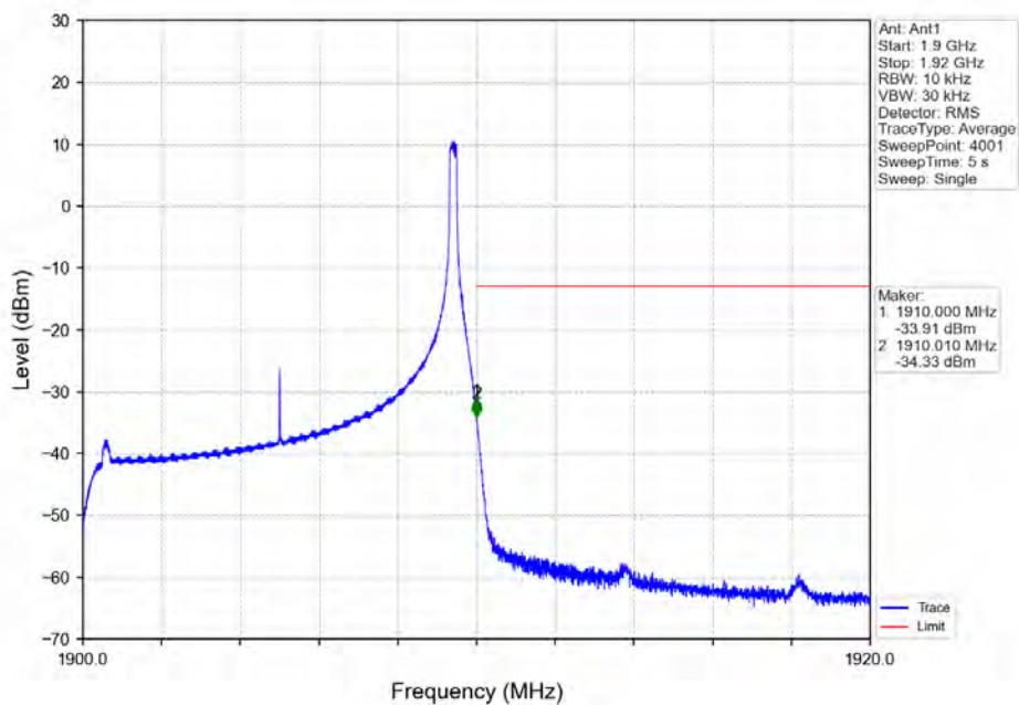
Band2_10MHz_64QAM_HCH_1905MHz_RB_1_49_NTNV
