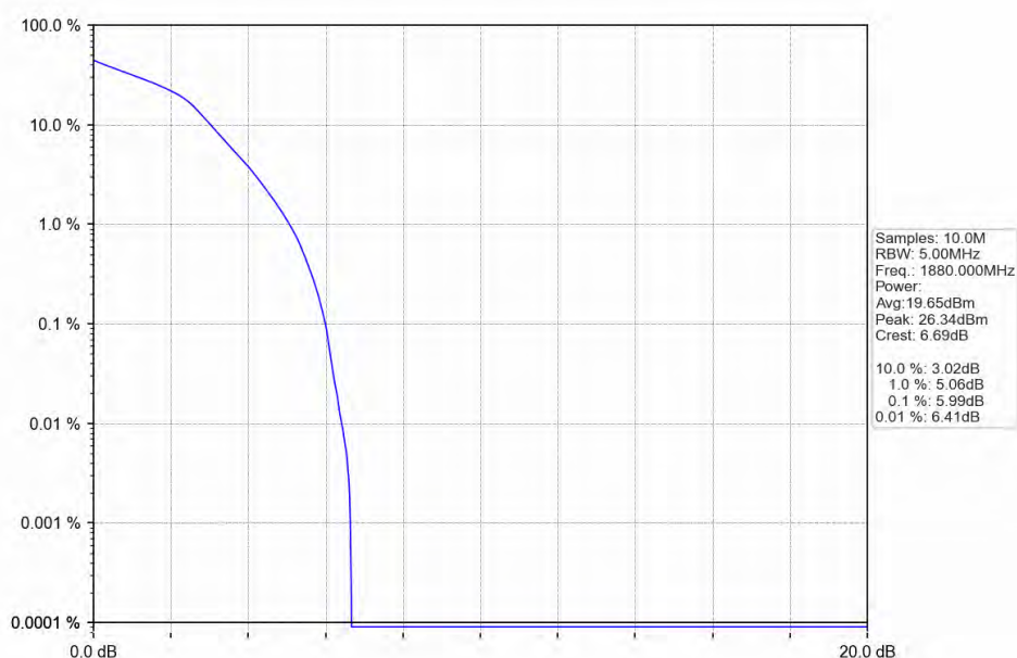
Band2 1.4MHz 16QAM MCH 1880MHz RB 6 0 NTN
