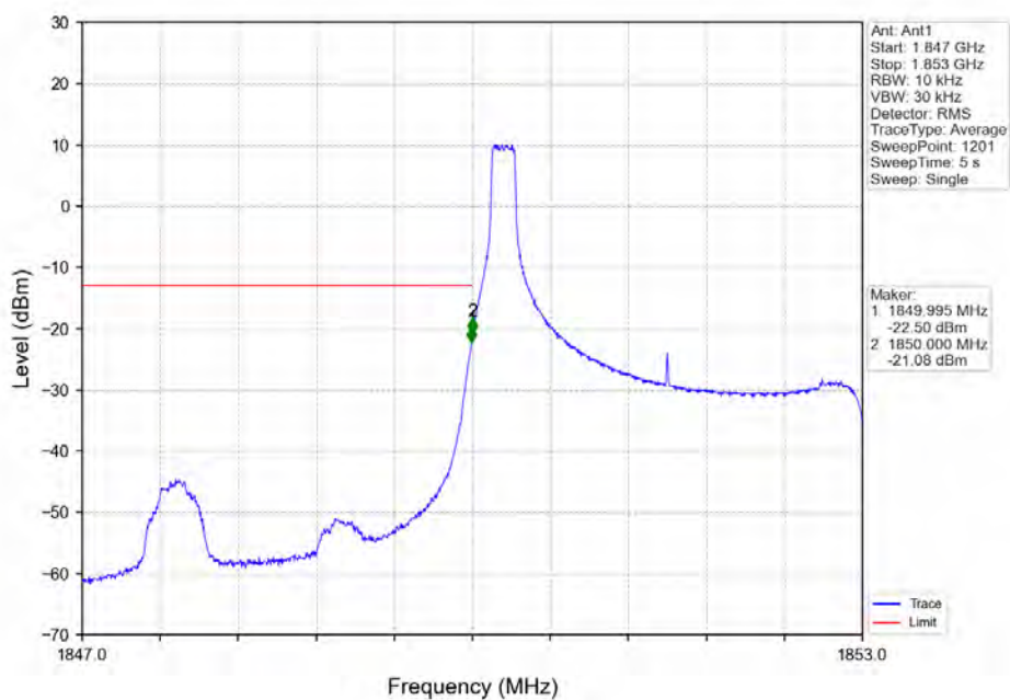
Band2_3MHz_64QAM_LCH_1851.5MHz_RB_1_0_NTNV
