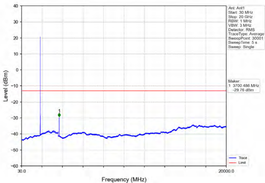
Band2_5MHz_16QAM_LCH_1852.5MHz_RB_25_0_NTNV
