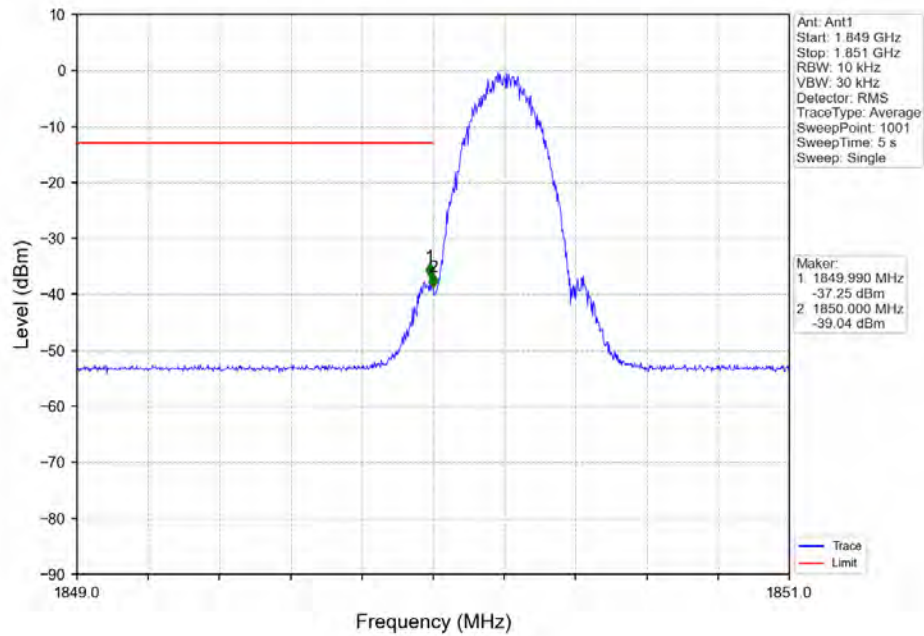
PCS1900_GSM_LCH_1850.2MHz_1 TX Slot_NTNV
