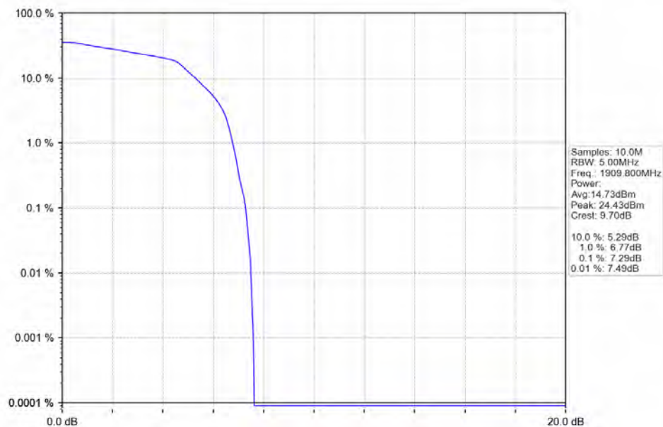
PCS1900_EGSM_HCH_1909.8MHz_4 TX Slots_NTNV
