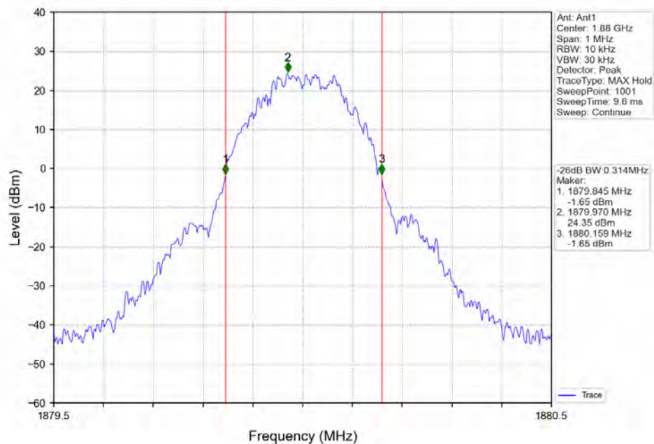
PCS1900_GSM_MCH_1880MHz_1 TX Slot_NTNV
