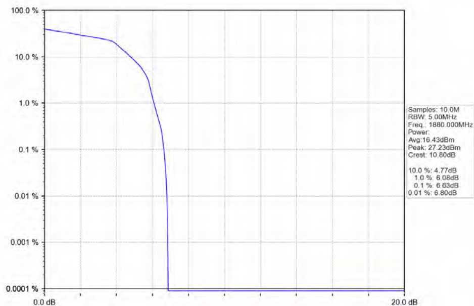
PCS1900_EGSM_MCH_1880MHz_4 TX Slots_NTNV
