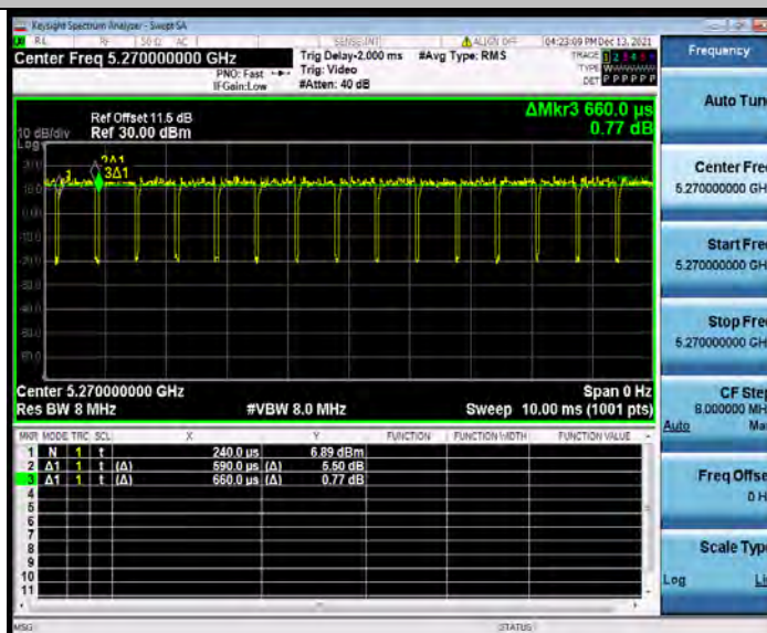
11AC40SISO_Ant1_5270
