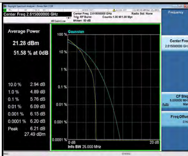
Band38-10MHz-64QAM-38200-50RB#0
