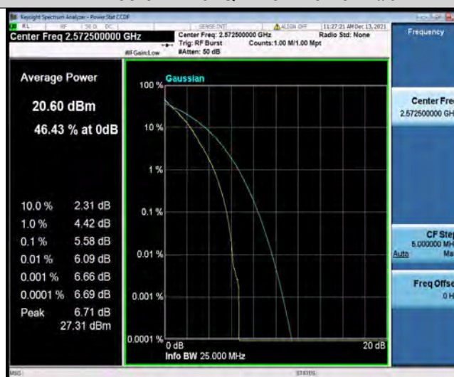
Band38-5MHz-64QAM-38000-1RB#0
