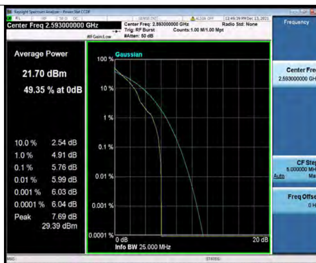
Band41-15MHz-64QAM-40620-75RB#0
