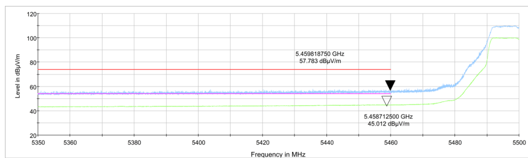
Fig.40 Band Edges (802.11n-HT20 Ch100, 5500MHz)
