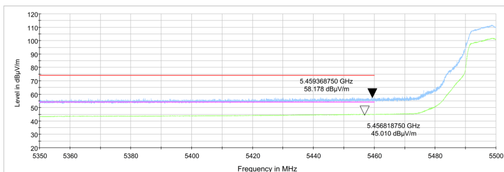
Fig.44 Band Edges (802.11ac-HT20 Ch100, 5500MHz)
