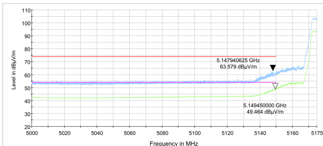
Fig.46 Band Edges (802.11n-HT40 Ch38, 5190MHz)
