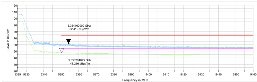
Fig.51 Band Edges (802.11ac-HT40 Ch62, 5310MHz)
