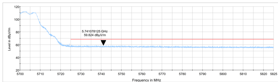
Fig.37 Band Edges (802.11a Ch140, 5700MHz)
