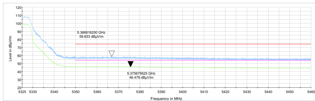
Fig.43 Band Edges (802.11ac-HT20 Ch64, 5320MHz)
