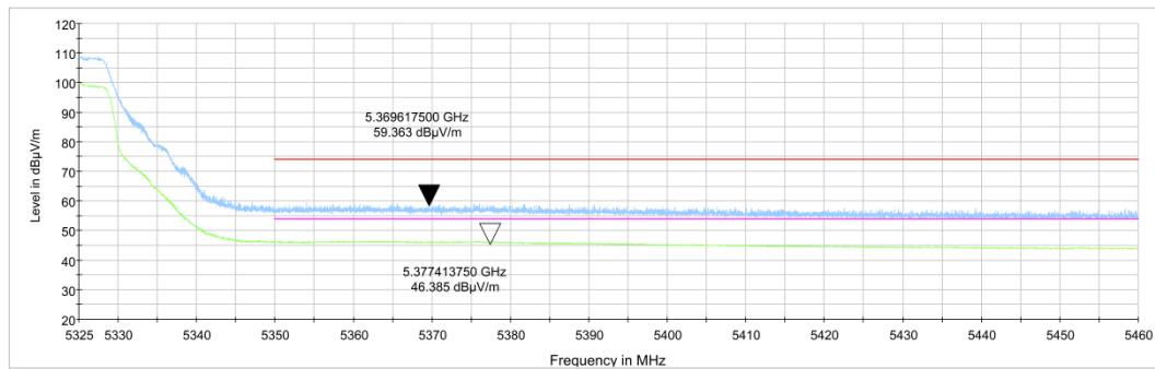
Fig.39 Band Edges (802.11n-HT20 Ch64, 5320MHz)
