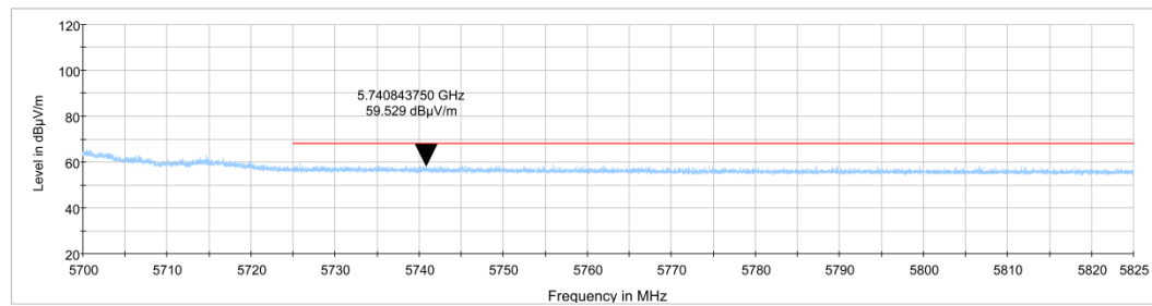
Fig.49 Band Edges (802.11n-HT40 Ch134, 5670MHz)
