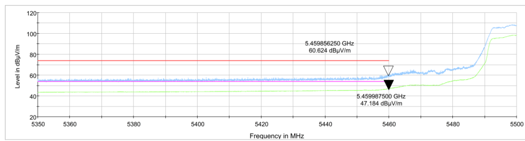
Fig.48 Band Edges (802.11n-HT40 Ch102, 5510MHz)
