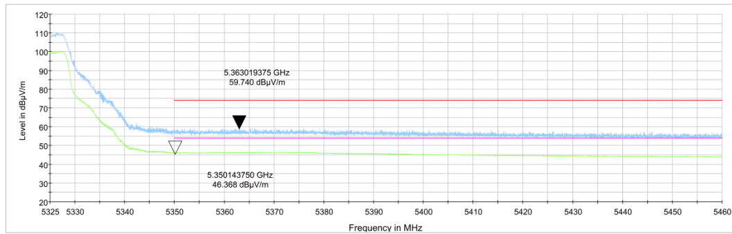
Fig.35 Band Edges (802.11a Ch64, 5320MHz)
