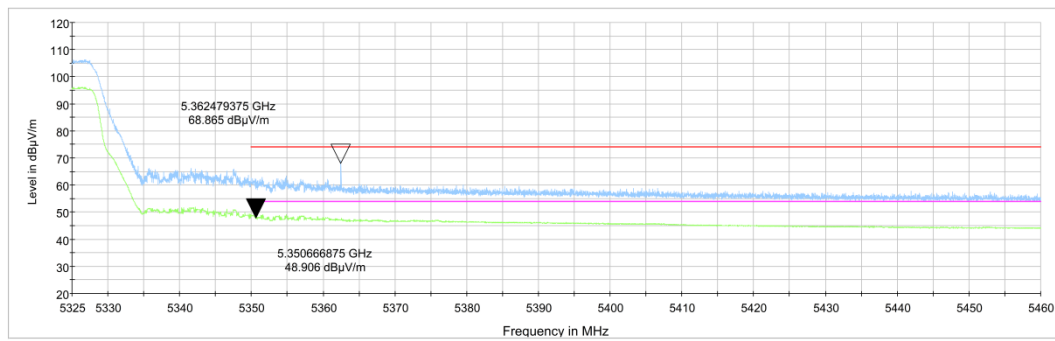
Fig.47 Band Edges (802.11n-HT40 Ch62, 5310MHz)
