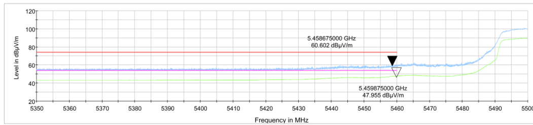
Fig.56 Band Edges (802.11ac-HT80 Ch106, 5530MHz)
