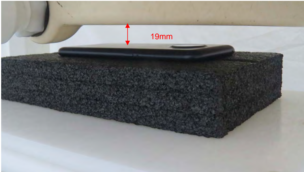
Picture 19: Back Side, the distance from handset to the bottom of the Phantom is 19mm
