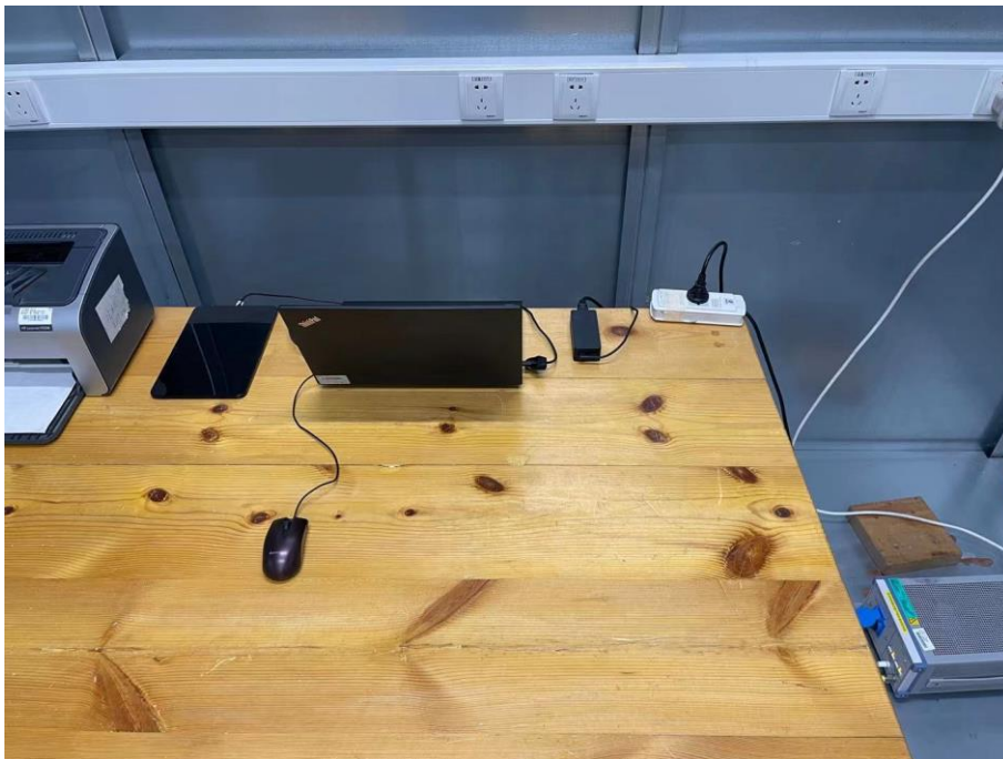
22. Conducted Emission (Part 15B, Data Transfer)
