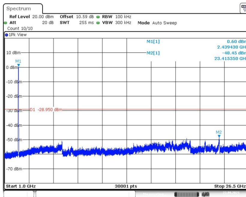
Fig.62 Conducted Spurious Emission (1GHz-26.5GHz, 802.11n-HT40, CH3)
