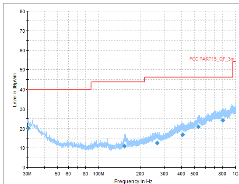
Fig.90 Radiated Spurious Emission (All Channels, 30MHz-1 GHz)
