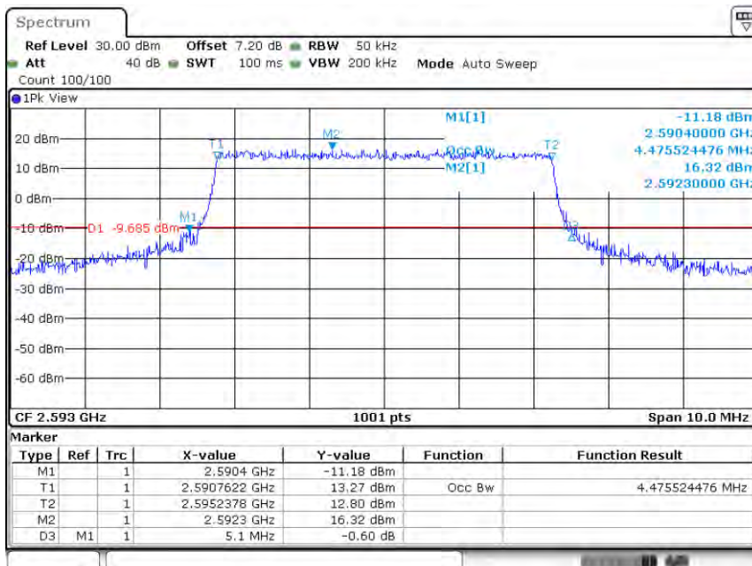
Band41-5MHz-QPSK-40620-25RB#0-4.476
