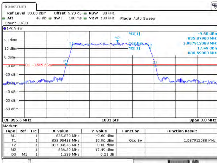
Band5-1.4MHz-QPSK-20525-6RB#0-1.088
