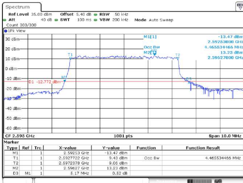
Band38-5MHz-QPSK-38000-25RB#0-4.466
