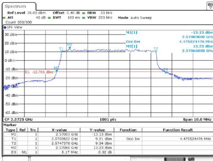
Band38-5MHz-QPSK-37775-25RB#0-4.476
