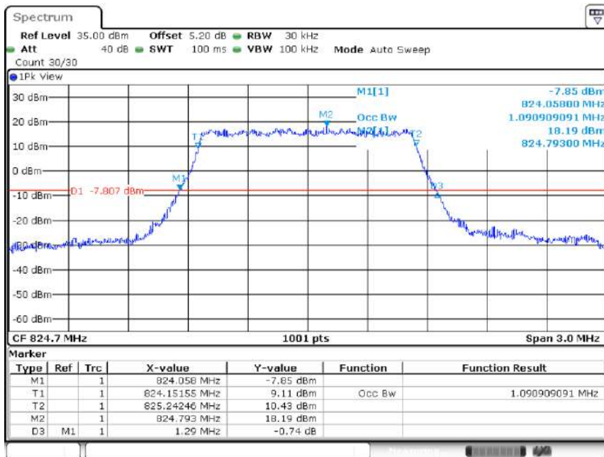
Band5-1.4MHz-OPSK-20407-6RB#0-1.091
