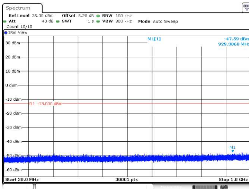
Band4-20MHz-QPSK-20175-1RB#0-Range1:30~1000MHz
