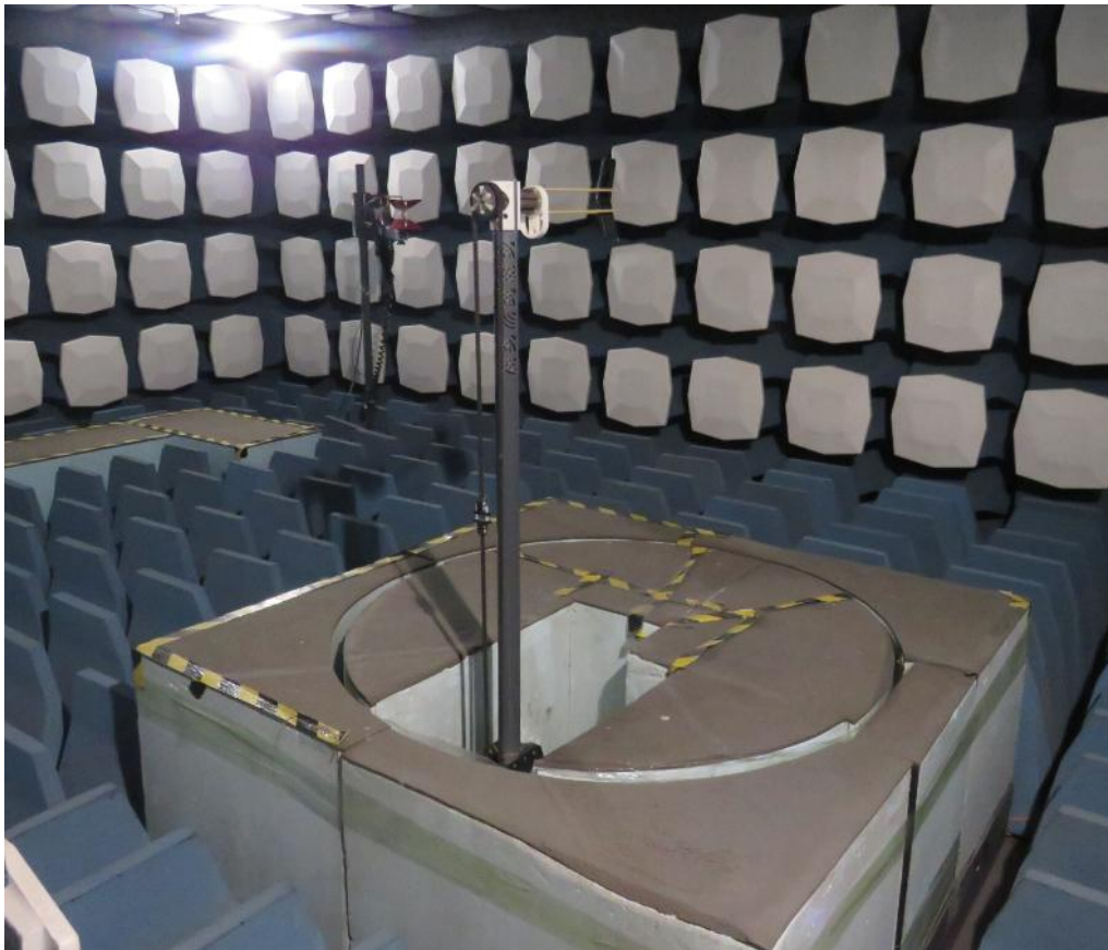
Radiated Spurious Emission and Output Power
