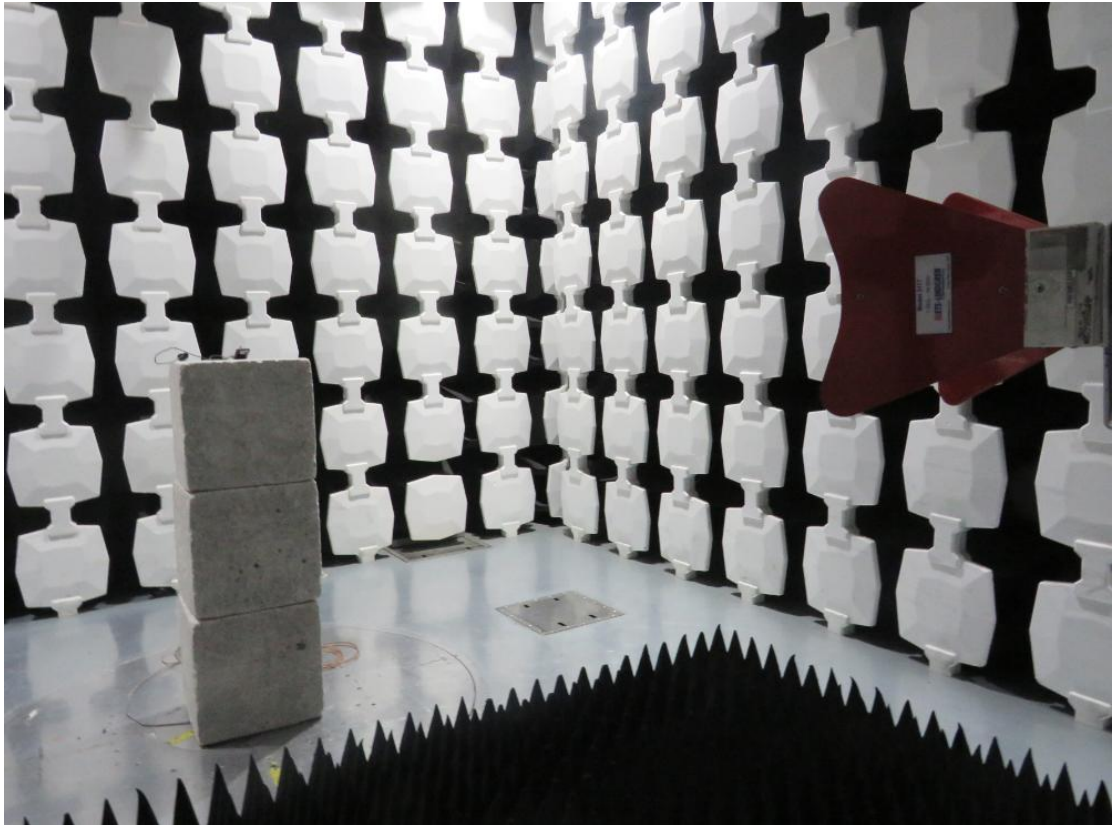
Radiated Spurious Emission and Output Power
