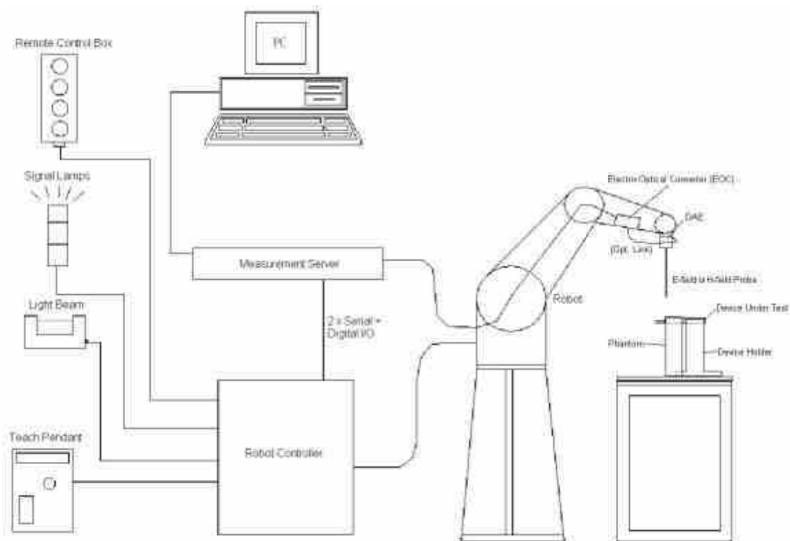
Fig 5.1 System Configurations
