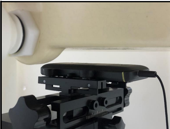
Rear Face of EUT with 1.5 cm Gap ( Earphone )
