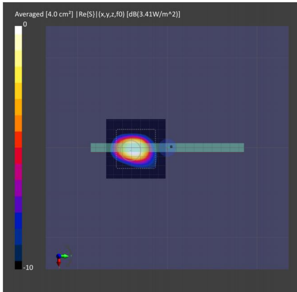
Figure 8-2: 4cm2-averaged power density distribution measured at input.power.limit of 3.03 dBm on the Back for n260 beam 38
