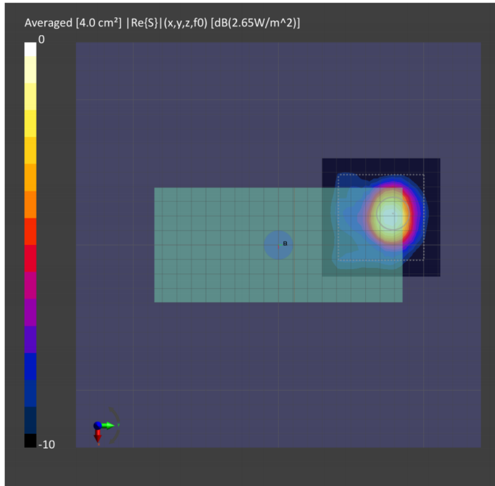
Figure 8-3: 4cm2-averaged power density distribution measured at input.power.limit of 2.27dBm on the back surface for n261 beam 29
