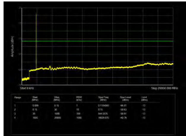
LTE Band 2 10MHz CH-Low 9kHz~20GHz
