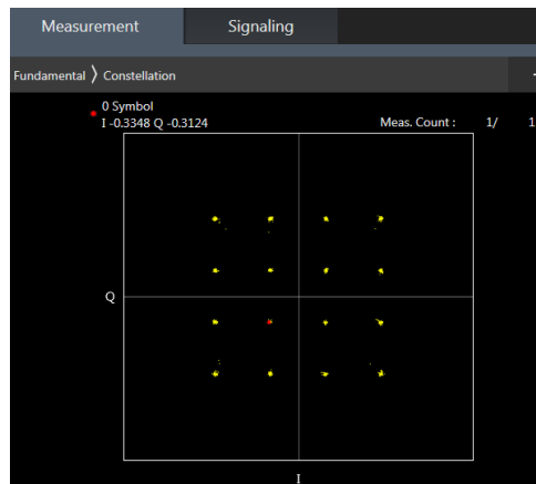
16QAM
