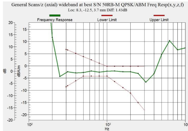
Figure C.13 Frequency Response of W850 - OTT VoIP
