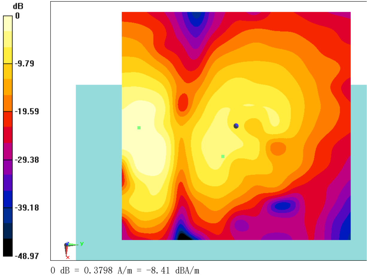
Fig B.21 T-Coil WiFi-2.4G
