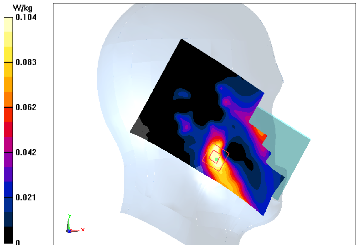
Fig.11 LTE Band 41
