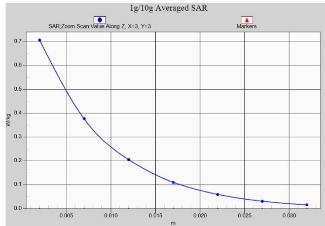
Fig. 10-1 Z-Scan at power reference point (LTE Band7)
