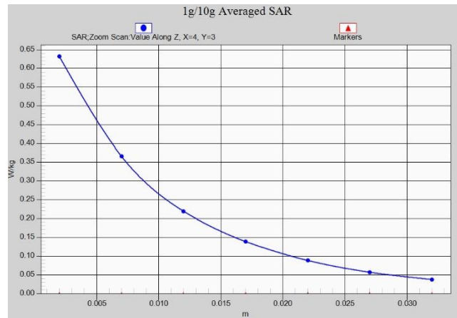
Fig. 8-1 Z-Scan at power reference point (LTE Band5)
