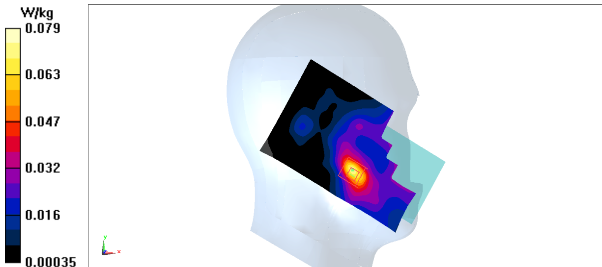
Fig.3 1900 MHz
