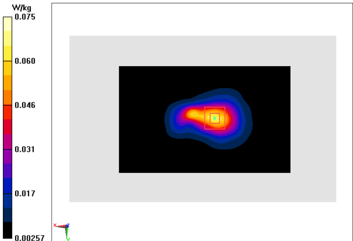
Fig.14 2450 MHz
