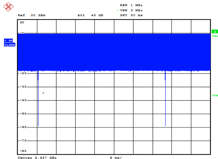
Picture 14.1 Duty factor plot for head
