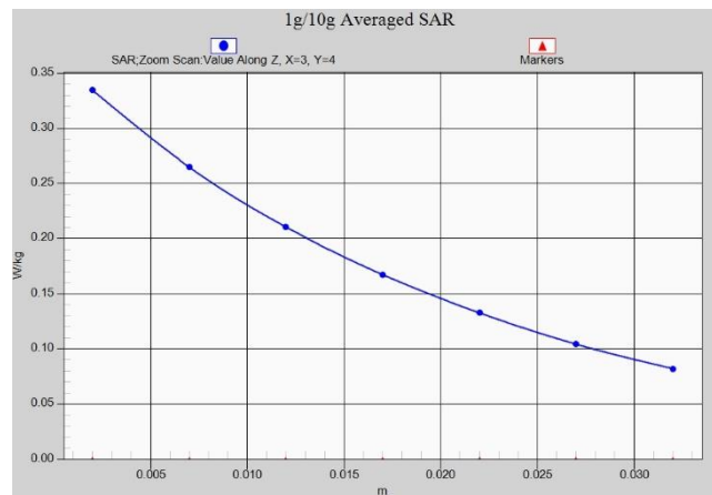
Fig. 7-1 Z-Scan at power reference point (LTE Band5)
