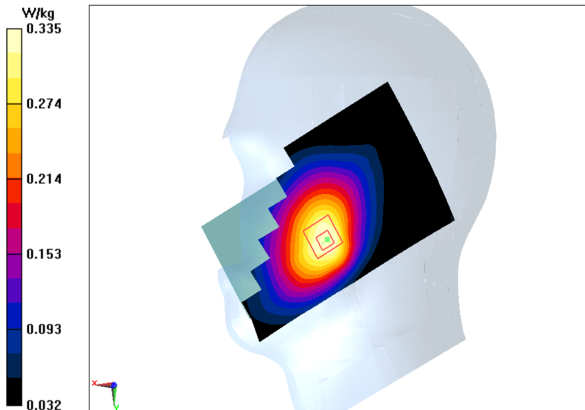
Fig.7 LTE Band5
