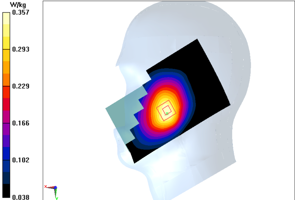
Fig.1 850MHz
