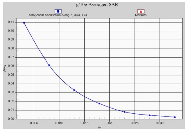
Fig. 9-1 Z-Scan at power reference point (LTE Band7)
