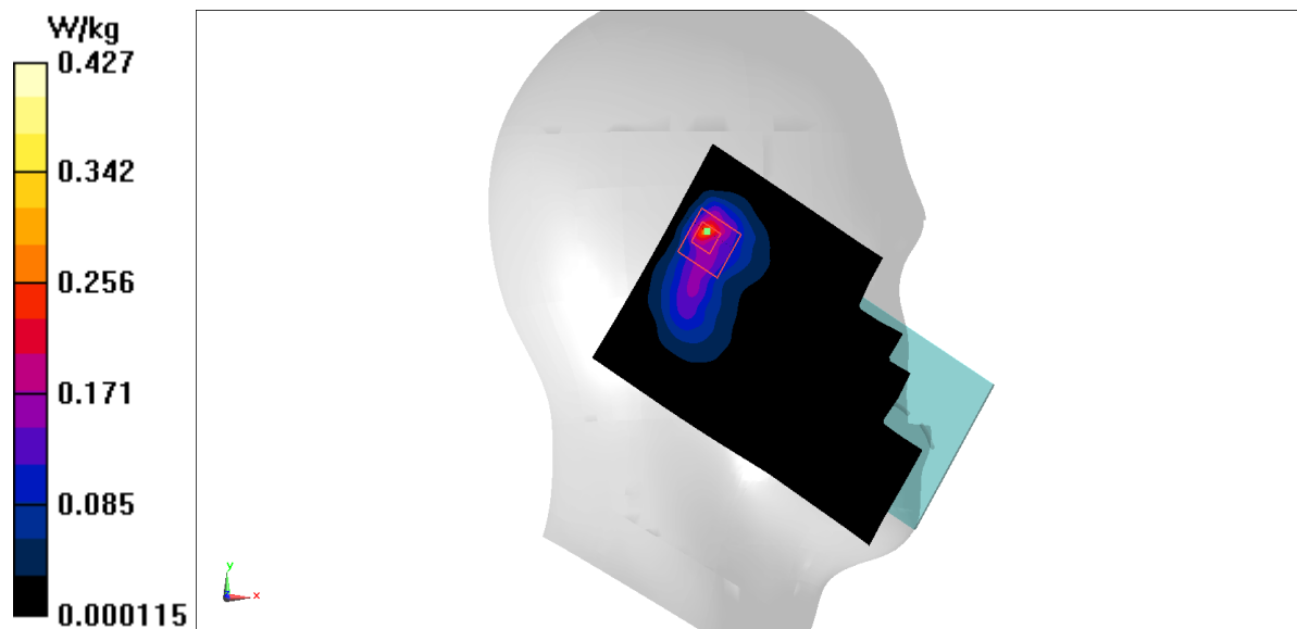
Fig.13 2450 MHz
