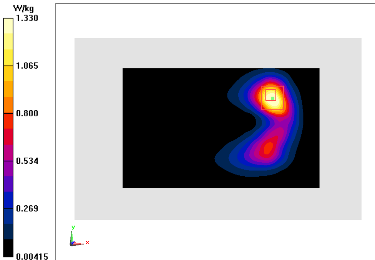
Fig.12 LTE Band 41
