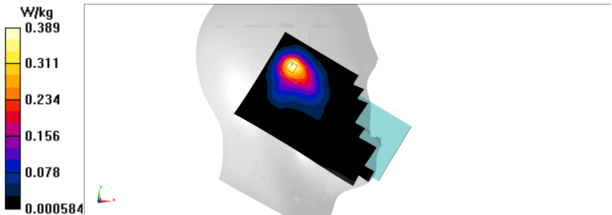
Fig.13 2450 MHz
