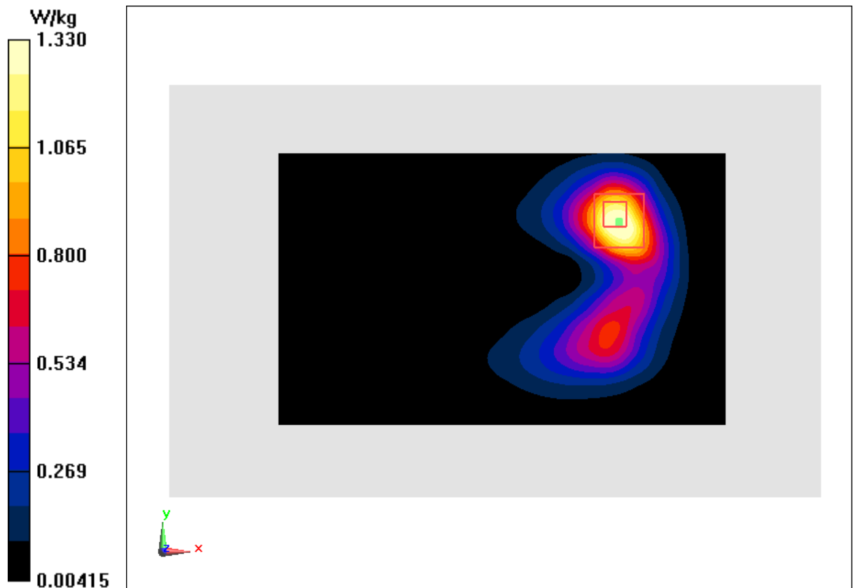
Fig.12 LTE Band 41
