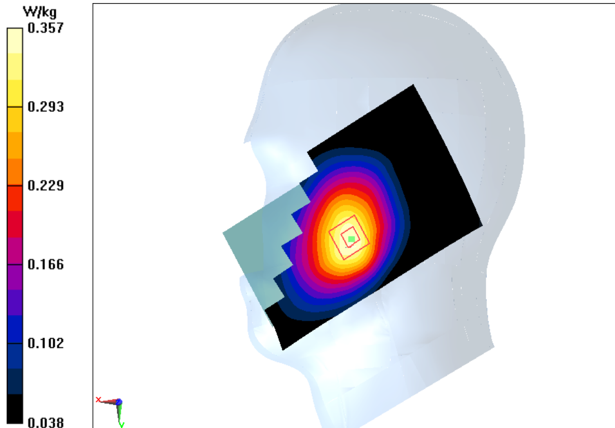
Fig.1 850MHz
