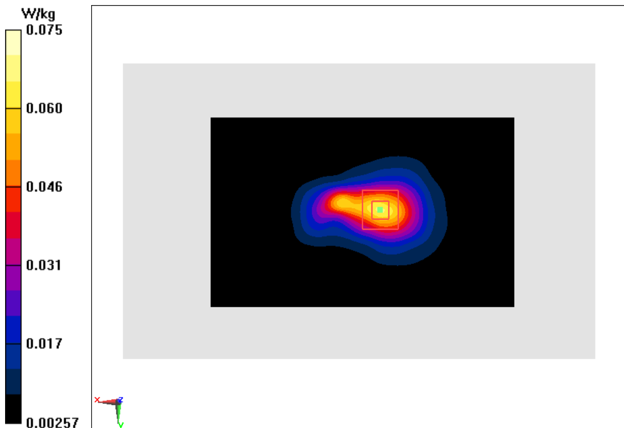
Fig.14 2450 MHz
