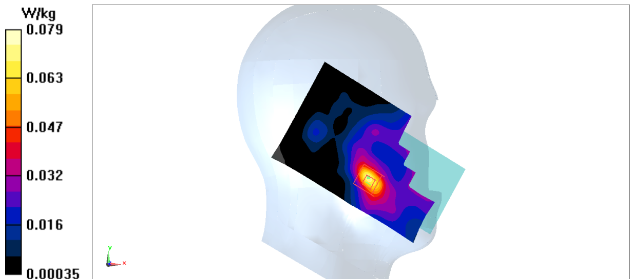
Fig.3 1900 MHz
