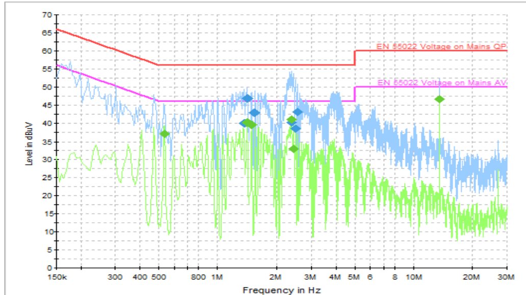
Figure A-5: Test result of EUT1 at test set. NFC01
