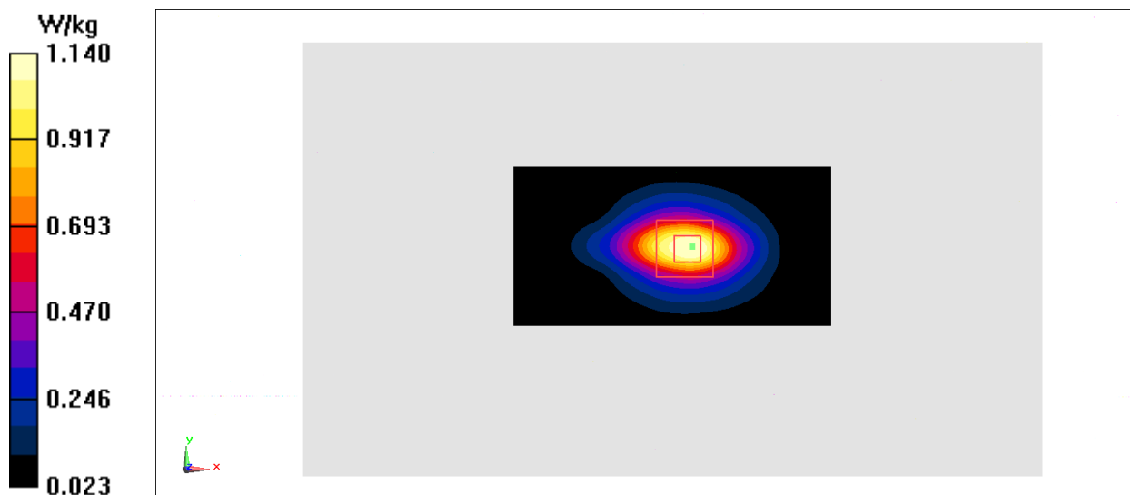
Fig.22 LTE Band66
