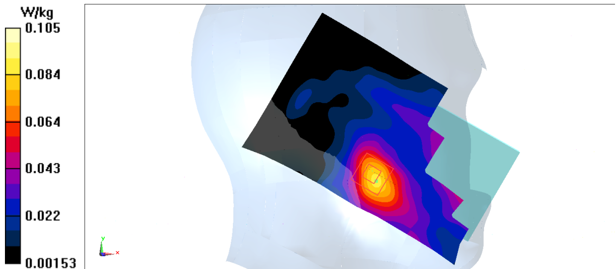
Fig.21 LTE Band66
