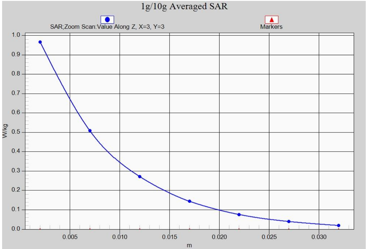
Fig. 20-1 Z-Scan at power reference point (LTE Band 38)
