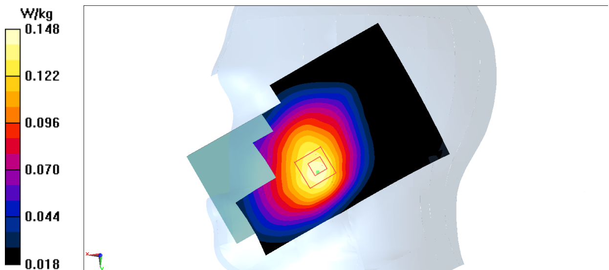
Fig.17 LTE Band12
