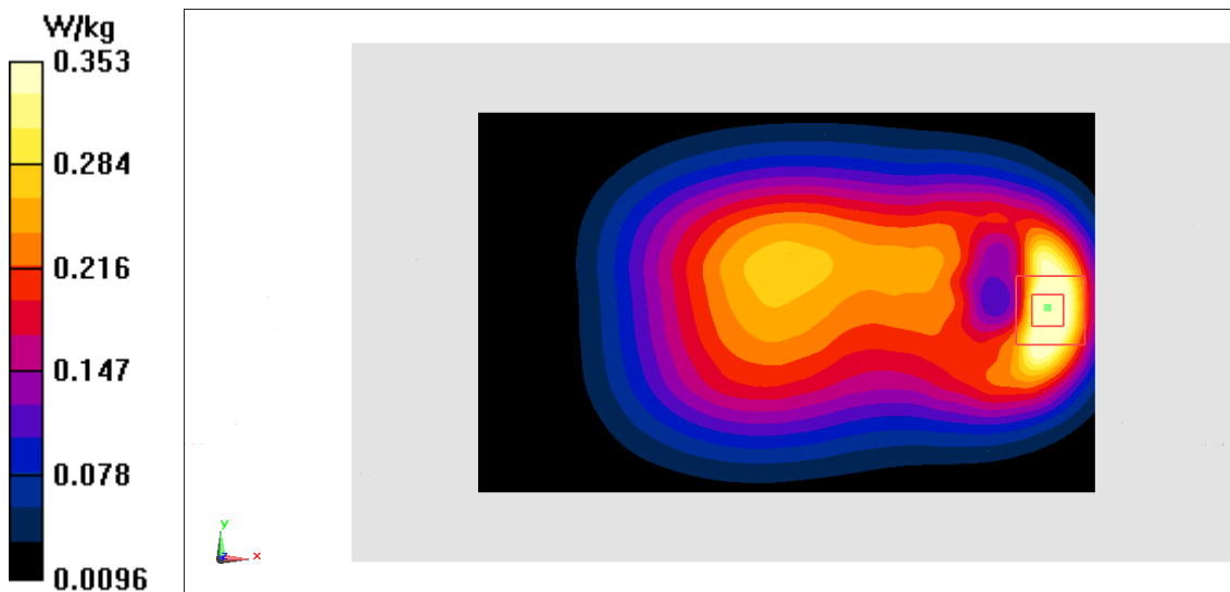
Fig.2 850 MHz
