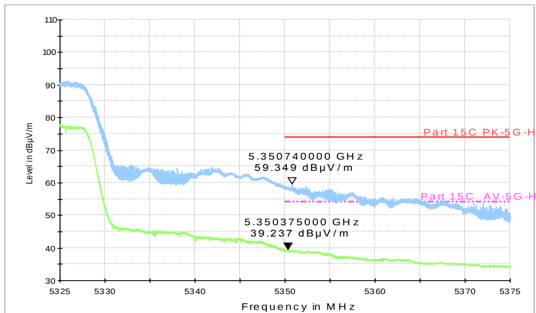
Fig. 35 Band Edges (802.11n-HT40, 5310MHz)
