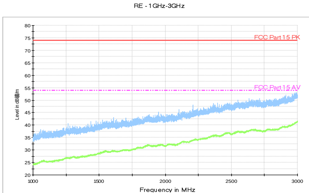
Fig. 99 Radiated Spurious Emission (802.11n-HT20, ch116, 1 GHz-3 GHz)
