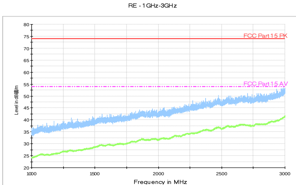
Fig. 47 Radiated Spurious Emission (802.11a, ch52, 1 GHz-3 GHz)
