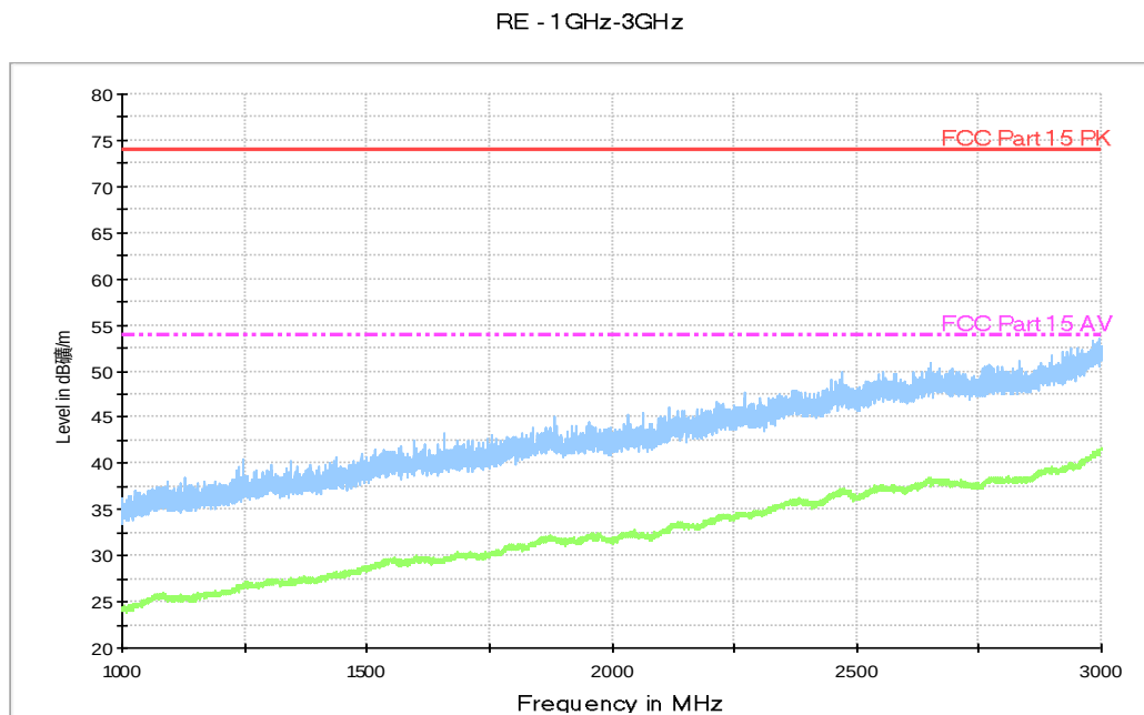
Fig. 51 Radiated Spurious Emission (802.11a, ch56, 1 GHz-3 GHz)
