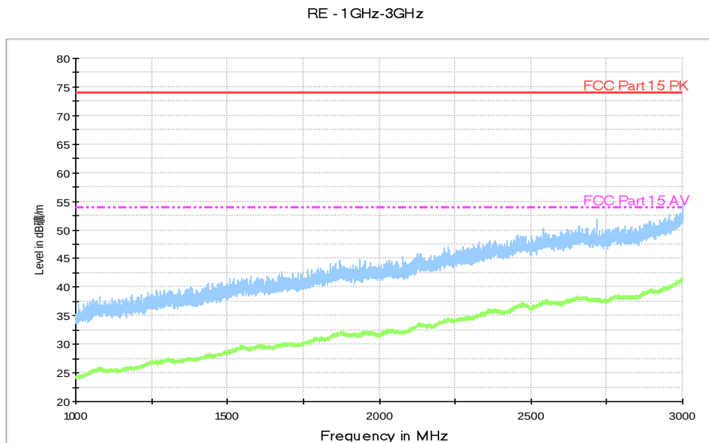
Fig. 117 Radiated Spurious Emission (802.11n-HT40, ch54, 1 GHz-3 GHz)
