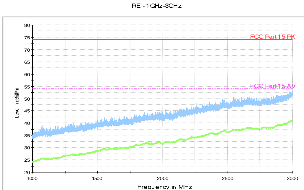
Fig. 39 Radiated Spurious Emission (802.11a, ch40, 1 GHz-3 GHz)
