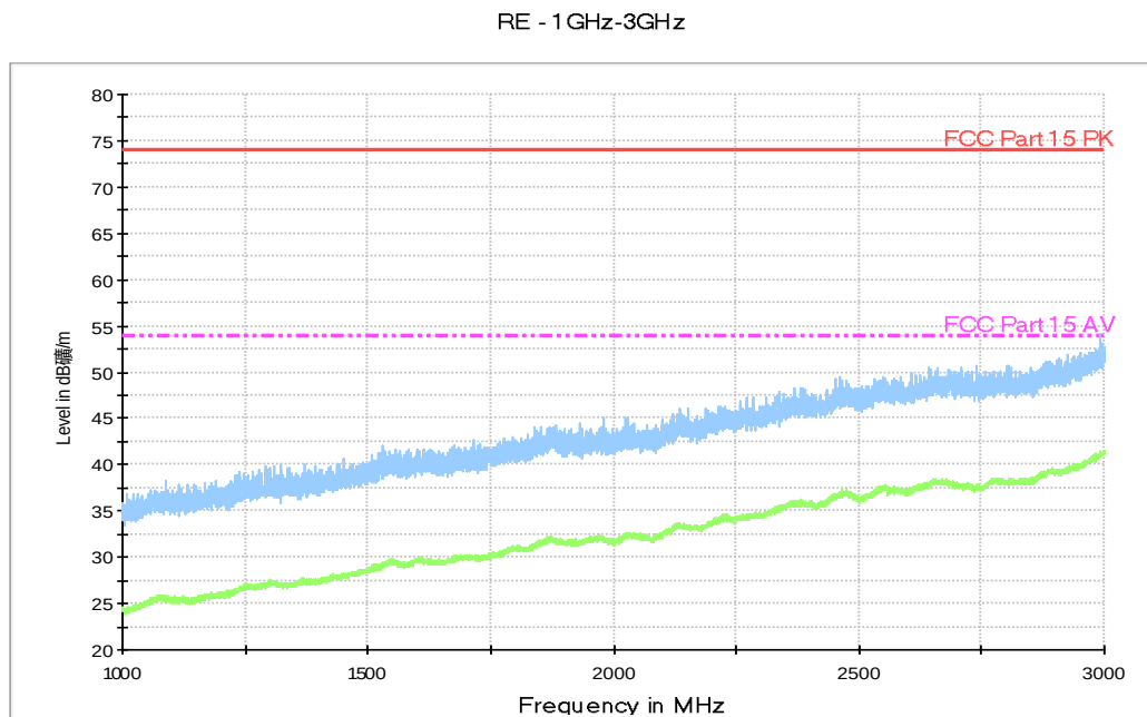
Fig. 71 Radiated Spurious Emission (802.11n-HT20, ch36, 1 GHz-3 GHz)
