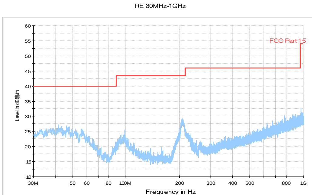
Fig. 107 Radiated Spurious Emission (802.11n-HT40, ch38, 30 MHz-1 GHz)
