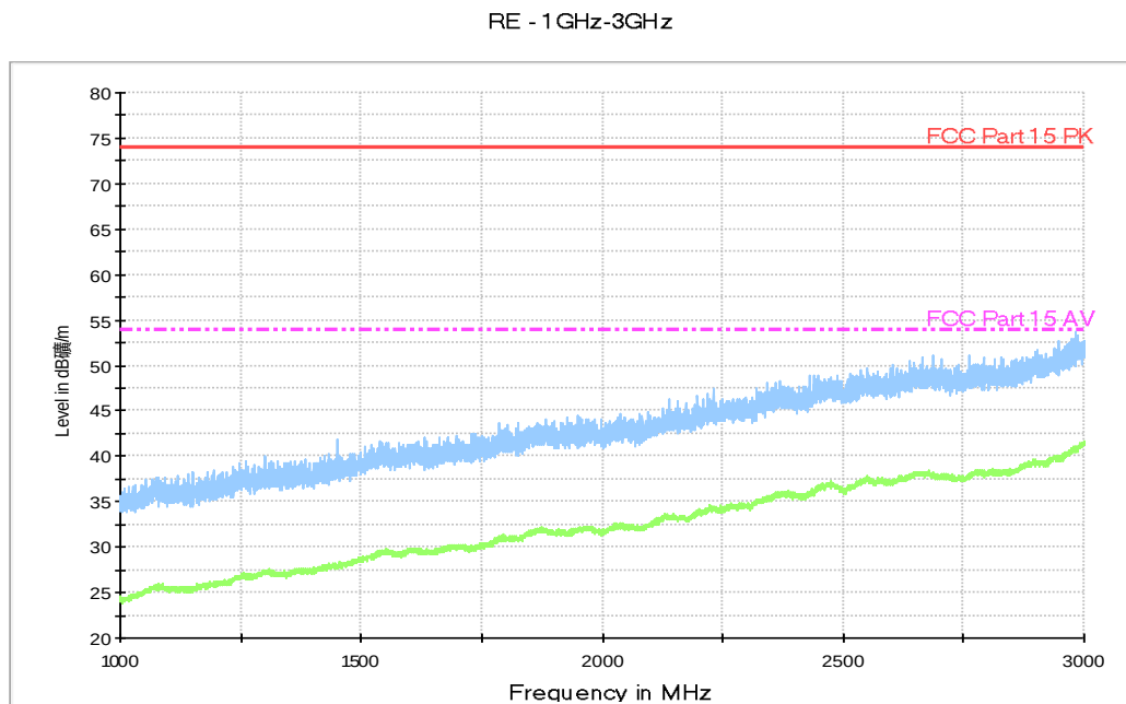
Fig. 87 Radiated Spurious Emission (802.11n-HT20, ch56, 1 GHz-3 GHz)
