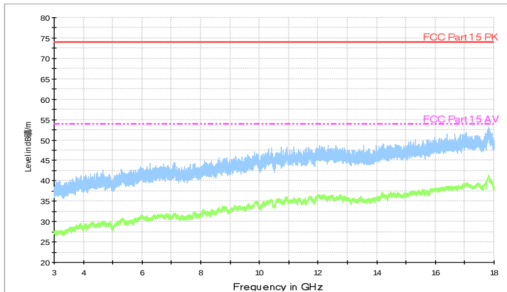
Fig.62. Radiated emission: GFSK, Channel 39, 3 GHz - 18 GHz
