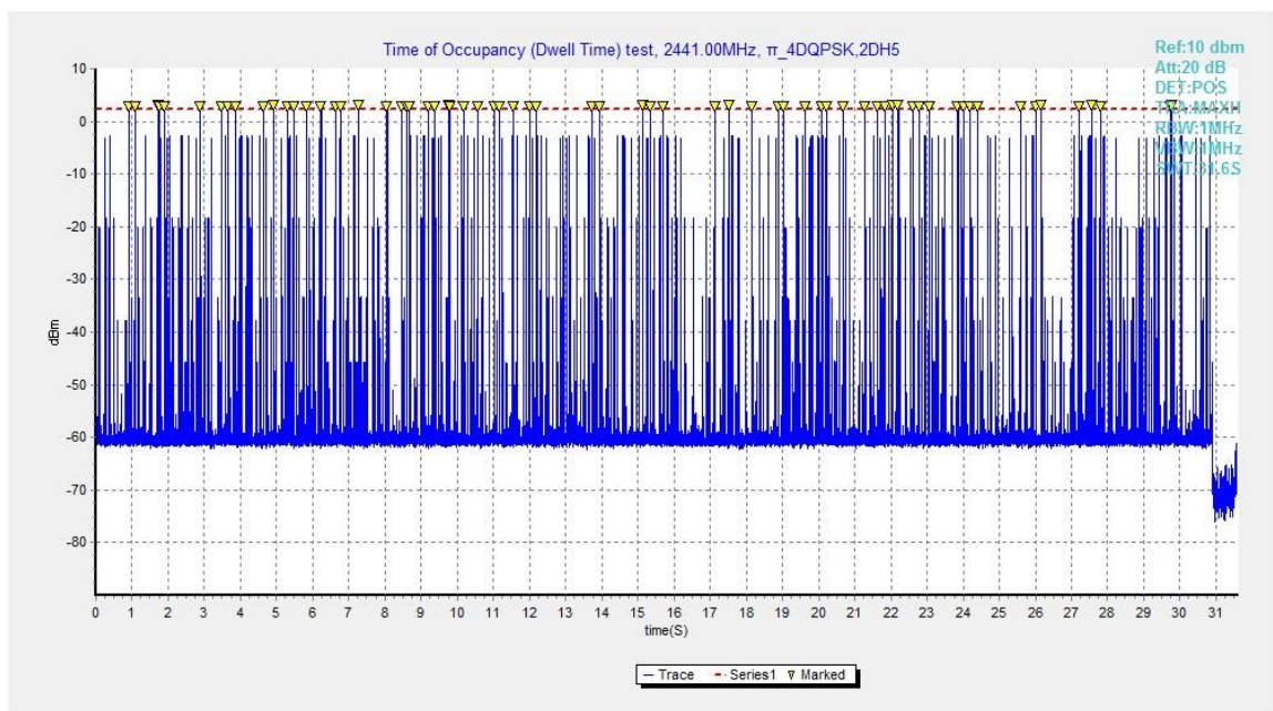
Fig.99. Number of Transmissions Measurement:Channel 39,Packet 2-DH5
