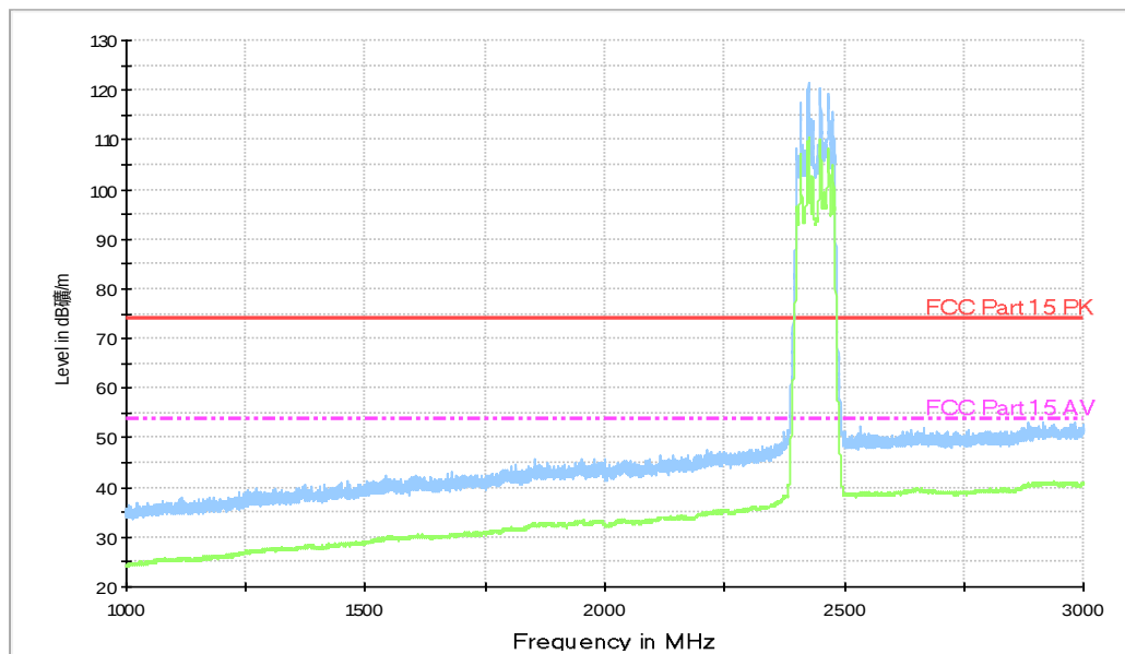
Fig.73. Radiated emission: \pi/4 DQPSK, Channel 78, 1 GHz - 3 GHz
