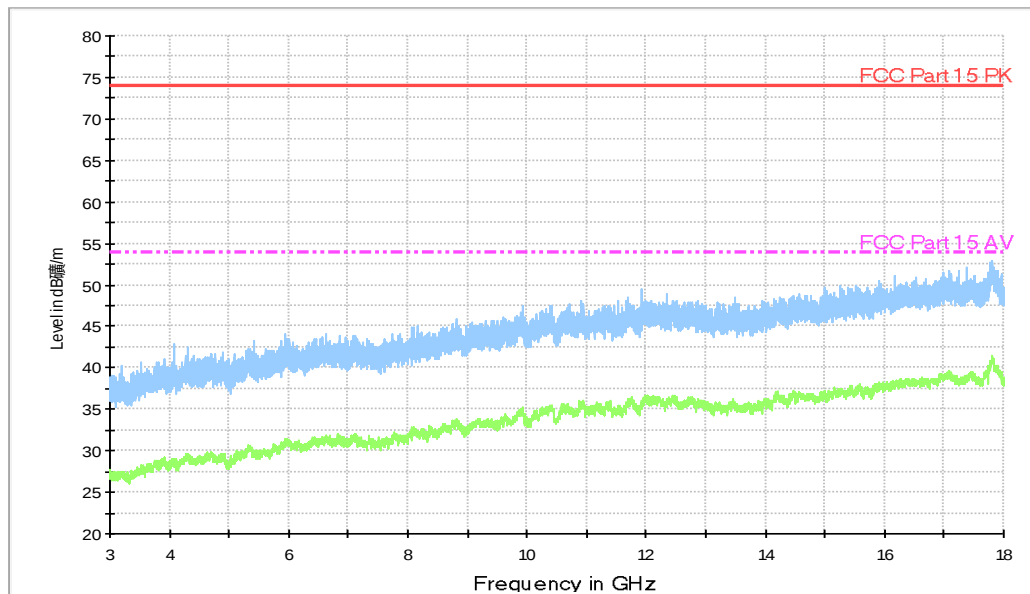
Fig.74. Radiated emission: \pi/4 DQPSK, Channel 78, 3 GHz - 18 GHz
