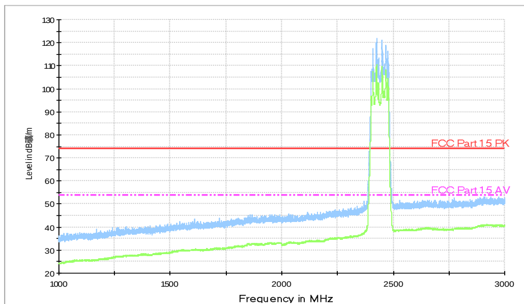
Fig.63. Radiated emission: GFSK, Channel 78, 1 GHz - 3 GHz
