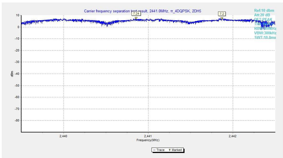
Fig.116. Carrier frequency separation measurement: \pi/4 DQPSK, Channel 39
