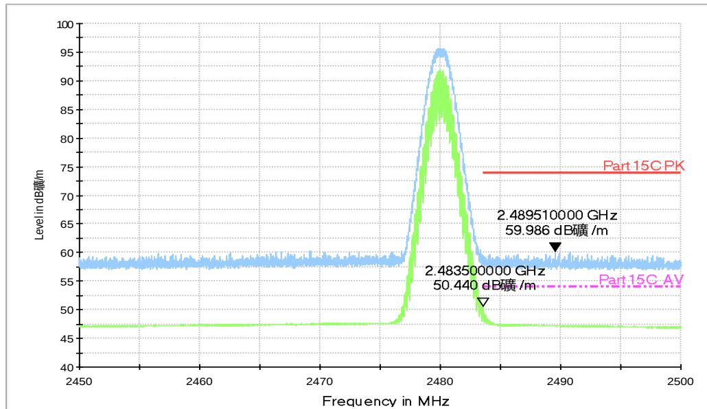
Fig.76. Radiated emission (Power): \pi/4 DQPSK, high channel
