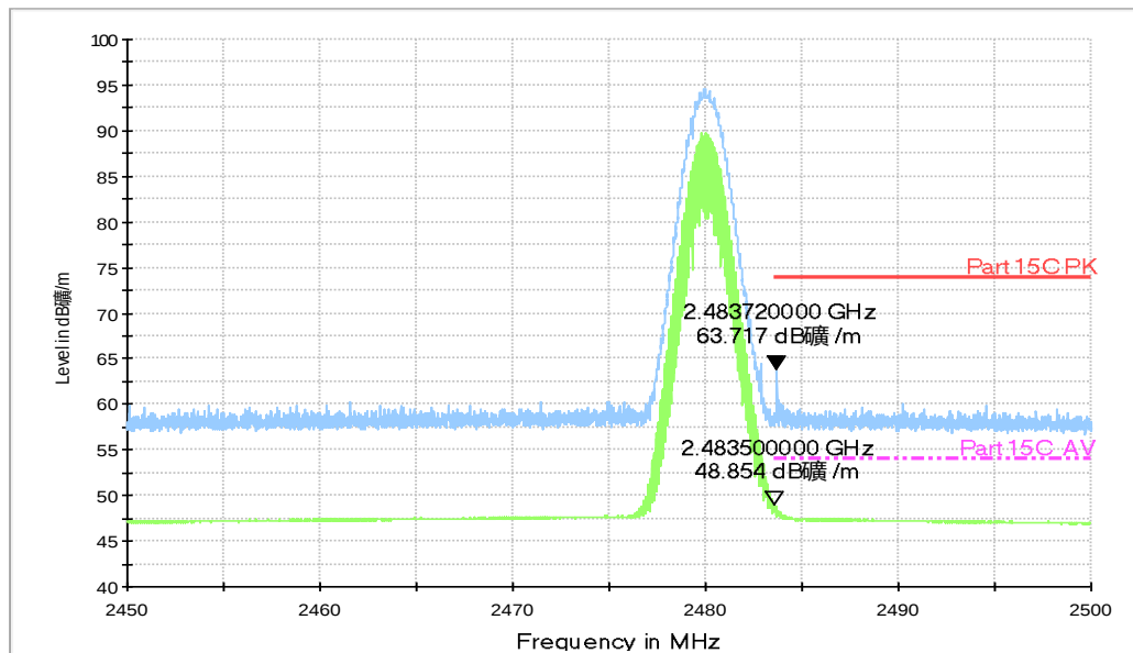
Fig.86. Radiated emission (Power): 8DPSK, high channel
