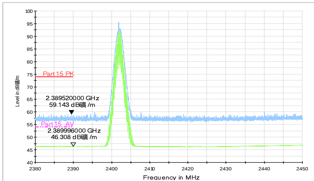
Fig.65. Radiated emission (Power): GFSK, low channel
