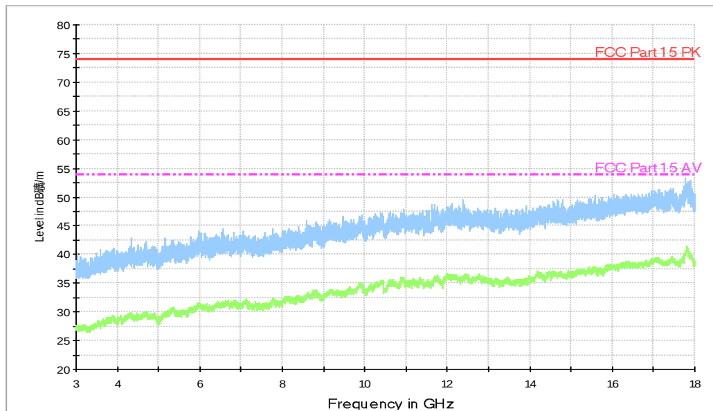
Fig.64. Radiated emission: GFSK, Channel 78, 3 GHz - 18 GHz
