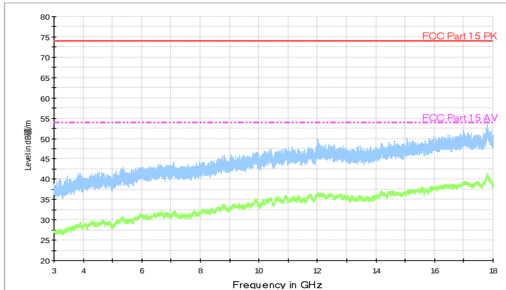
Fig.72. Radiated emission: \pi/4 DQPSK, Channel 39, 3 GHz - 18 GHz
