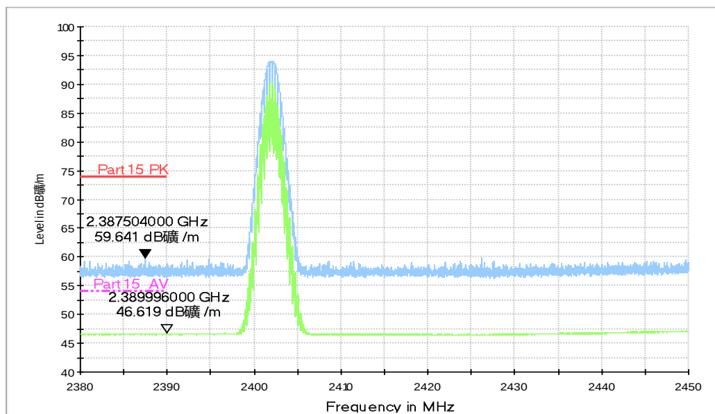
Fig.75. Radiated emission (Power): \pi/4 DQPSK, low channel
