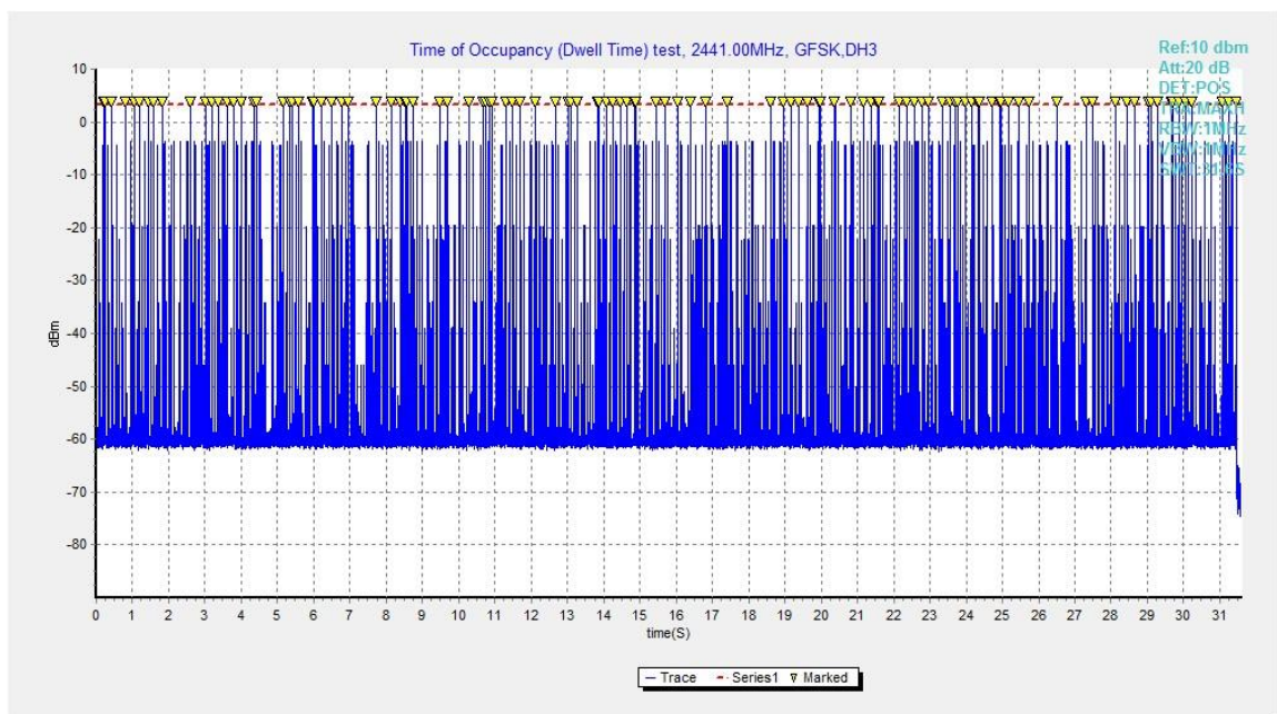
Fig.91. Number of Transmissions Measurement:Channel 39,Packet DH3
