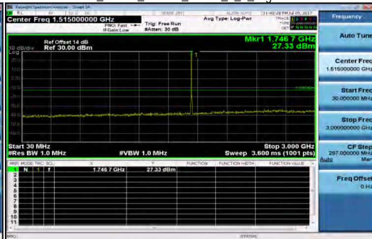
30MHz~3GHz_Band4_10MHz_QPSK_1_0_HighCH20350-1750
