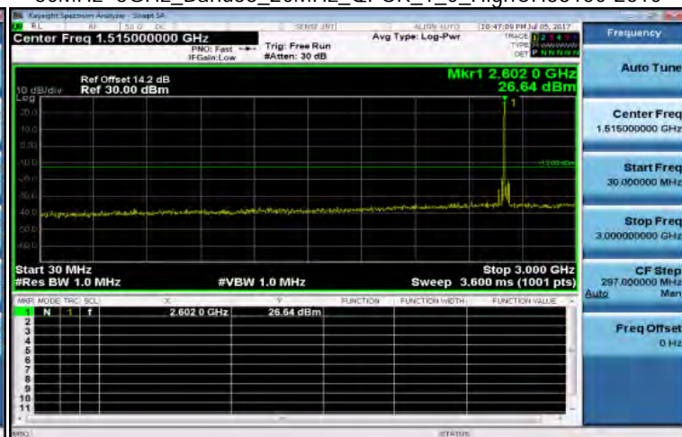
30MHz~3GHz_Band38_20MHz_QPSK_1_0_HighCH38150-2610
