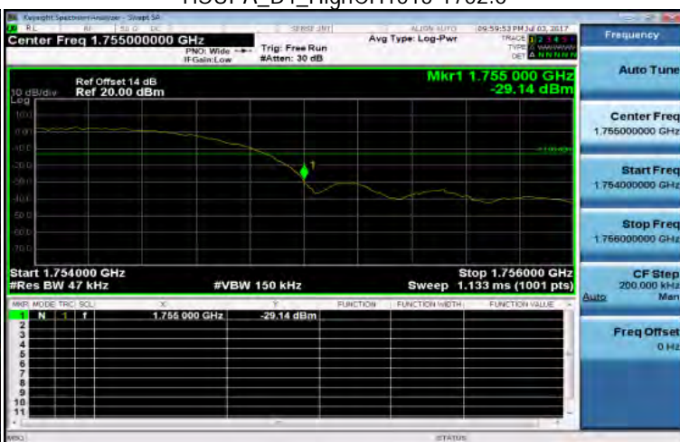
HSUPA_B4_HighCH1513-1752.6
