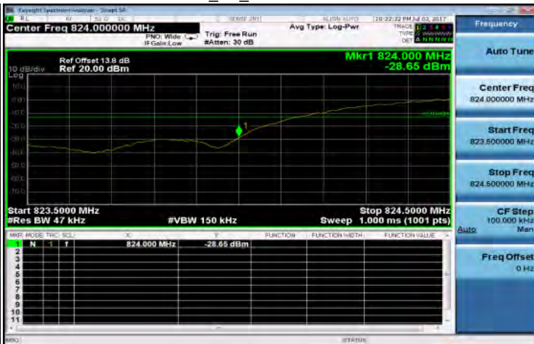
HSUPA_B5_LowCH4132-826.4
