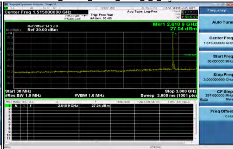
30MHz~3GHz_Band38_10MHz_QPSK_1_0_HighCH38200-2615
