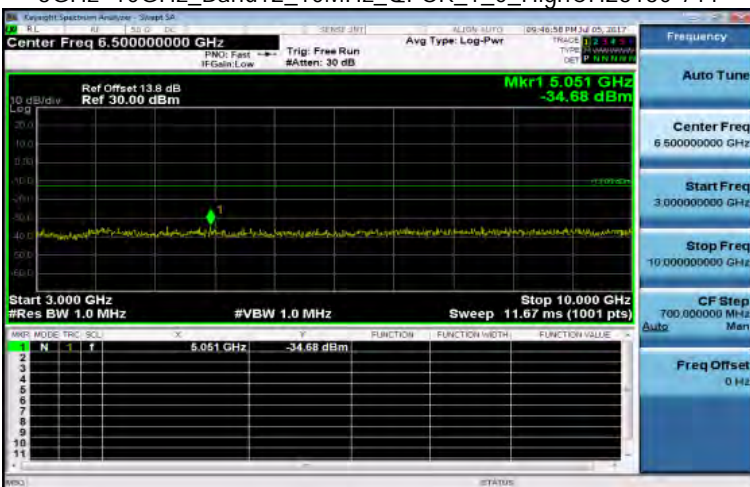
3GHz~10GHz_Band12_10MHz_QPSK_1_0_HighCH23130-711
