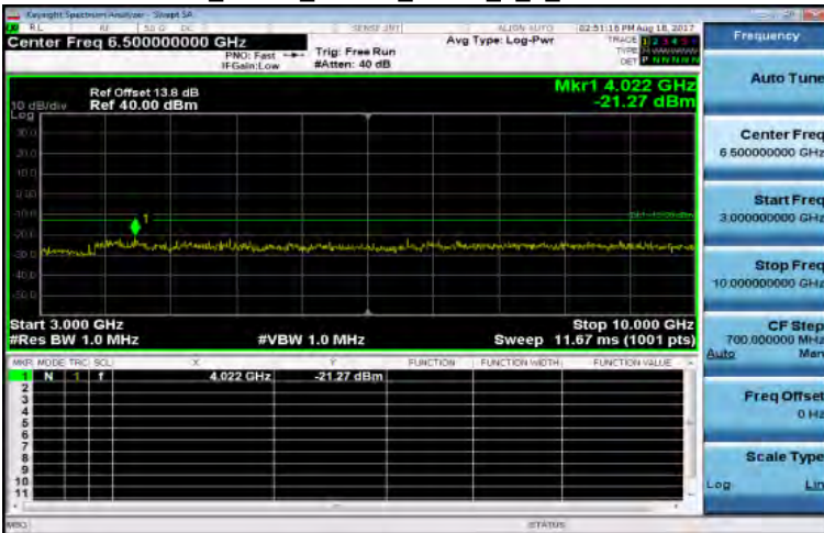
3GHz~10GHz_Band5_10MHz_QPSK_1_0_MidCH20525-836.5
