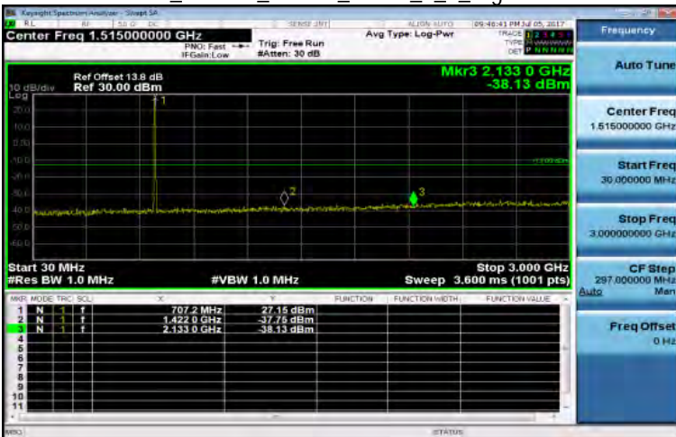
30MHz~3GHz_Band12_10MHz_QPSK_1_0_HighCH23130-711
