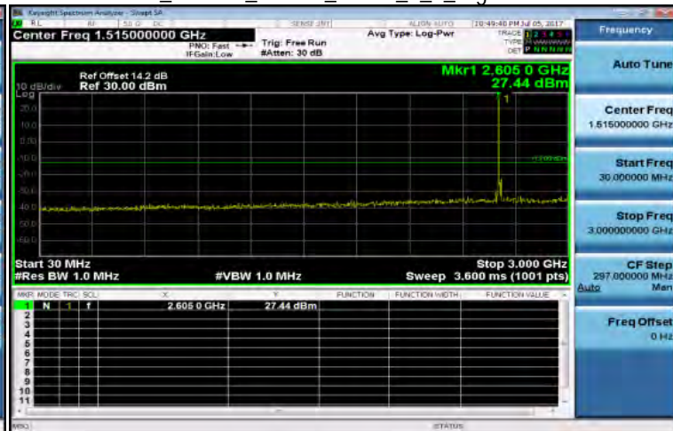
30MHz~3GHz_Band38_15MHz_QPSK_1_0_HighCH38175-2612.5
