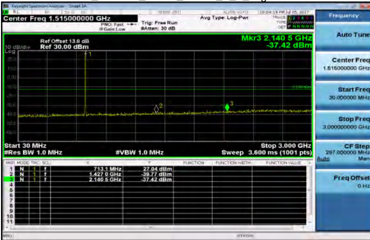
30MHz~3GHz_Band17_5MHz_QPSK_1_0_HighCH23825-713.5
