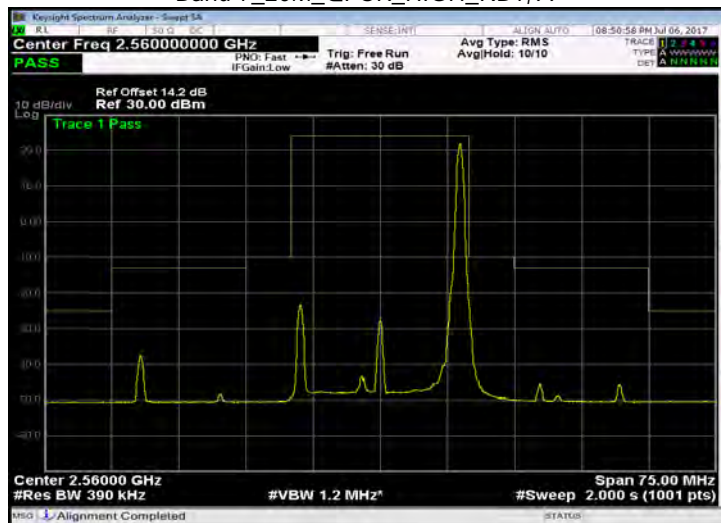
Band 7_20M_QPSK_HIGH_RB100,0
