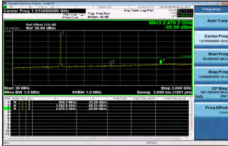
30MHz~3GHz_HSUPA_B5_LowCH4132-826.4
