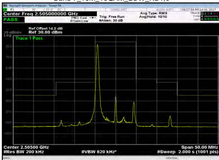
Band 7_10M_16QAM_LOW_RB1,49
