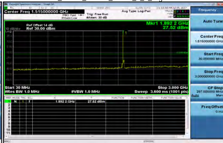
30MHz~3GHz_Band2_20MHz_QPSK_1_0_HighCH19100-1900
