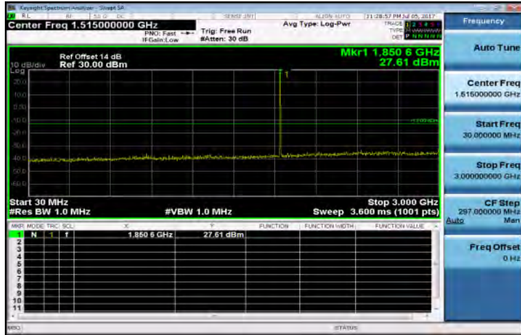
30MHz~3GHz_Band2_1_4MHz_QPSK_1_0_LowCH18607-1850.7
