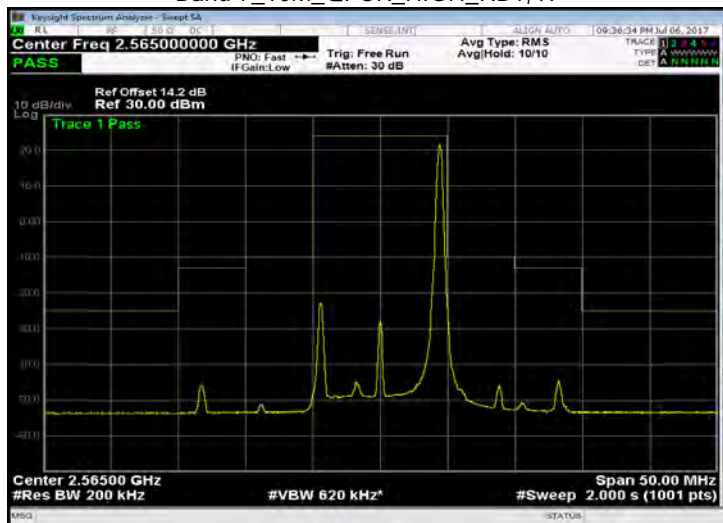
Band 7_10M_QPSK_HIGH_RB50,0
