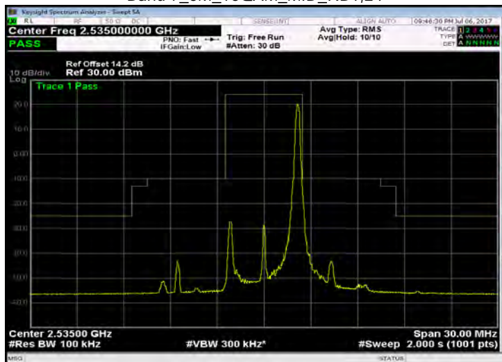
Band 7_5M_16QAM_MID_RB25,0
