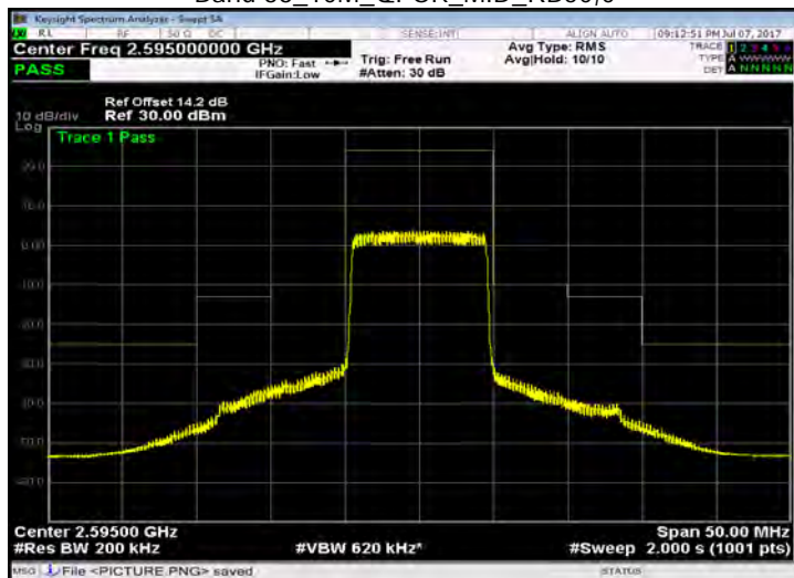
Band 38_10M_QPSK_MID_RB50,0
