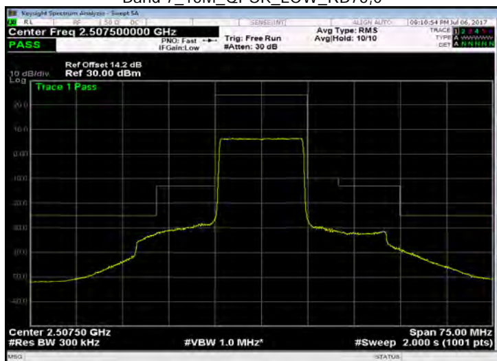
Band 7_15M_QPSK_LOW_RB75,0
