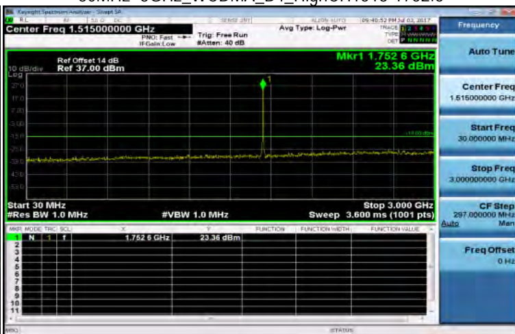
30MHz~3GHz_WCDMA_B4_HighCH1513-1752.6
