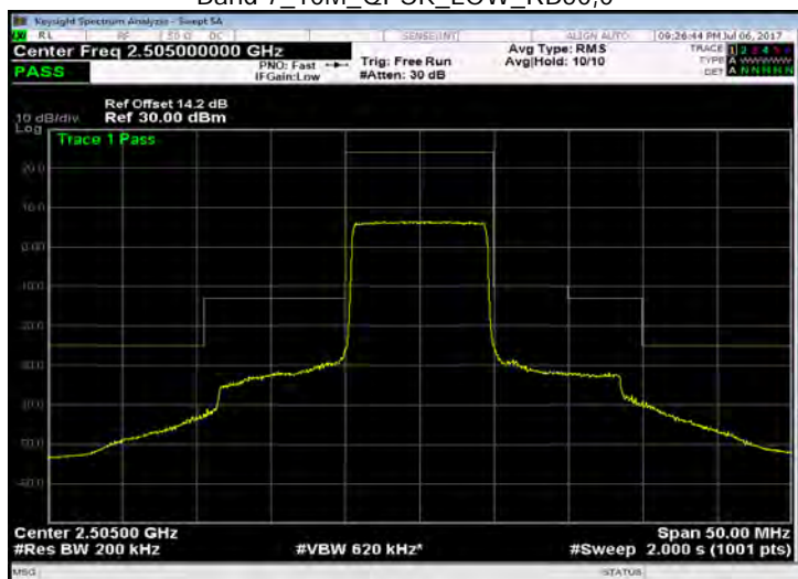
Band 7_10M_QPSK_LOW_RB50,0
