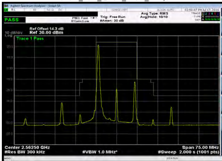
Band 7_15M_QPSK_HIGH_RB1,74
