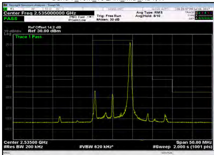
Band 7_10M_16QAM_MID_RB50,0
