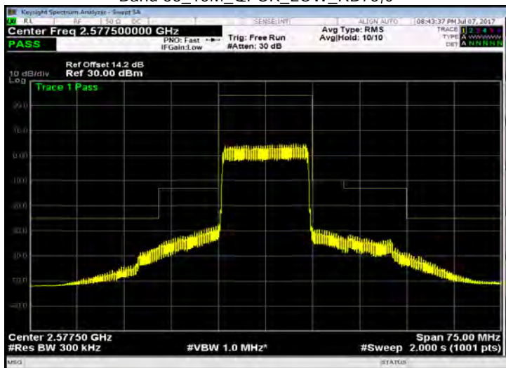
Band 38_15M_QPSK_LOW_RB75,0
