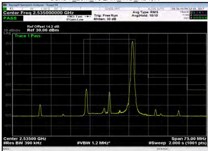
Band 7_20M_16QAM_MID_RB100,0
