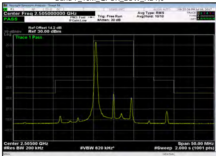
Band 7_10M_QPSK_LOW_RB1,49
