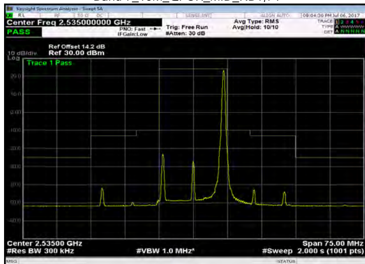
Band 7_15M_QPSK_MID_RB75,0
