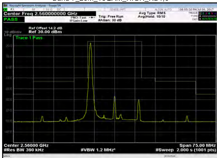
Band 7_20M_16QAM_HIGH_RB1,99
