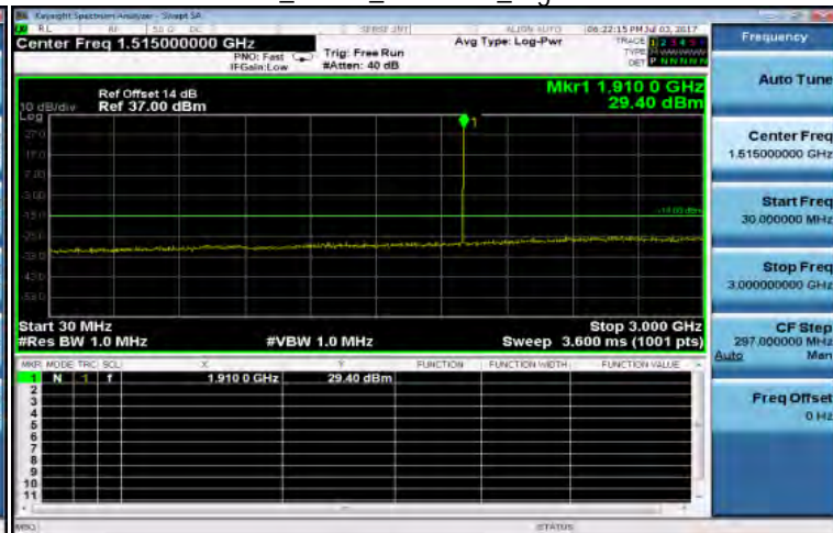
30MHz~3GHz_EDGE_1900MHz_HighCH810-1909.8
