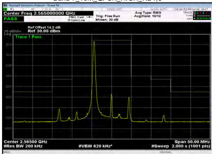
Band 7_10M_QPSK_HIGH_RB1,49
