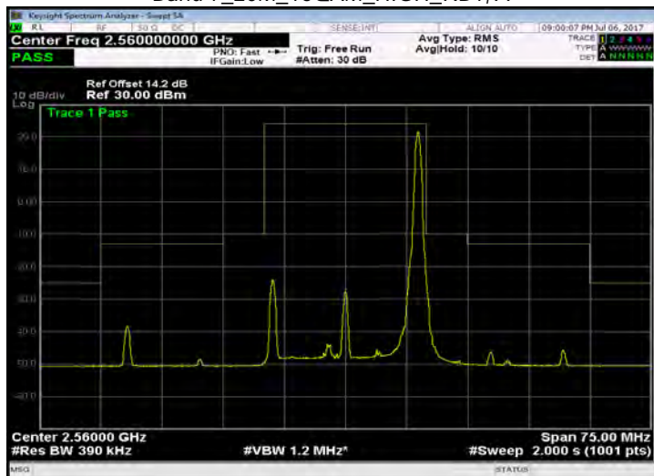
Band 7_20M_16QAM_HIGH_RB100,0
