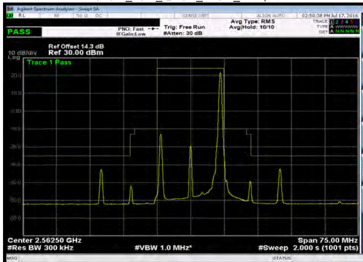
Band 7_15M_QPSK_HIGH_RB75,0
