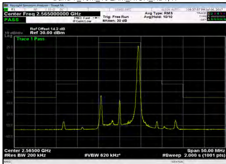
Band 7_10M_16QAM_HIGH_RB50,0
