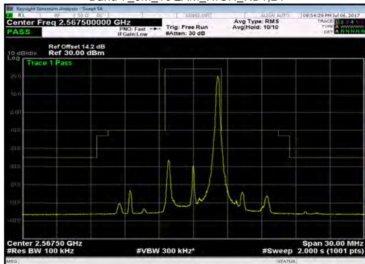
Band 7_5M_16QAM_HIGH_RB25,0
