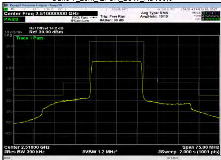
Band 7_20M_QPSK_LOW_RB100,0
