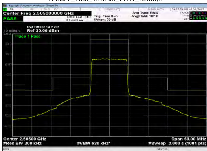
Band 7_10M_16QAM_LOW_RB50,0
