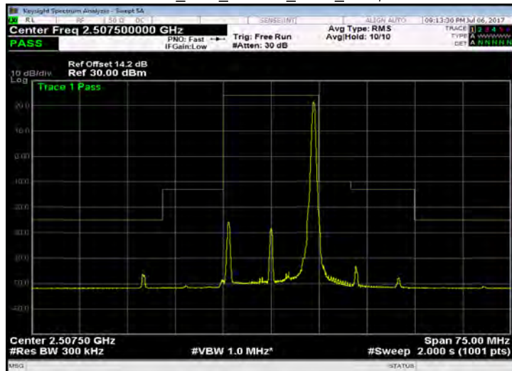
Band 7_15M_16QAM_LOW_RB75,0
