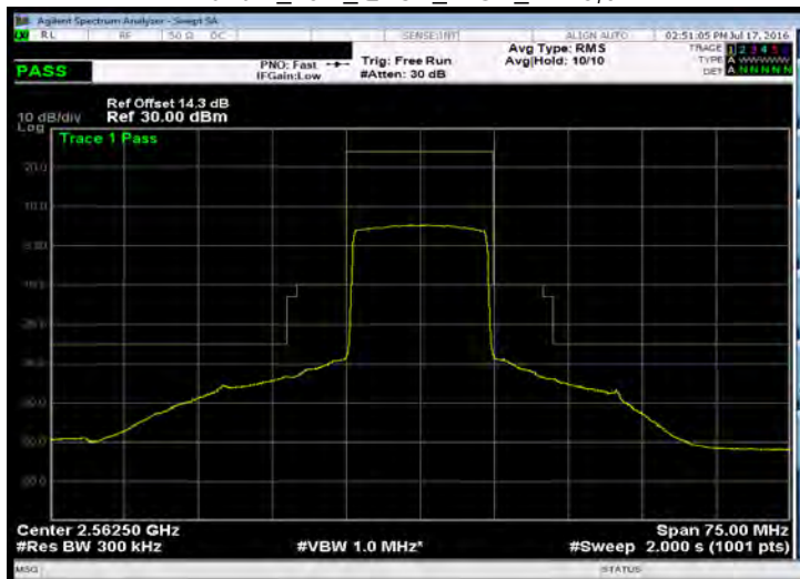
Band 7_15M_QPSK_HIGH_RB75,0
