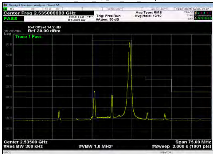
Band 7_15M_16QAM_MID_RB75,0
