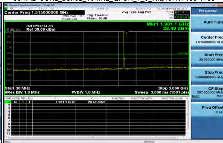
30MHz~3GHz_Band2_10MHz_QPSK_1_0_HighCH19150-1905
