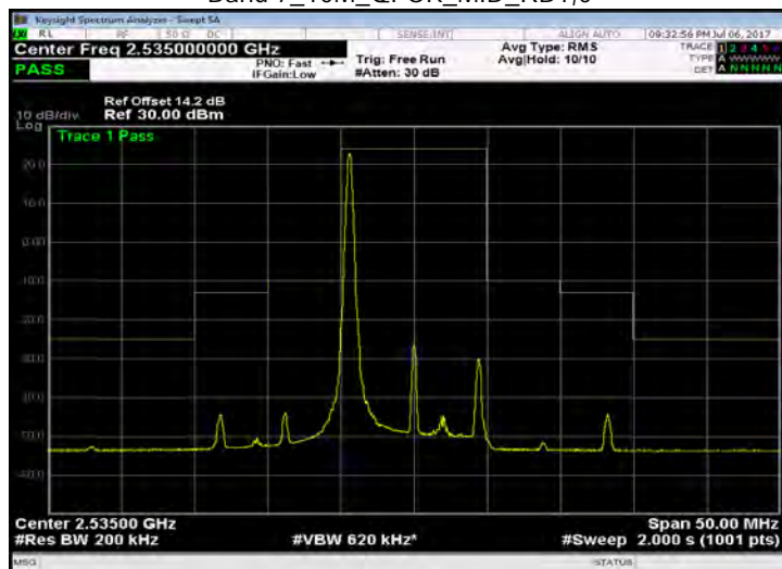
Band 7_10M_QPSK_MID_RB1,49
