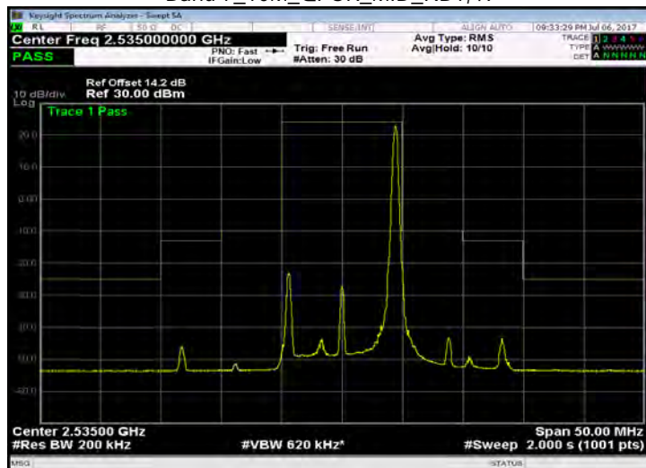
Band 7_10M_QPSK_MID_RB50,0
