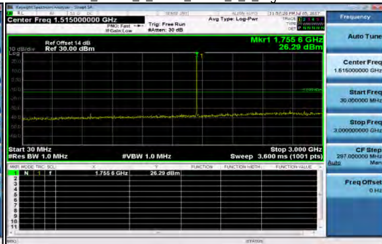
30MHz~3GHz_Band4_1_4MHz_QPSK_1_0_HighCH20393-1754.3
