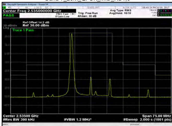
Band 7_20M_QPSK_MID_RB1,99
