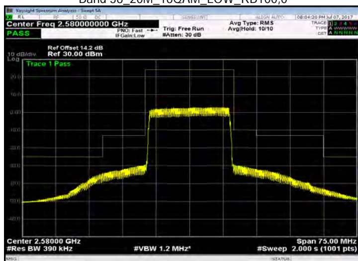
Band 38_20M_16QAM_LOW_RB100,0
