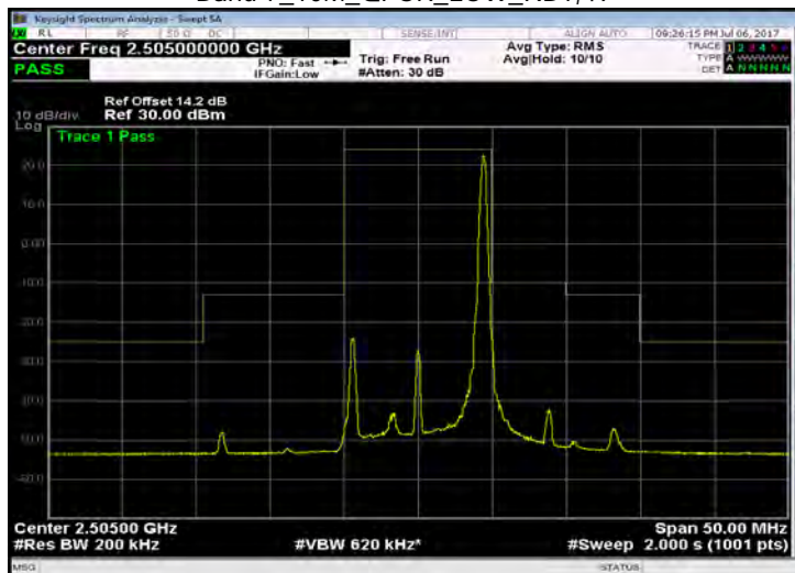
Band 7_10M_QPSK_LOW_RB50,0
