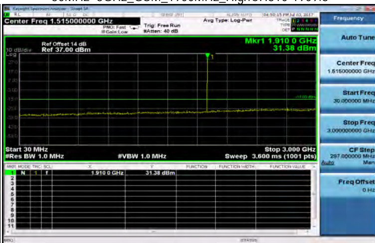
30MHz~3GHz_GSM_1900MHz_HighCH810-1909.8
