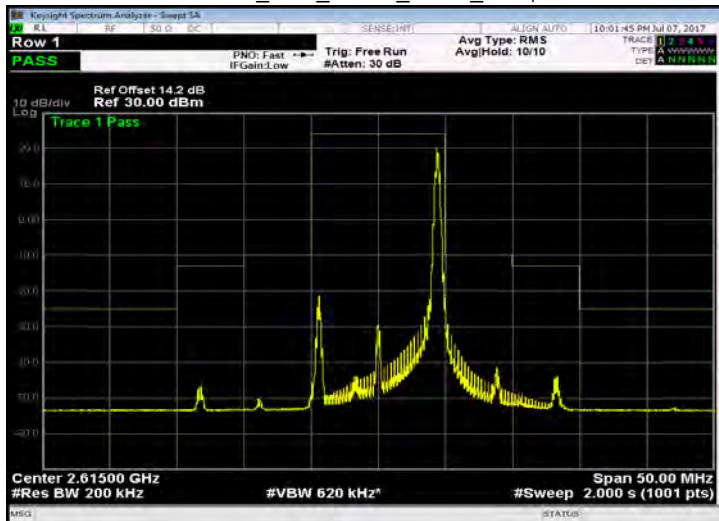
Band 38_10M_QPSK_HIGH_RB50,0
