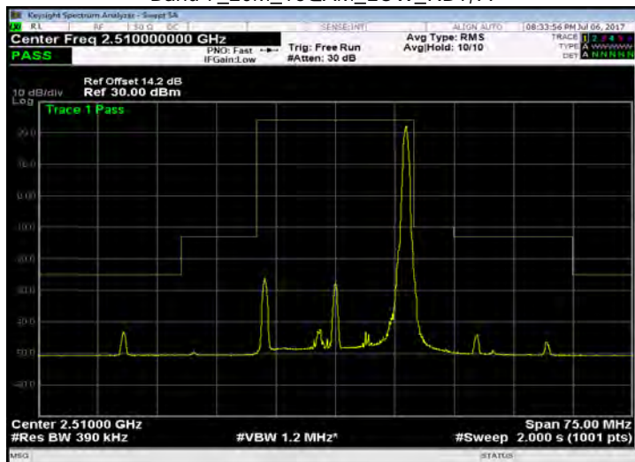
Band 7_20M_16QAM_LOW_RB100,0
