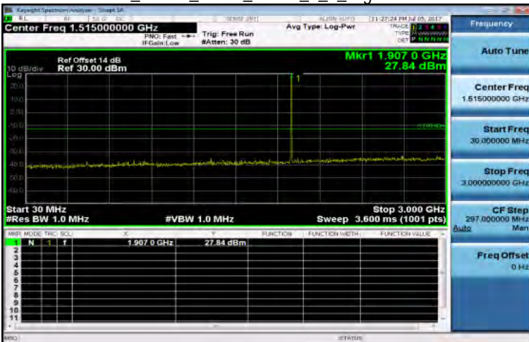
30MHz~3GHz_Band2_3MHz_QPSK_1_0_HighCH19185-1908.5
