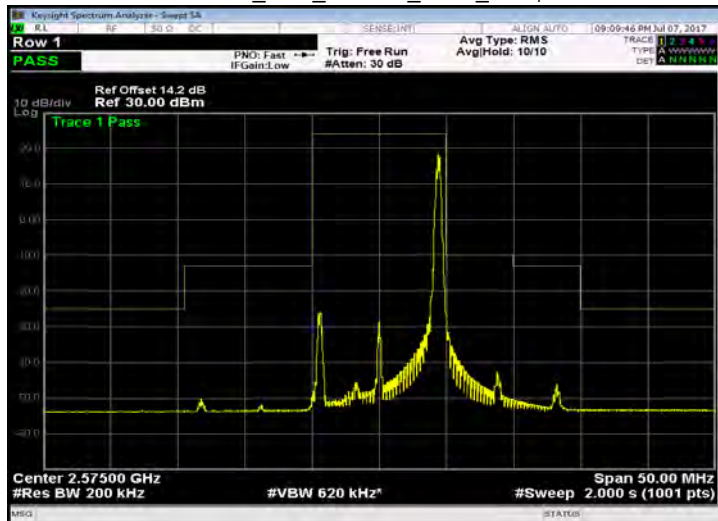
Band 38_10M_16QAM_LOW_RB50,0
