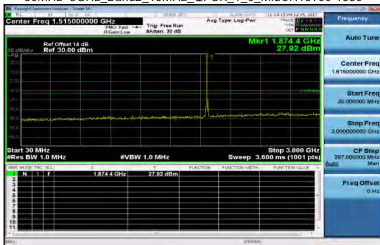
30MHz~3GHz_Band2_15MHz_QPSK_1_0_MidCH18900-1880
