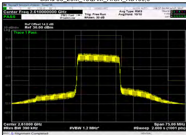
Band 38_20M_16QAM_HIGH_RB100,0
