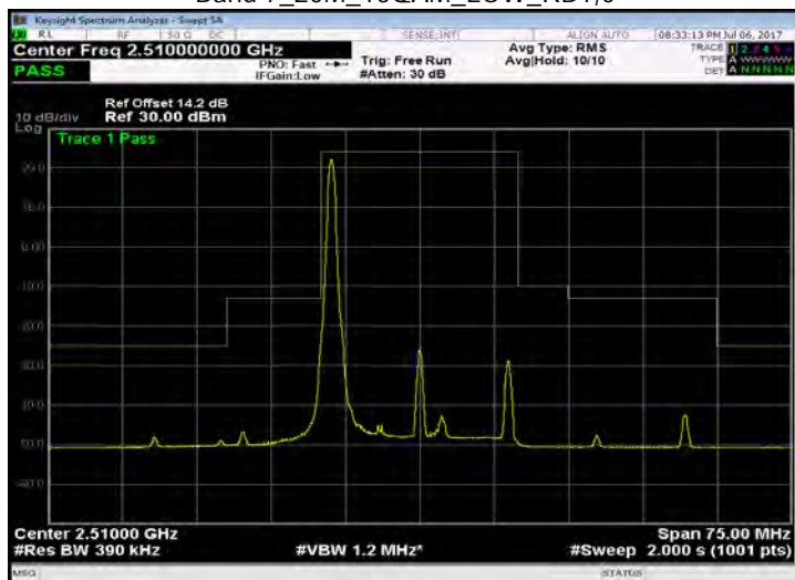
Band 7_20M_16QAM_LOW_RB1,99
