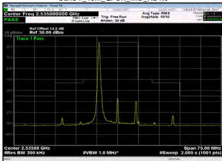
Band 7_15M_QPSK_MID_RB1,74
