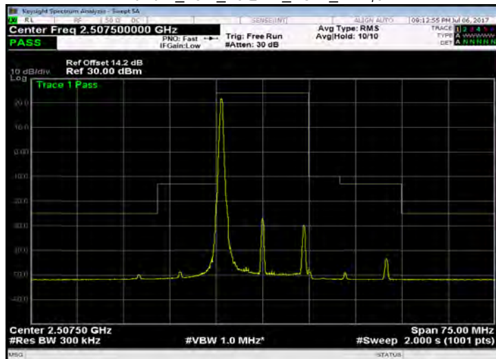
Band 7_15M_16QAM_LOW_RB1,74
