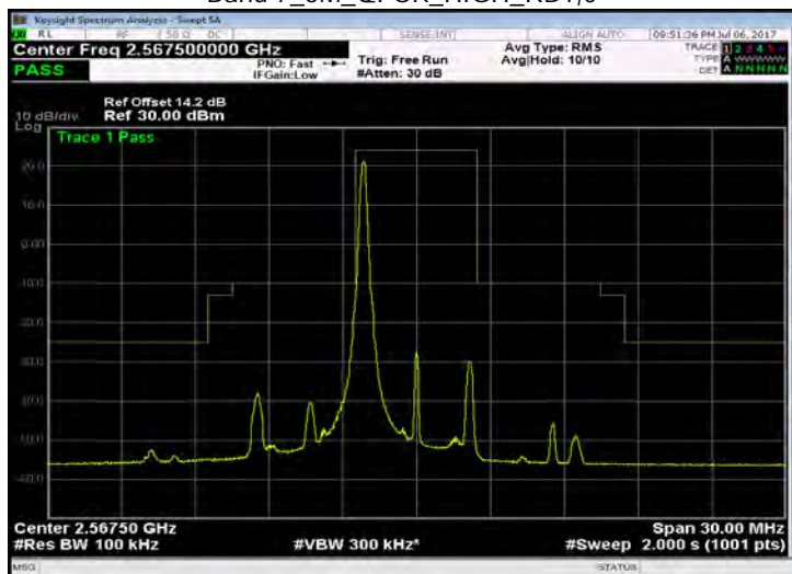
Band 7_5M_QPSK_HIGH_RB1,24
