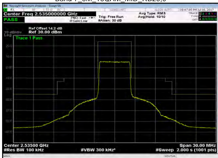
Band 7_5M_16QAM_MID_RB25,0
