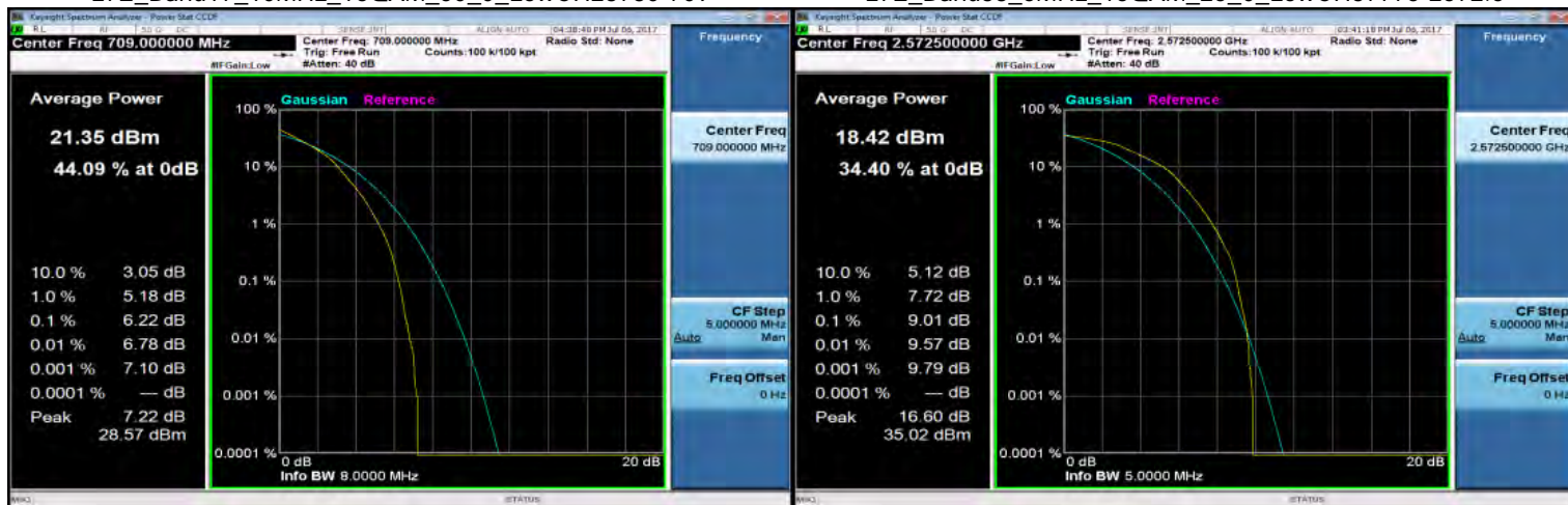
LTE_Band17_10MHz_16QAM_50_0_LowCH23780-709
