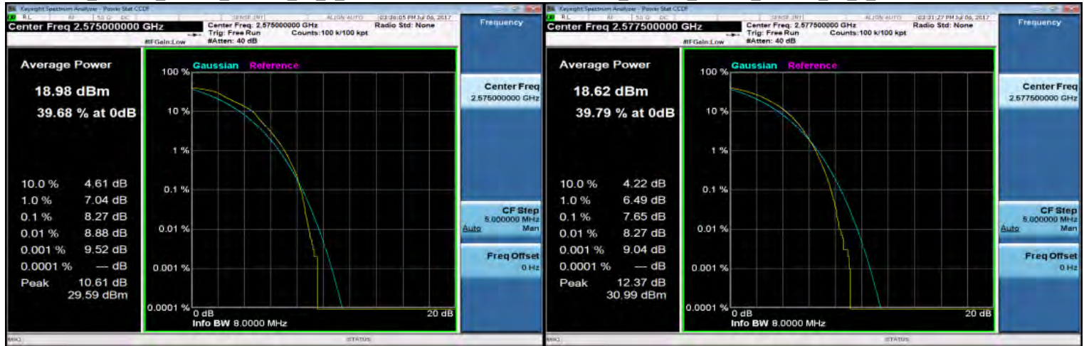
LTE_Band38_10MHz_16QAM_50_0_LowCH37800-2575
