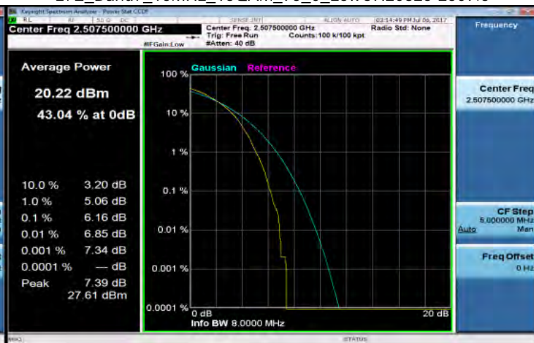
LTE_Band7_15MHz_16QAM_75_0_LowCH20825-2507.5
