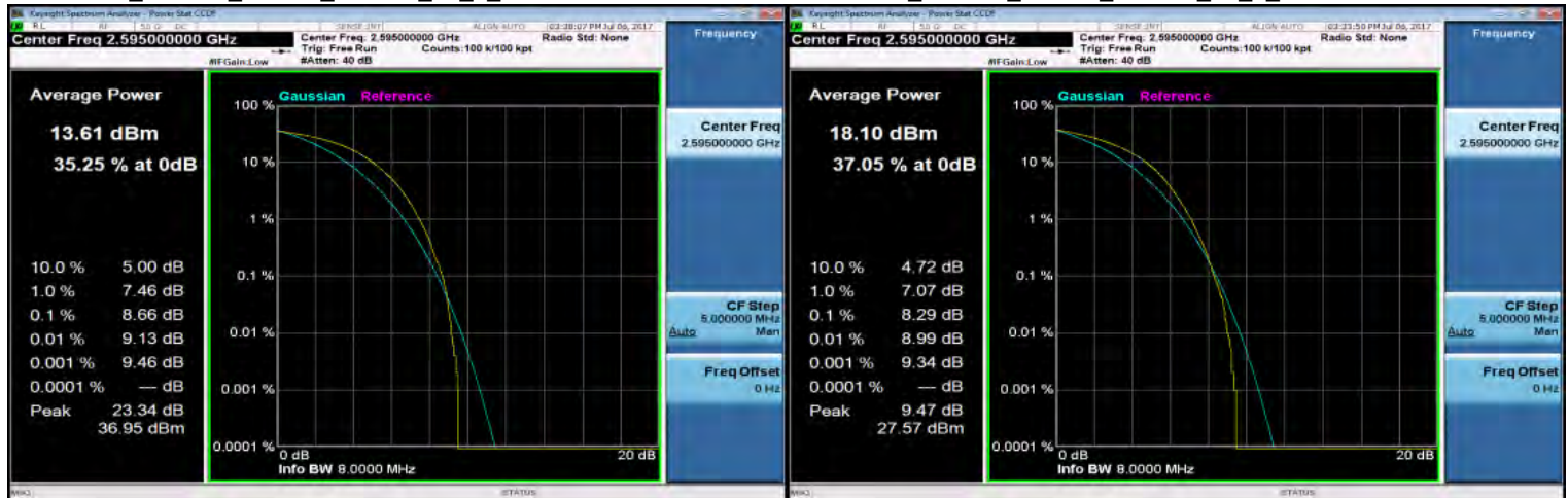
LTE_Band38_10MHz_16QAM_50_0_MidCH38000-2595
