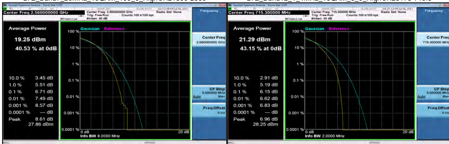
LTE_Band7_20MHz_16QAM_100_0_HighCH21350-2560
