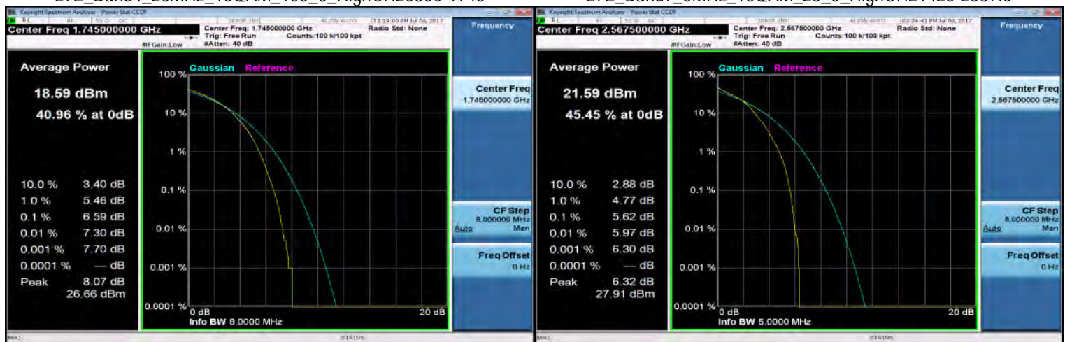
LTE_Band4_20MHz_16QAM_100_0_HighCH20300-1745
