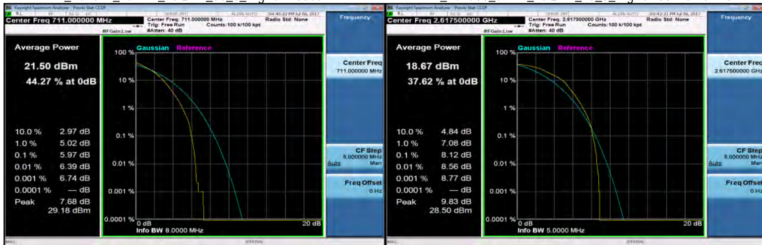
LTE_Band17_10MHz_16QAM_50_0_HighCH23800-711
