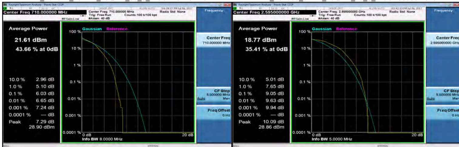
LTE_Band17_10MHz_16QAM_50_0_MidCH23790-710
