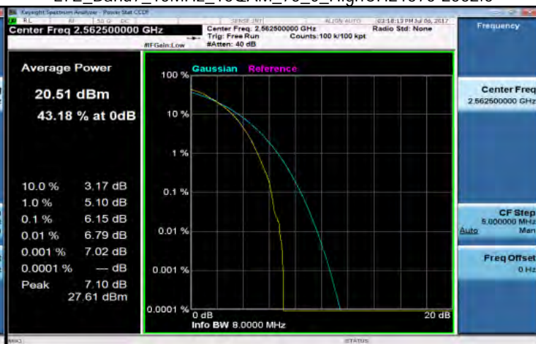
LTE_Band7_15MHz_16QAM_75_0_HighCH21375-2562.5
