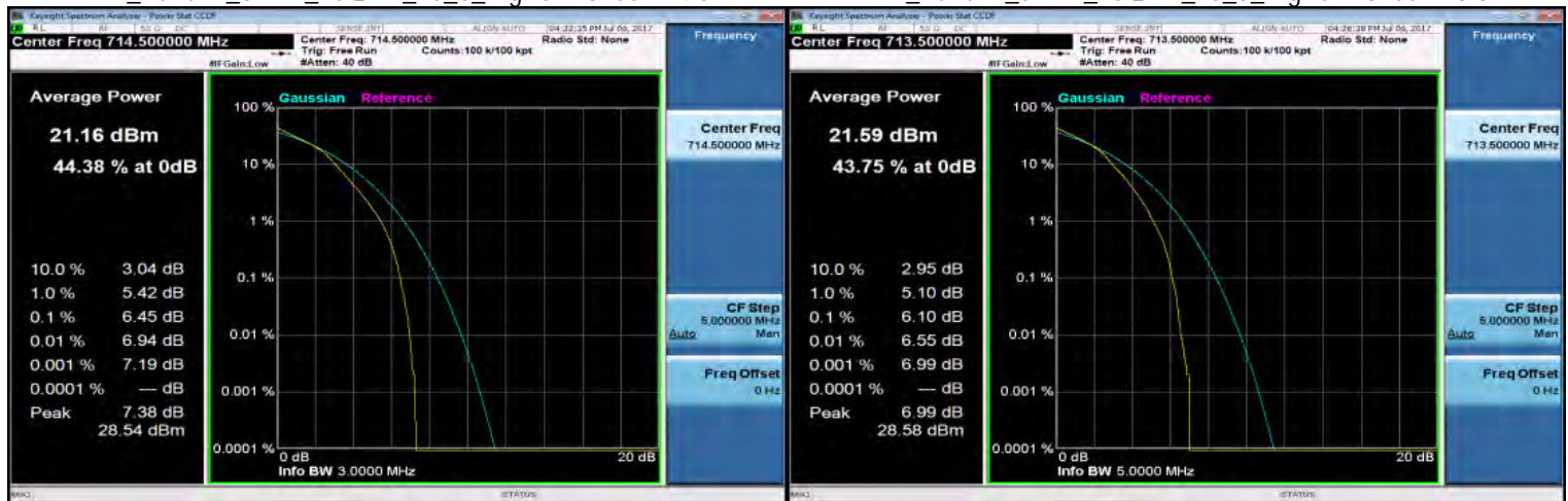
LTE_Band12_3MHz_16QAM_15_0_HighCH23165-714.5
