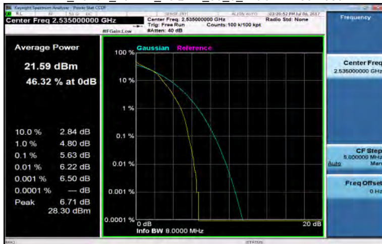
LTE_Band7_10MHz_16QAM_50_0_MidCH21100-2535
