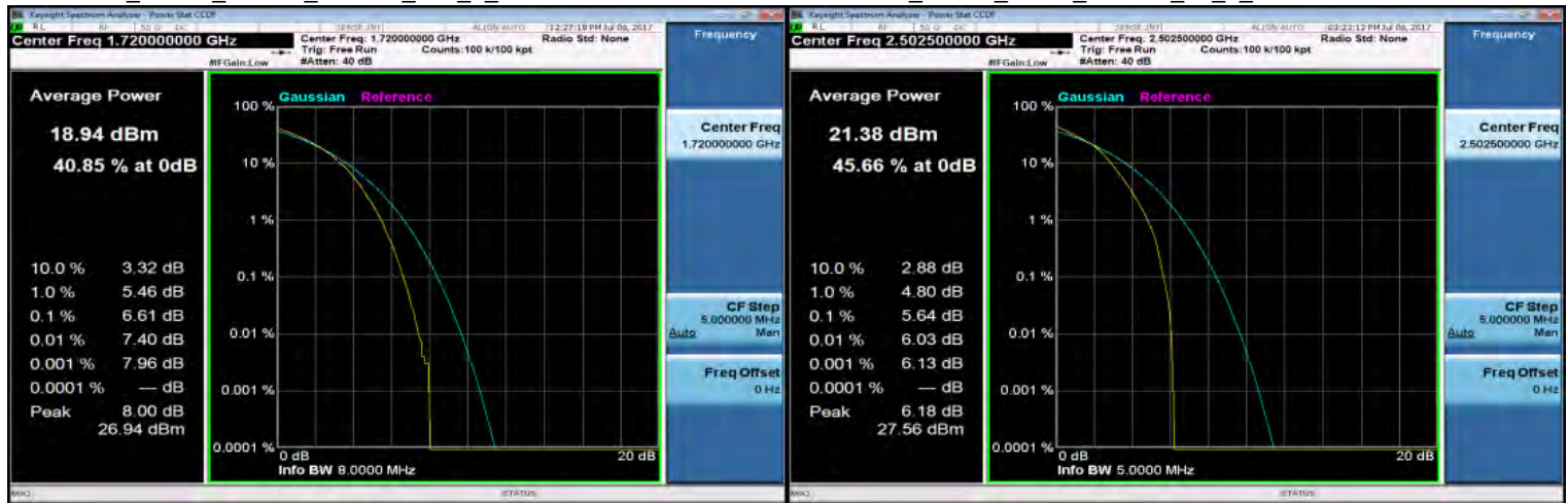
LTE_Band4_20MHz_16QAM_100_0_LowCH20050-1720
