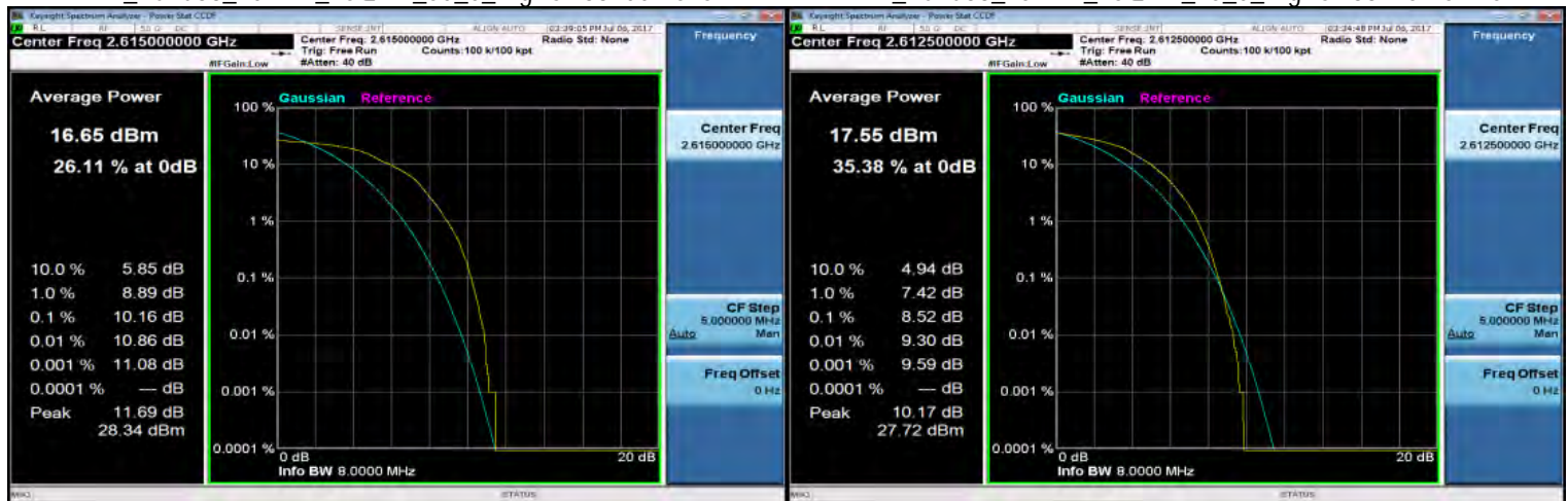
LTE_Band38_10MHz_16QAM_50_0_HighCH38200-2615
