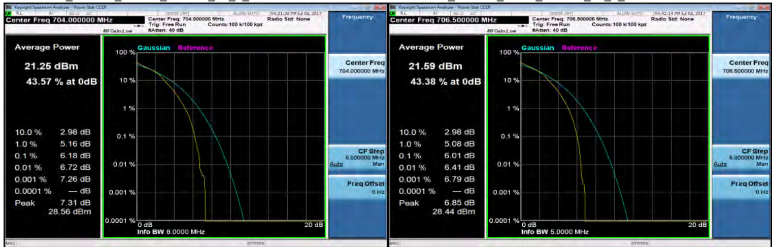
LTE_Band12_10MHz_16QAM_50_0_LowCH23060-704
