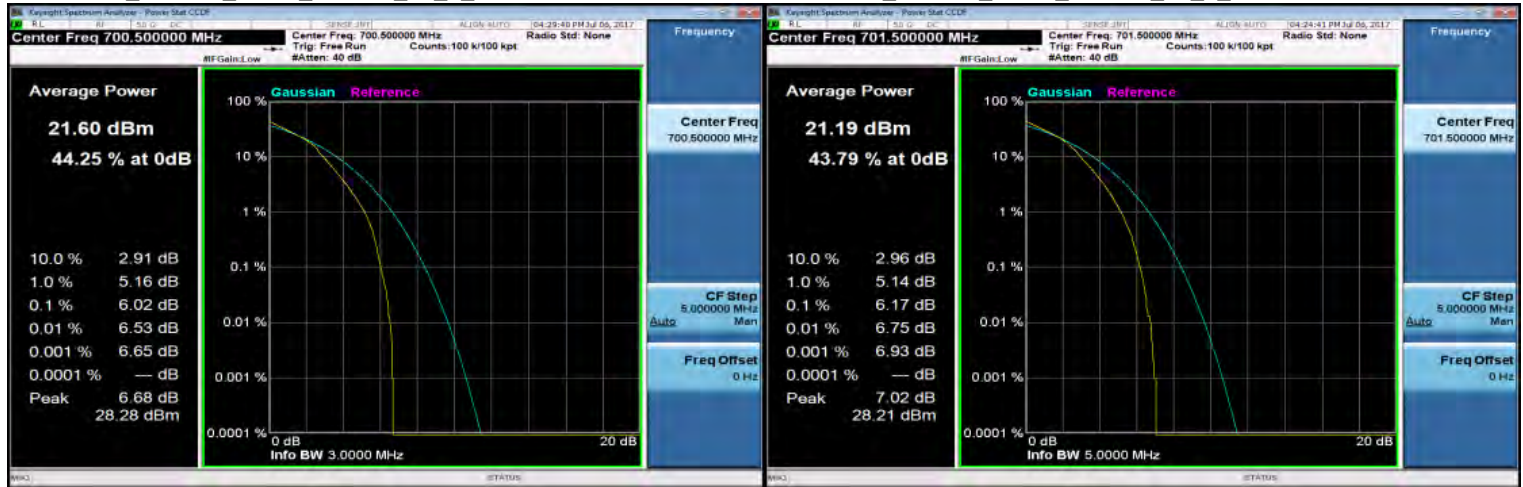
LTE_Band12_3MHz_16QAM_15_0_LowCH23025-700.5
