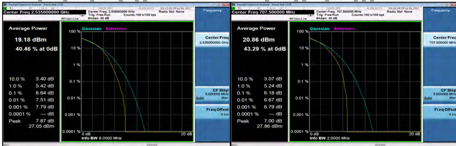
LTE_Band7_20MHz_16QAM_100_0_MidCH21100-2535
