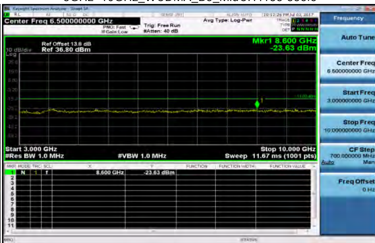
3GHz~10GHz_WCDMA_B5_MidCH4183-836.6
