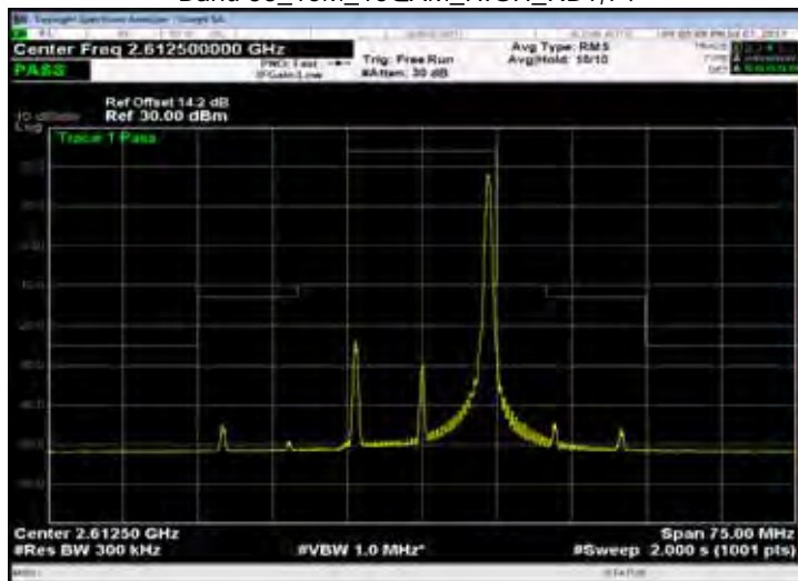
Band 38_15M_16QAM_HIGH_RB75,0
