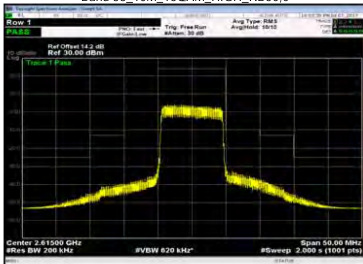
Band 38_10M_16QAM_HIGH_RB50,0
