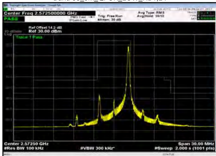
Band 38_5M_QPSK_LOW_RB25,0
