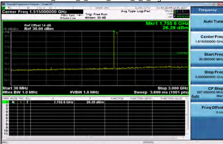
30MHz~3GHz_Band4_1_4MHz_QPSK_1_0_HighCH20393-1754.3
