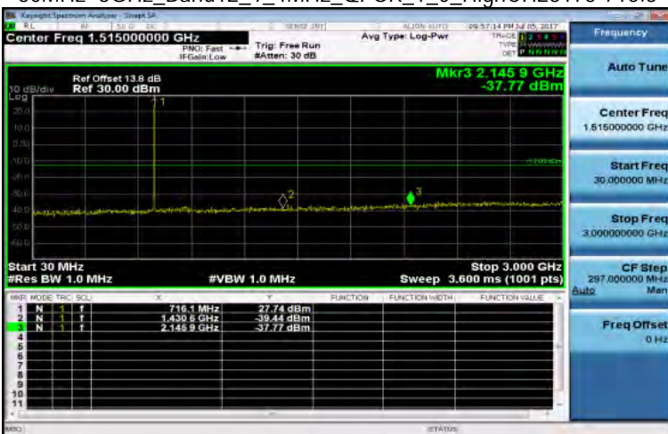
30MHz~3GHz_Band12_1_4MHz_QPSK_1_0_HighCH23173-715.3
