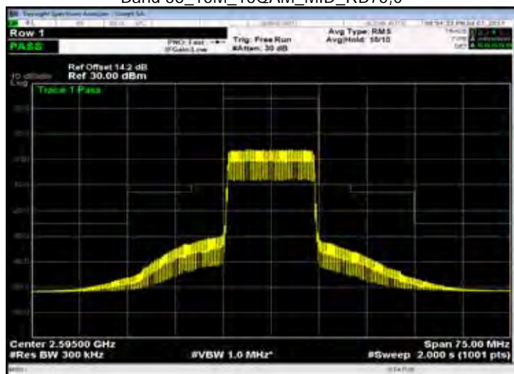
Band 38_15M_16QAM_MID_RB75,0
