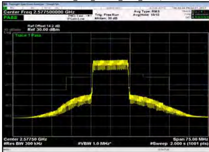
Band 38_15M_16QAM_LOW_RB75,0
