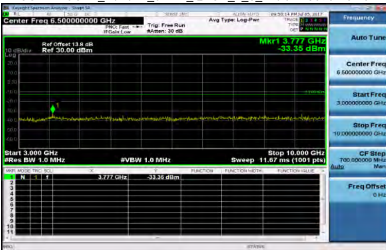
3GHz~10GHz_Band12_5MHz_QPSK_1_0_MidCH23095-707.5
