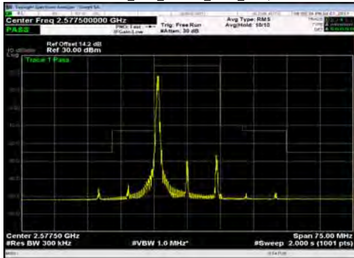
Band 38_15M_16QAM_LOW_RB1,74
