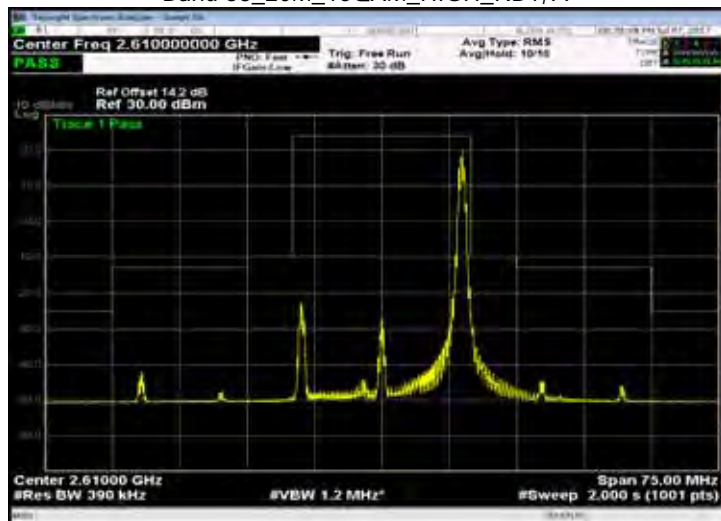
Band 38_20M_16QAM_HIGH_RB100,0
