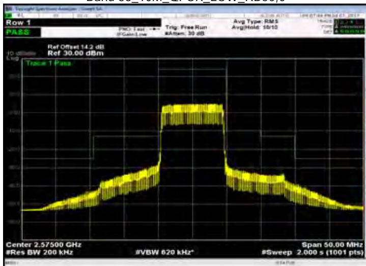
Band 38_10M_QPSK_LOW_RB50,0
