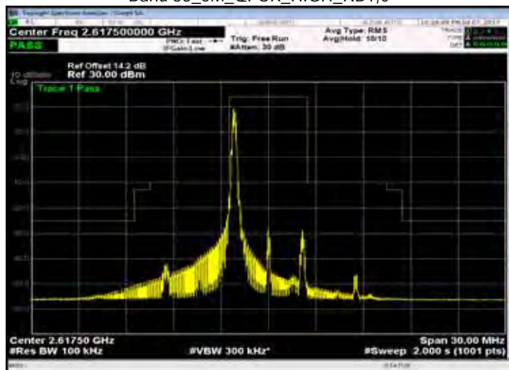
Band 38_5M_QPSK_HIGH_RB1,24
