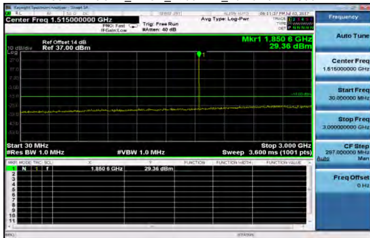
30MHz~3GHz_EDGE_1900MHz_LowCH512-1850.2
