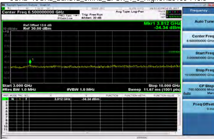
3GHz~10GHz_Band12_5MHz_QPSK_1_0_HighCH23155-713.5
