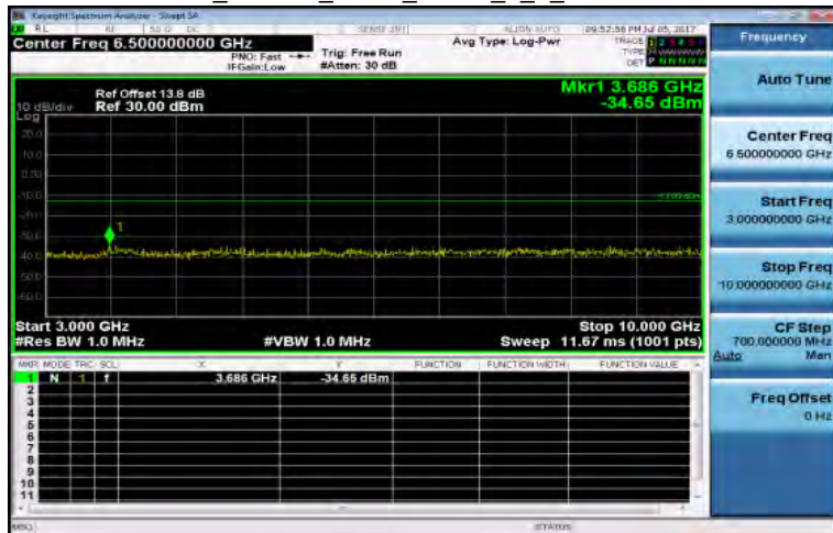
3GHz~10GHz_Band12_3MHz_QPSK_1_0_LowCH23025-700.5
