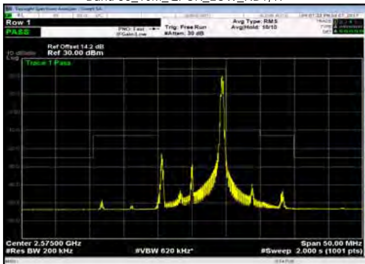
Band 38_10M_QPSK_LOW_RB50,0
