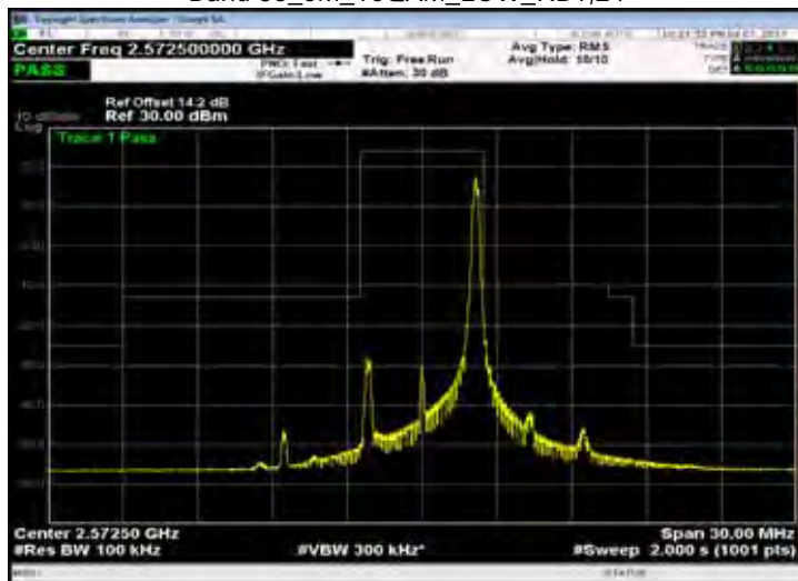
Band 38_5M_16QAM_LOW_RB25,0
