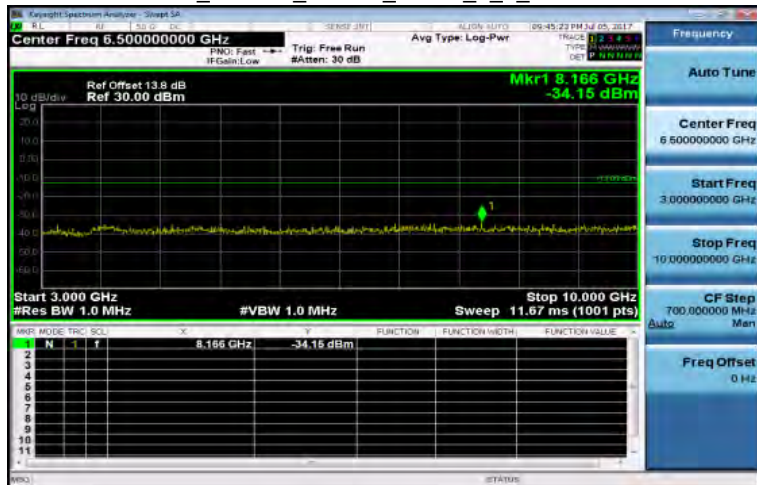
3GHz~10GHz_Band12_10MHz_QPSK_1_0_LowCH23060-704
