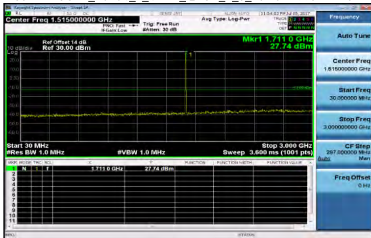
30MHz-3GHz_Band4_1_4MHz_QPSK_1_0_LowCH19957-1710.7
