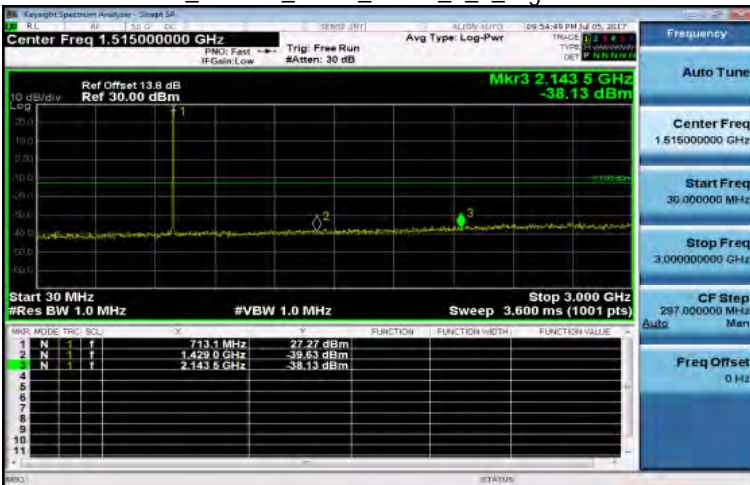
30MHz~3GHz_Band12_3MHz_QPSK_1_0_HighCH23165-714.5
