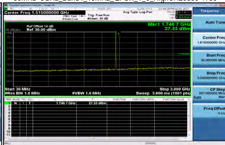
30MHz~3GHz_Band4_10MHz_QPSK_1_0_HighCH20350-1750
