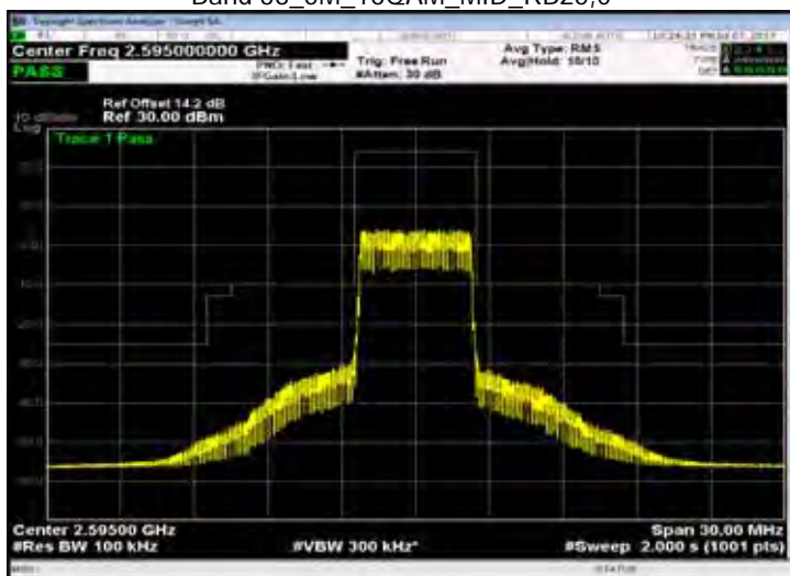
Band 38_5M_16QAM_MID_RB25,0
