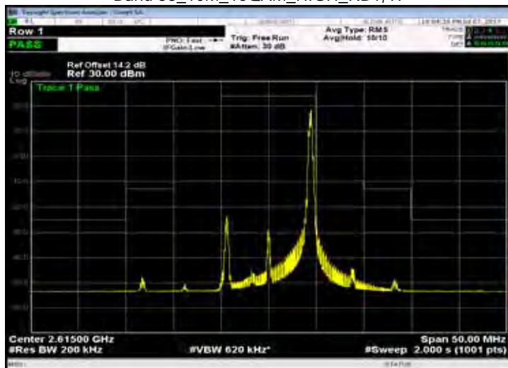
Band 38_10M_16QAM_HIGH_RB50,0
