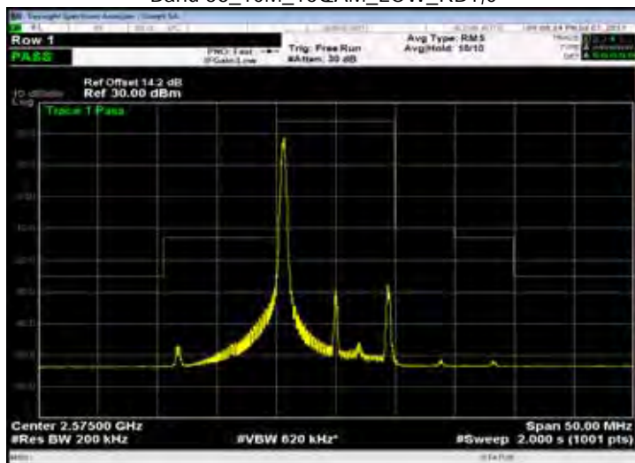
Band 38_10M_16QAM_LOW_RB1,49
