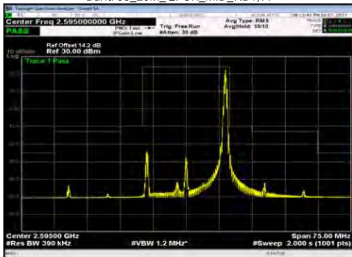
Band 38_20M_QPSK_MID_RB100,0
