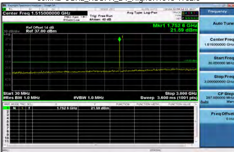
30MHz~3GHz_HSUPA_B4_HighCH1513-1752.6
