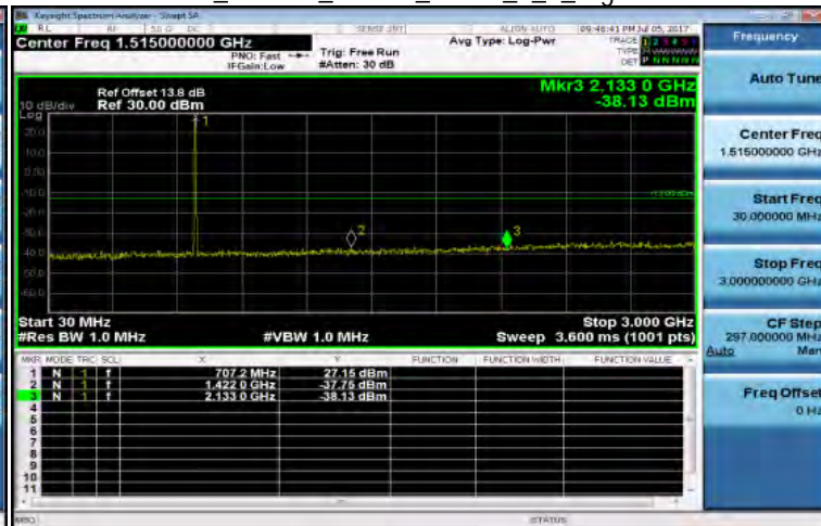
30MHz~3GHz_Band12_10MHz_QPSK_1_0_HighCH23130-711
