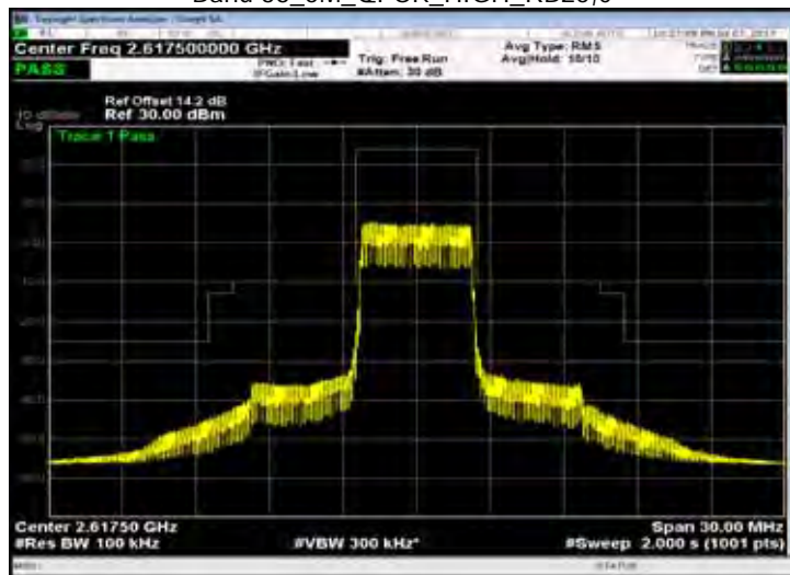
Band 38_5M_QPSK_HIGH_RB25,0
