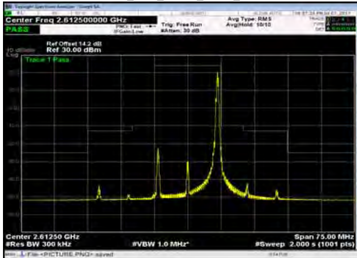
Band 38_15M_QPSK_HIGH_RB75,0
