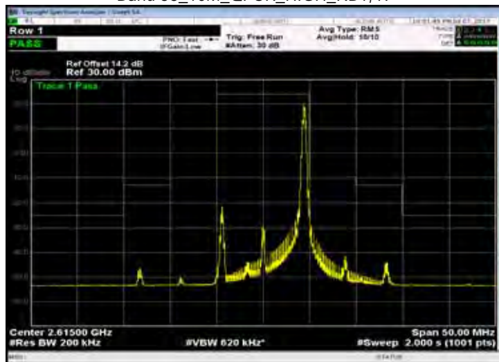
Band 38_10M_QPSK_HIGH_RB50,0
