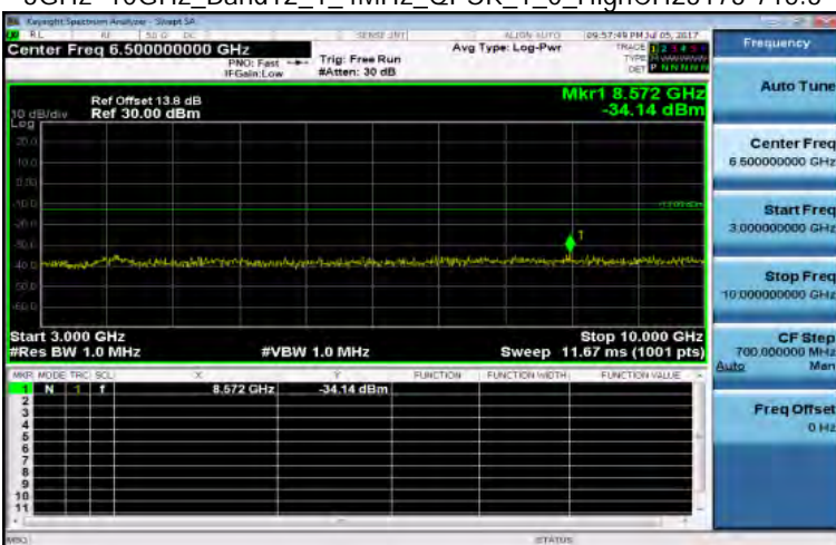
3GHz~10GHz_Band12_1_4MHz_QPSK_1_0_HighCH23173-715.3
