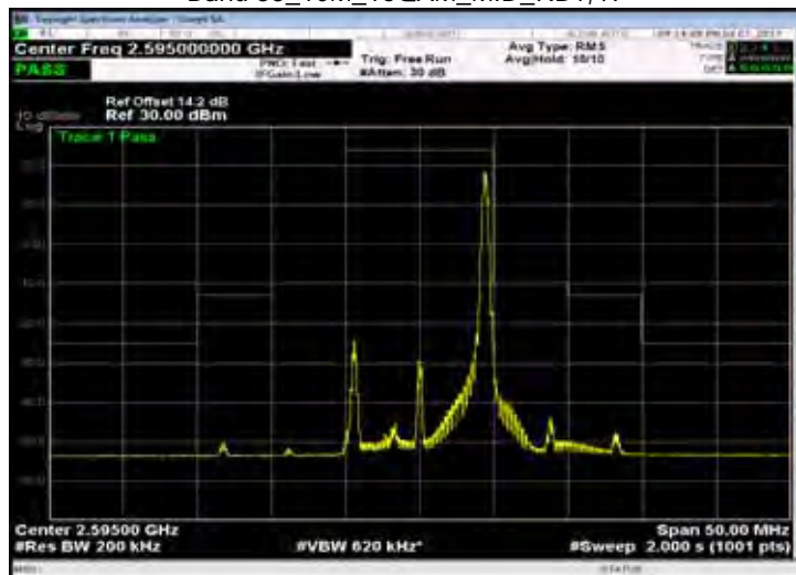
Band 38_10M_16QAM_MID_RB50,0
