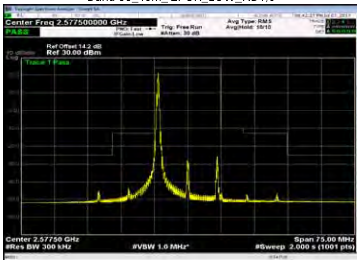
Band 38_15M_QPSK_LOW_RB1,74
