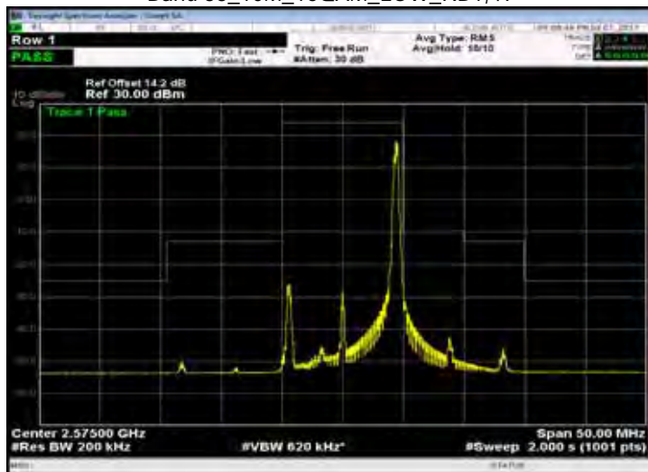
Band 38_10M_16QAM_LOW_RB50,0
