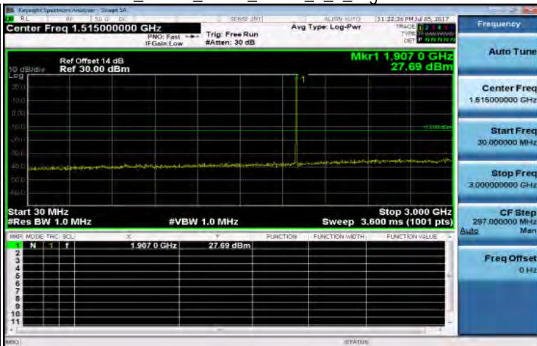
30MHz~3GHz_Band2_5MHz_QPSK_1_0_HighCH19175-1907.5
