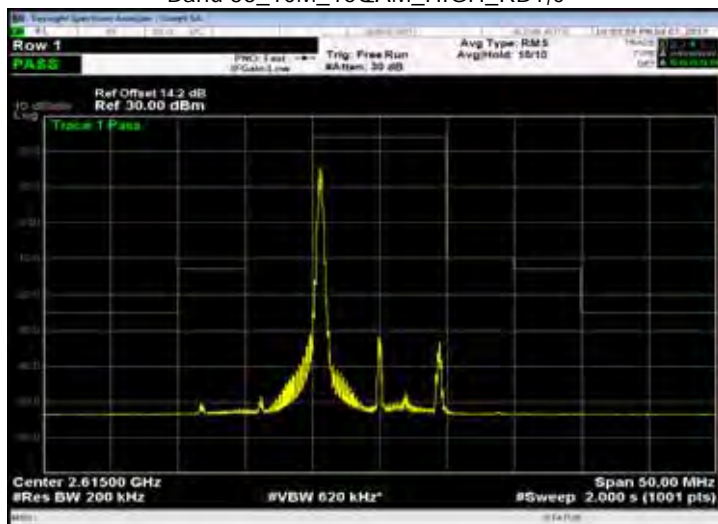
Band 38_10M_16QAM_HIGH_RB1,49
