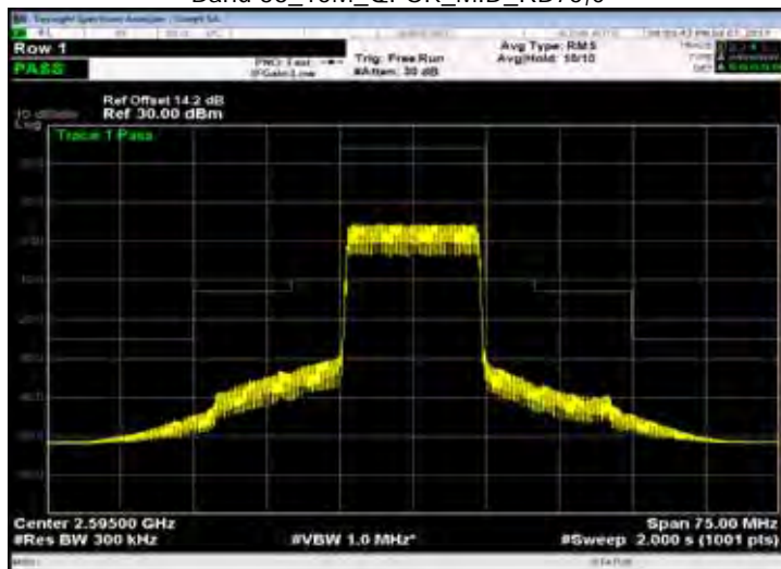
Band 38_15M_QPSK_MID_RB75,0
