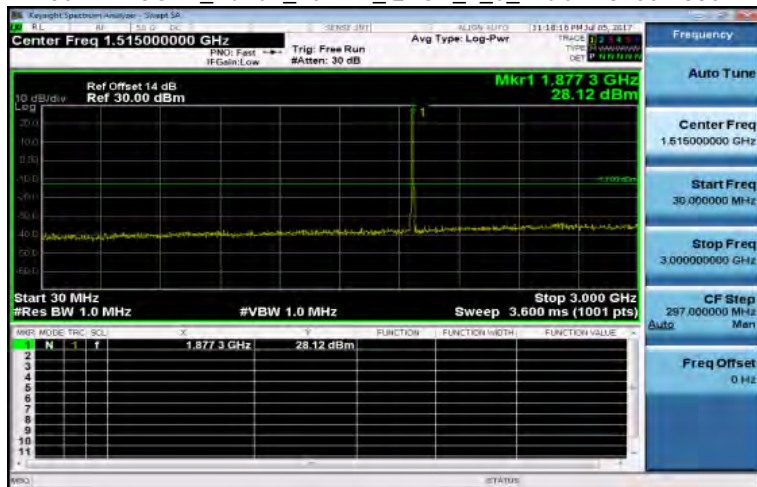
30MHz~3GHz_Band2_10MHz_QPSK_1_0_MidCH1890-1880
