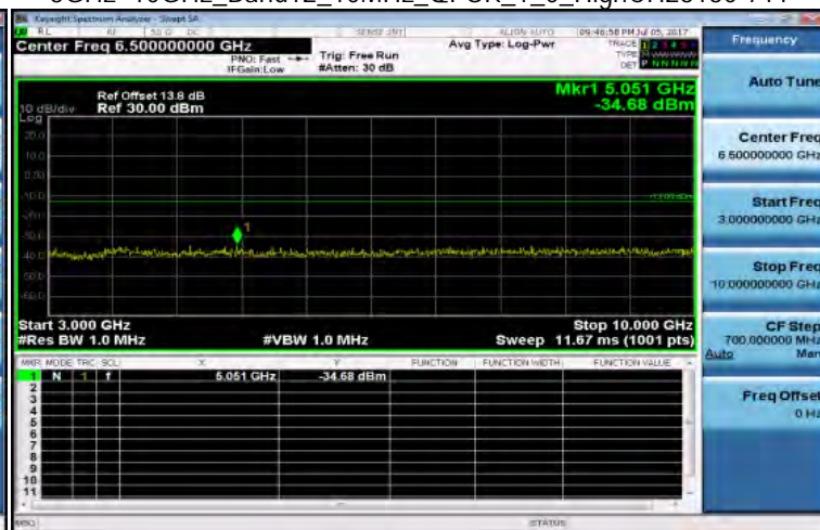
3GHz~10GHz_Band12_10MHz_QPSK_1_0_HighCH23130-711
