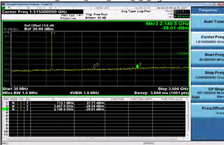
30MHz~3GHz_Band12_5MHz_QPSK_1_0_HighCH23155-713.5
