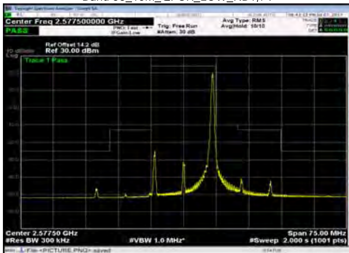
Band 38_15M_QPSK_LOW_RB75,0
