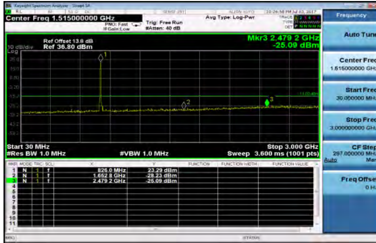
30MHz~3GHz_HSUPA_B5_LowCH4132-826.4
