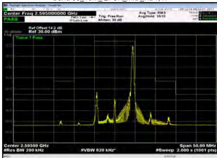
Band 38_10M_QPSK_MID_RB50,0
