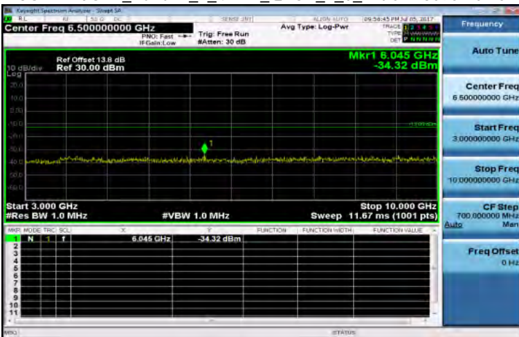
3GHz~10GHz_Band12_1_4MHz_QPSK_1_0_MidCH23095-707.5
