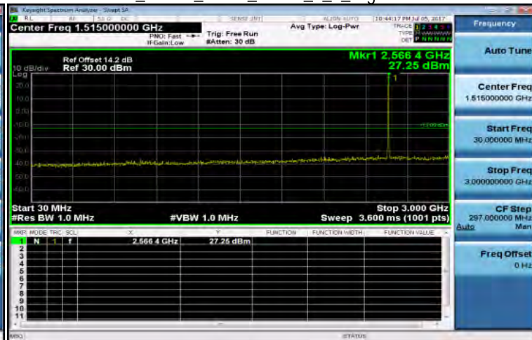
30MHz~3GHz_Band7_5MHz_QPSK_1_0_HighCH21425-2567.5
