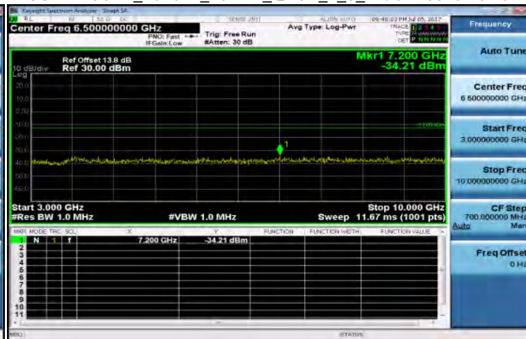
3GHz~10GHz_Band12_10MHz_QPSK_1_0_MidCH23095-707.5
