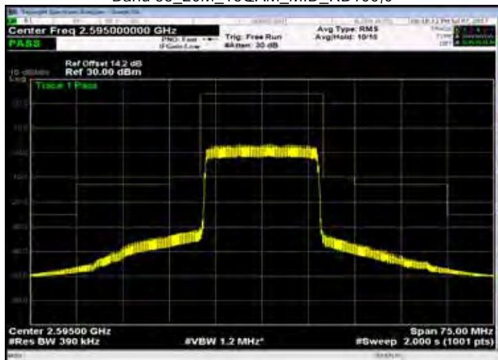
Band 38_20M_16QAM_MID_RB100,0
