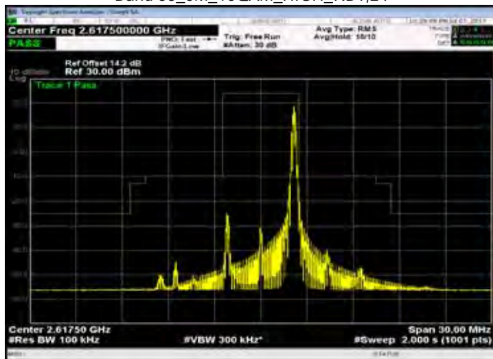
Band 38_5M_16QAM_HIGH_RB25,0
