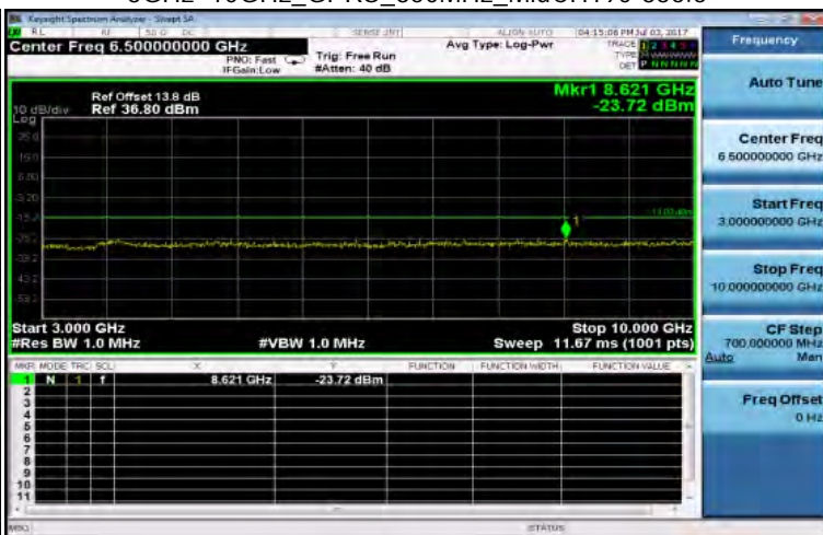
3GHz~10GHz_GPRS_850MHz_MidCH190-836.6
