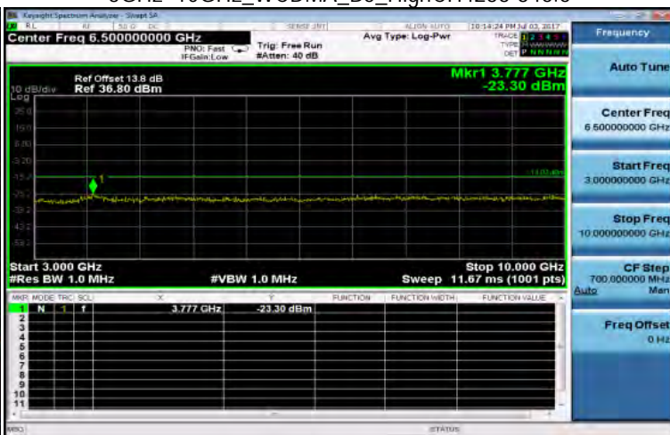
3GHz~10GHz_WCDMA_B5_HighCH4233-846.6
