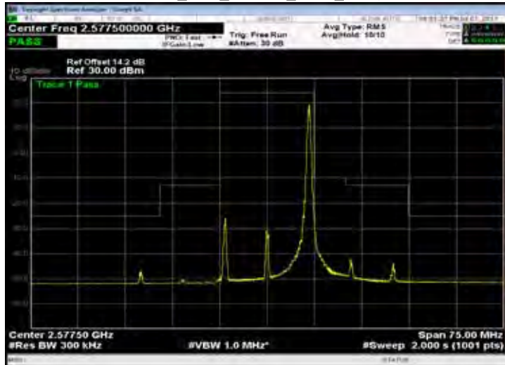
Band 38_15M_16QAM_LOW_RB75,0
