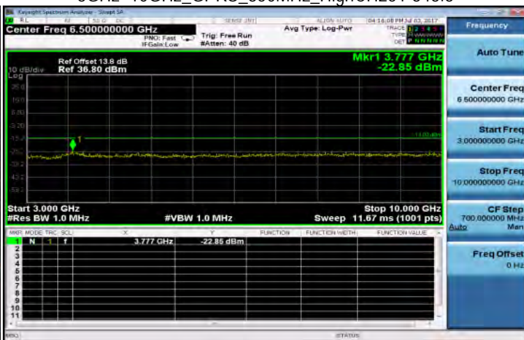
3GHz~10GHz_GPRS_850MHz_HighCH251-848.8
