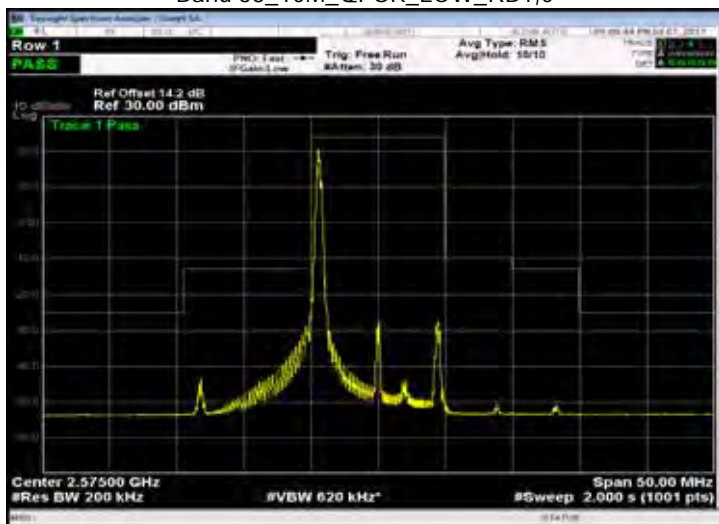
Band 38_10M_QPSK_LOW_RB1,49
