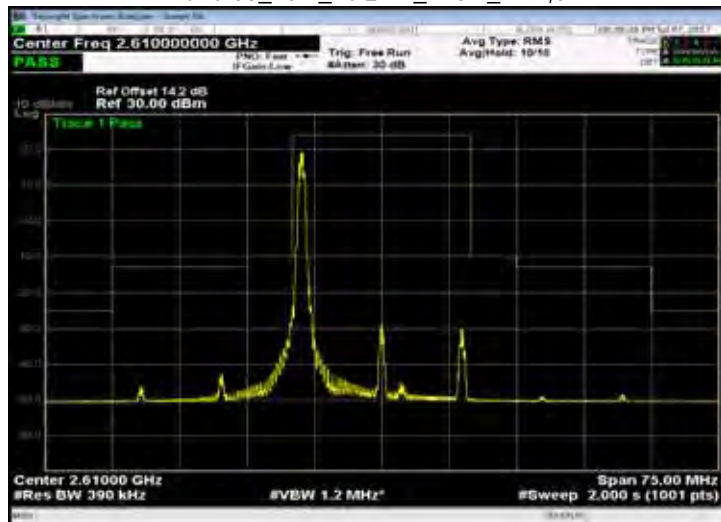
Band 38_20M_16QAM_HIGH_RB1,99
