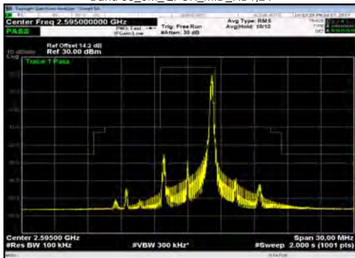
Band 38_5M_QPSK_MID_RB25,0
