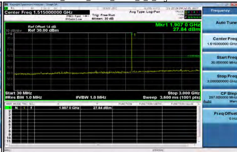
30MHz~3GHz_Band2_3MHz_QPSK_1_0_HighCH19185-1908.5
