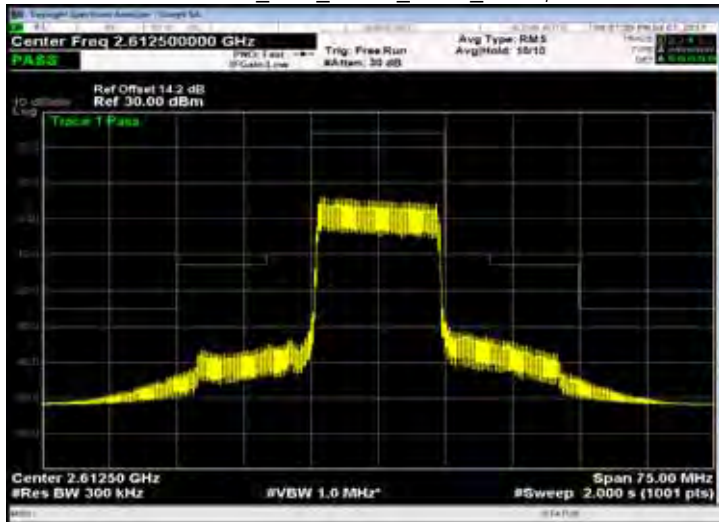
Band 38_15M_QPSK_HIGH_RB75,0
