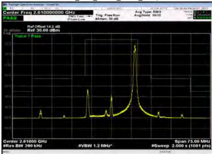
Band 38_20M_QPSK_HIGH_RB100,0
