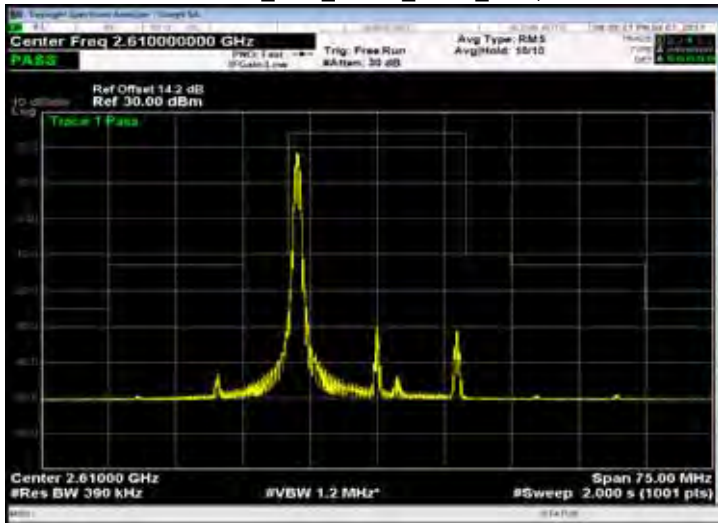
Band 38_20M_QPSK_HIGH_RB1,99
