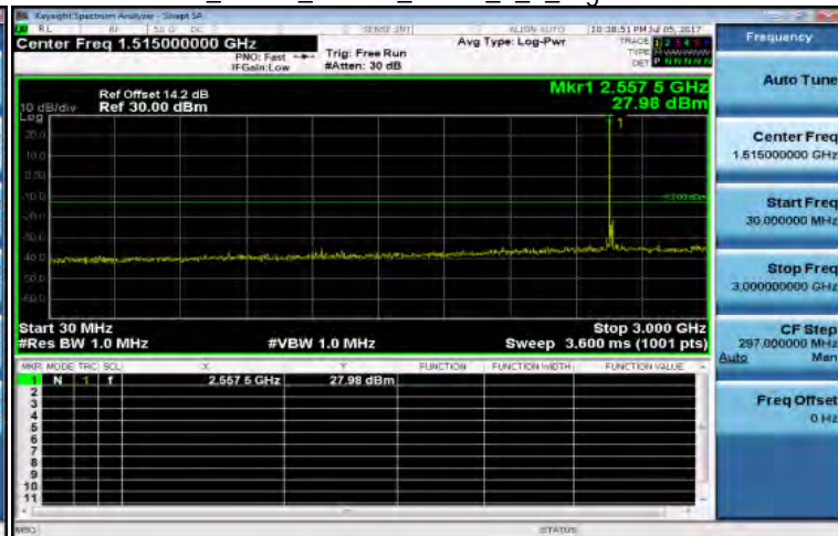
30MHz~3GHz_Band7_15MHz_QPSK_1_0_HighCH21375-2562.5
