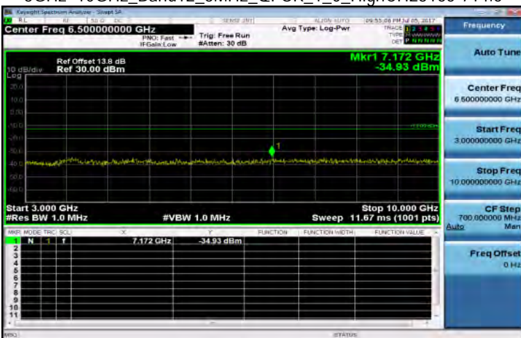
3GHz~10GHz_Band12_3MHz_QPSK_1_0_HighCH23165-714.5
