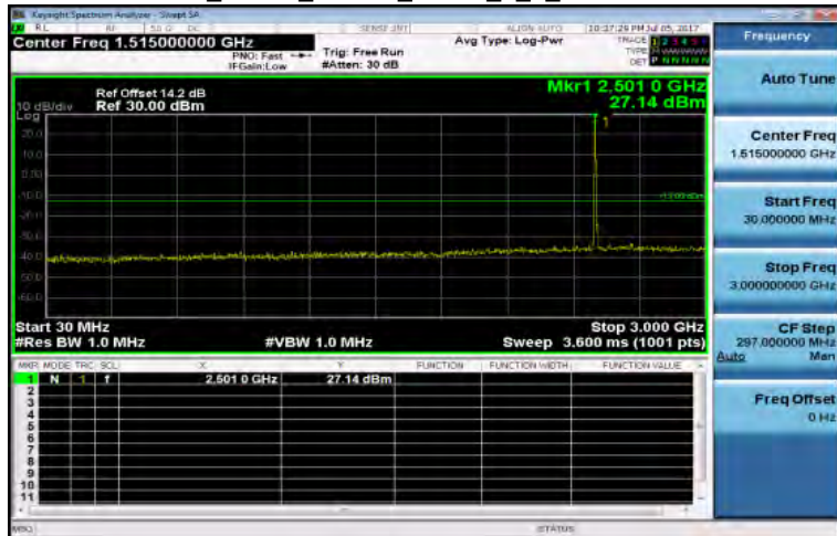
30MHz~3GHz_Band7_15MHz_QPSK_1_0_LowCH20825-2507.5
