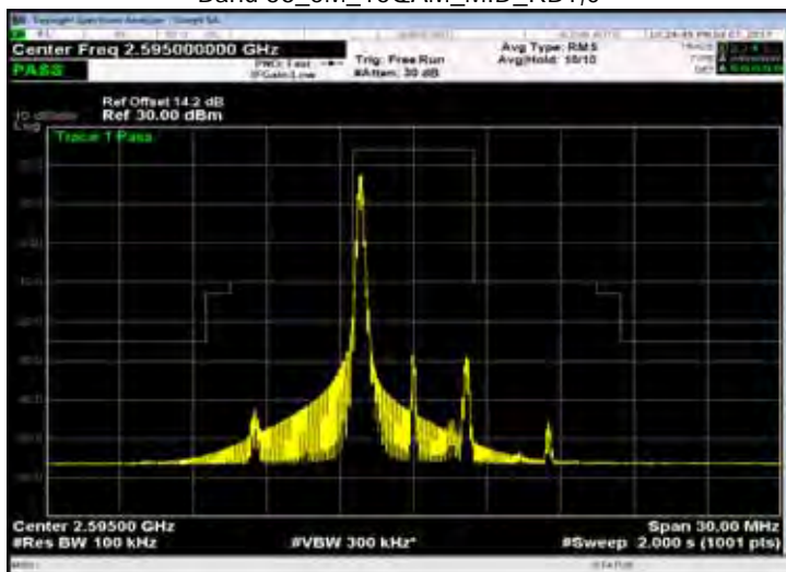
Band 38_5M_16QAM_MID_RB1,24
