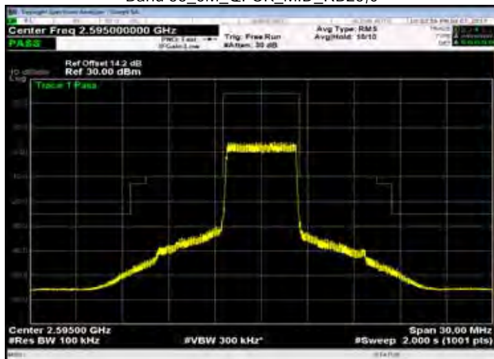
Band 38_5M_QPSK_MID_RB25,0
