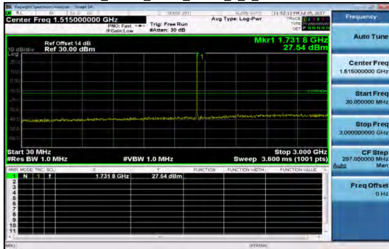
30MHz~3GHz_Band4_3MHz_QPSK_1_0_MidCH20175-1732.5
