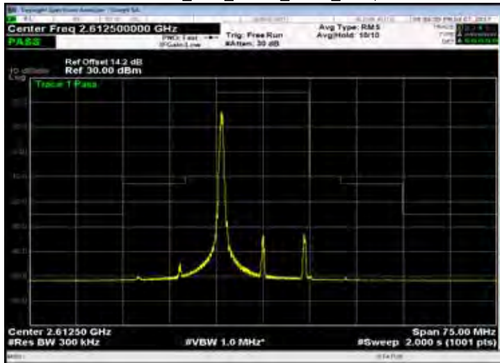
Band 38_15M_QPSK_HIGH_RB1,74
