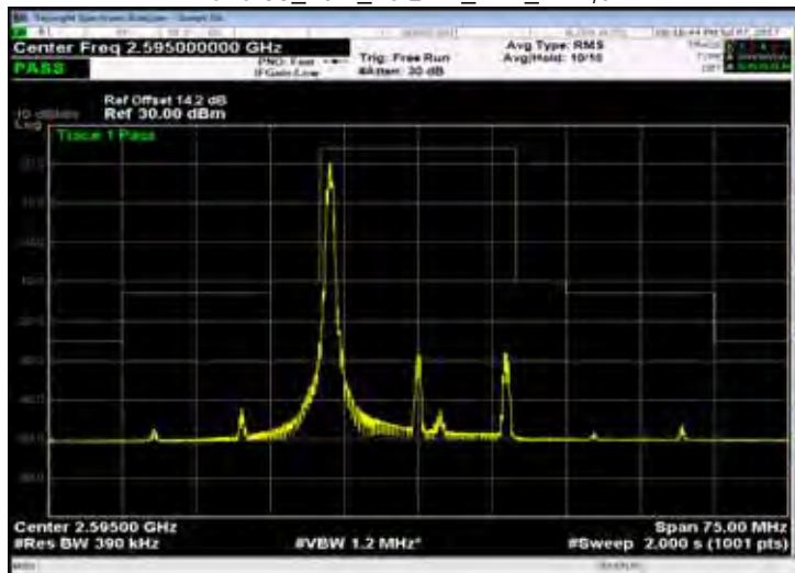
Band 38_20M_16QAM_MID_RB1,99
