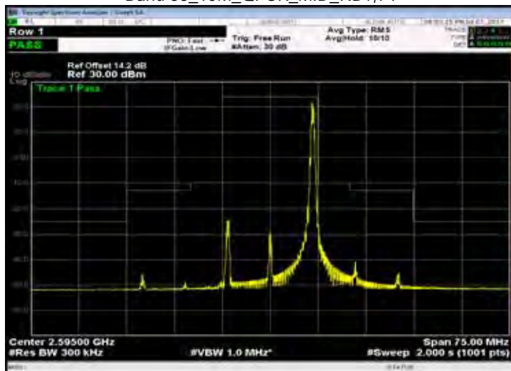
Band 38_15M_QPSK_MID_RB75,0
