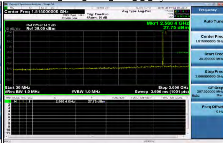
30MHz-3GHz_Band7_10MHz_QPSK_1_0_HighCH21400-2565
