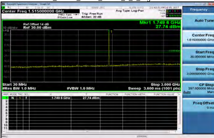
30MHz~3GHz_Band4_5MHz_QPSK_1_0_HighCH20375-1752.5
