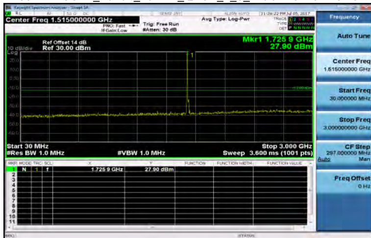
30MHz~3GHz_Band4_15MHz_QPSK_1_0_MidCH20175-1732.5
