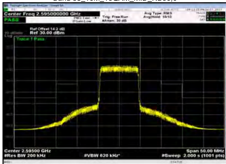
Band 38_10M_16QAM_MID_RB50,0
