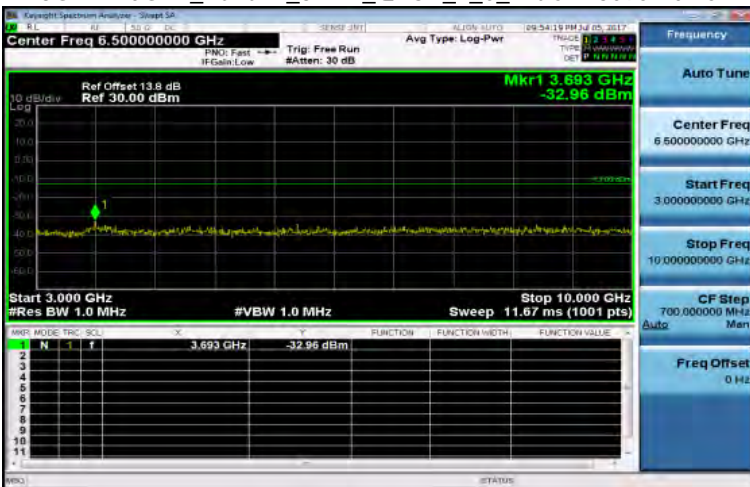
3GHz~10GHz_Band12_3MHz_QPSK_1_0_MidCH23095-707.5
