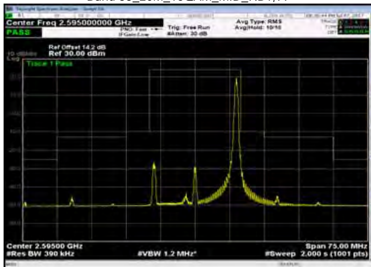
Band 38_20M_16QAM_MID_RB100,0
