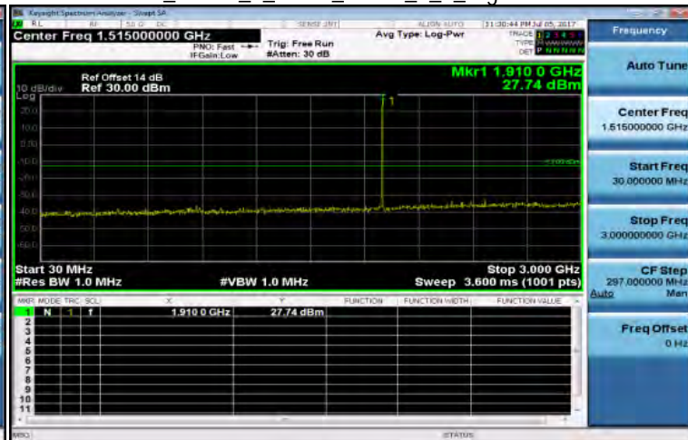
30MHz~3GHz_Band2_1_4MHz_QPSK_1_0_HighCH19193-1909.3
