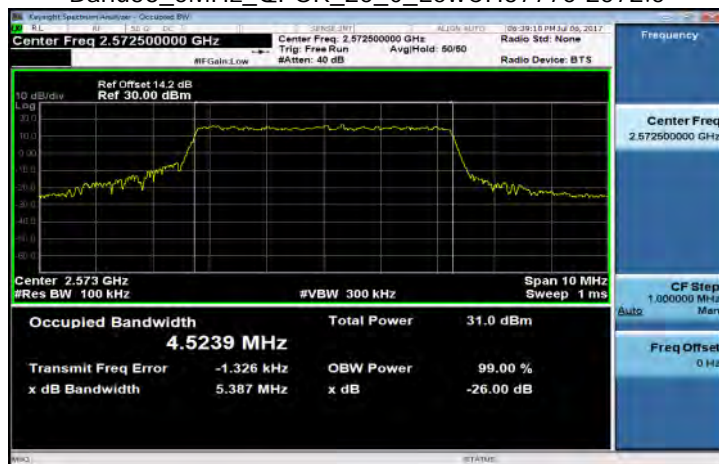
Band38_5MHz_QPSK_25_0_LowCH37775-2572.5
