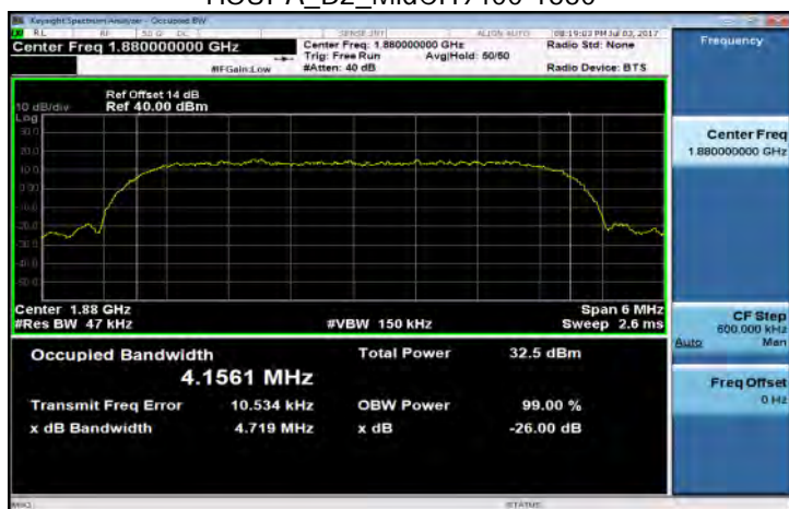
HSUPA_B2_MidCH9400-1880
