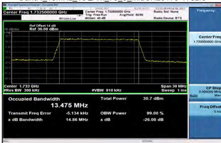
Band4_15MHz_16QAM_75_0_MidCH20175-1732.5
