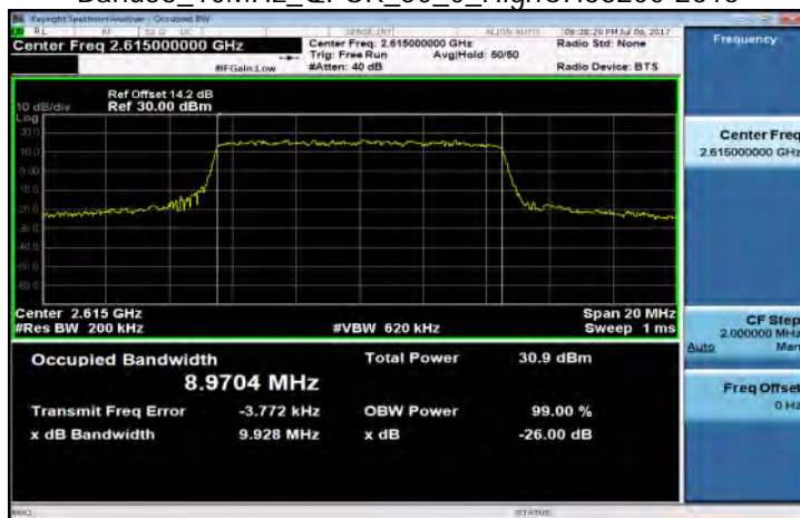
Band38_10MHz_QPSK_50_0_HighCH38200-2615
