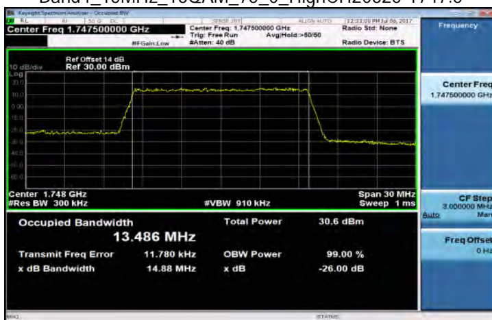
Band4_15MHz_16QAM_75_0_HighCH20325-1747.5
