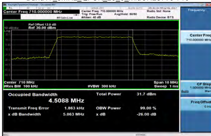
Band17_5MHz_QPSK_25_0_MidCH23790-710
