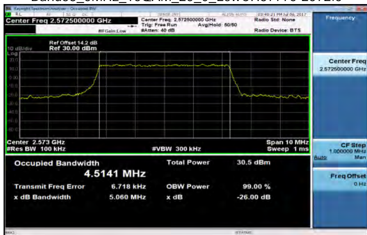
Band38_5MHz_16QAM_25_0_LowCH37775-2572.5
