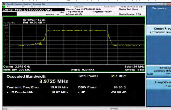
Band38_10MHz_QPSK_50_0_LowCH37800-2575
