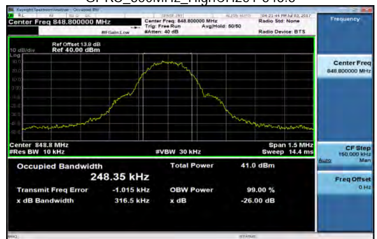
GPRS_850MHz_HighCH251-848.8
