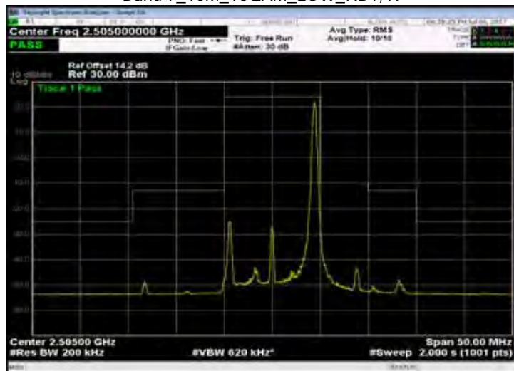
Band 7_10M_16QAM_LOW_RB50,0
