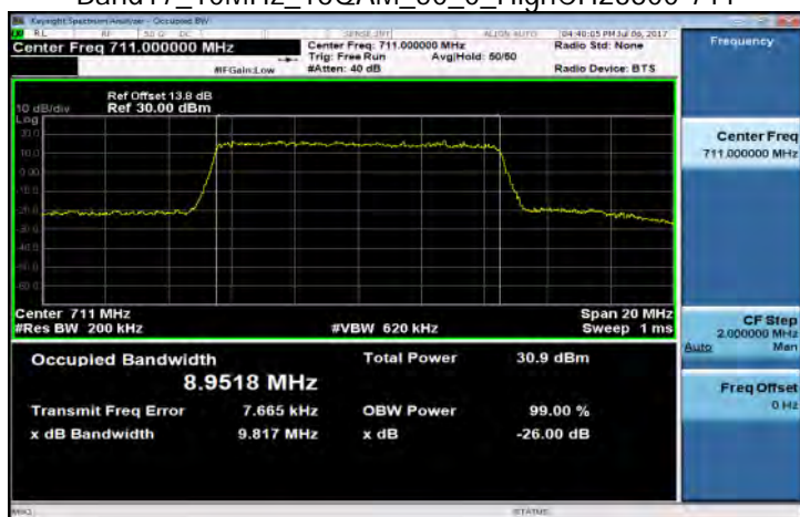
Band17_10MHz_16QAM_50_0_HighCH23800-711
