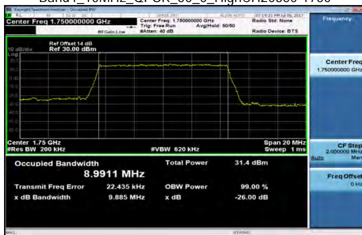
Band4_10MHz_QPSK_50_0_HighCH20350-1750
