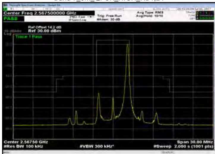
Band 7_5M_QPSK_HIGH_RB25,0
