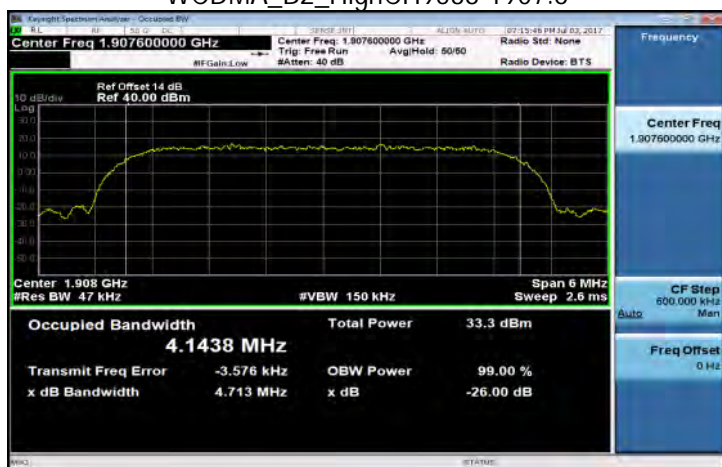
WCDMA_B2_HighCH9538-1907.6
