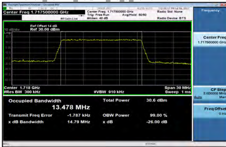
Band4_15MHz_16QAM_75_0_LowCH20025-1717.5
