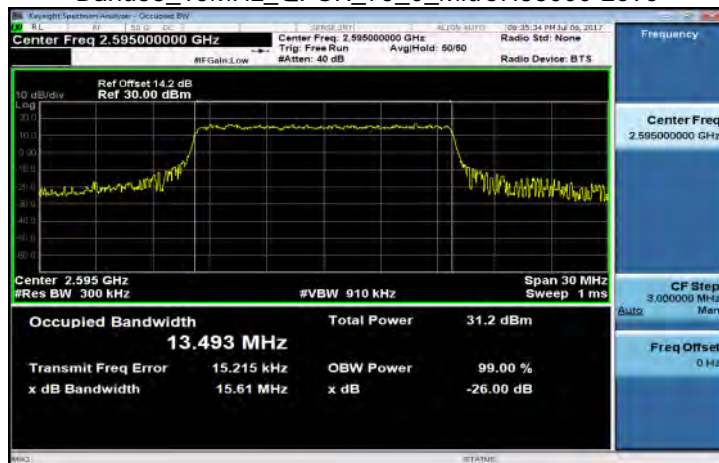
Band38_15MHz_QPSK_75_0_MidCH38000-2595
