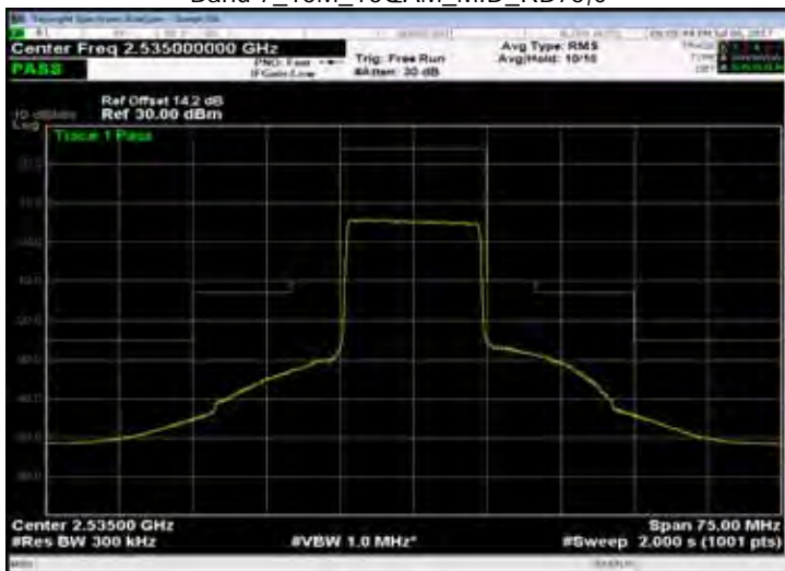
Band 7_15M_16QAM_MID_RB75,0
