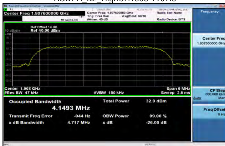
HSDPA_B2_HighCH9538-1907.6
