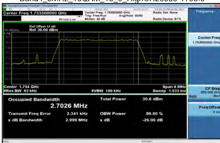
Band4_3MHz_16QAM_15_0_HighCH20385-1753.5
