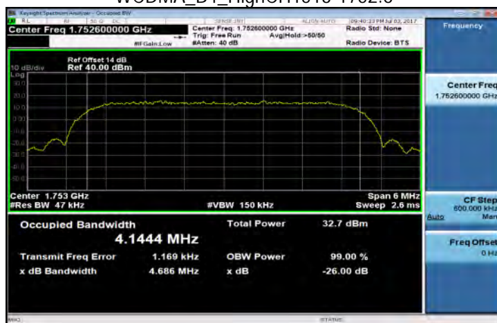
WCDMA_B4_HighCH1513-1752.6
