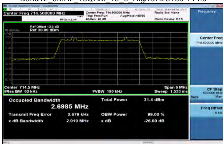
Band12_3MHz_16QAM_15_0_HighCH23165-714.5
