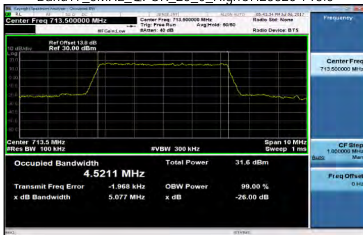
Band17_5MHz_QPSK_25_0_HighCH23825-713.5
