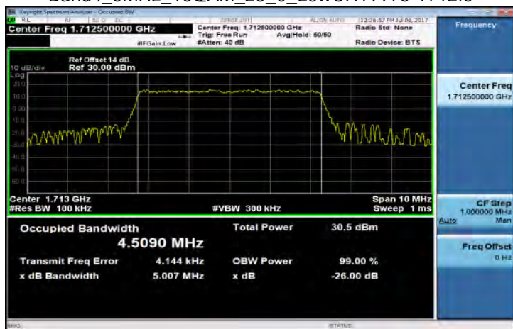
Band4_5MHz_16QAM_25_0_LowCH19975-1712.5
