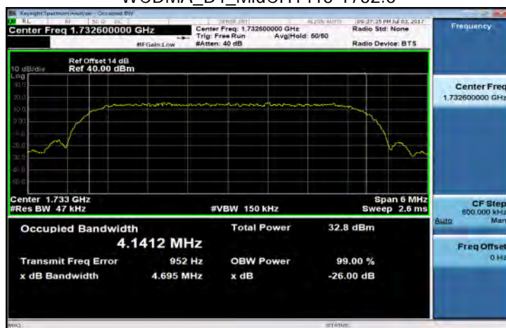
WCDMA_B4_MidCH1413-1732.6
