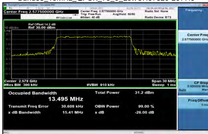
Band38_15MHz_QPSK_75_0_LowCH37825-2577.5
