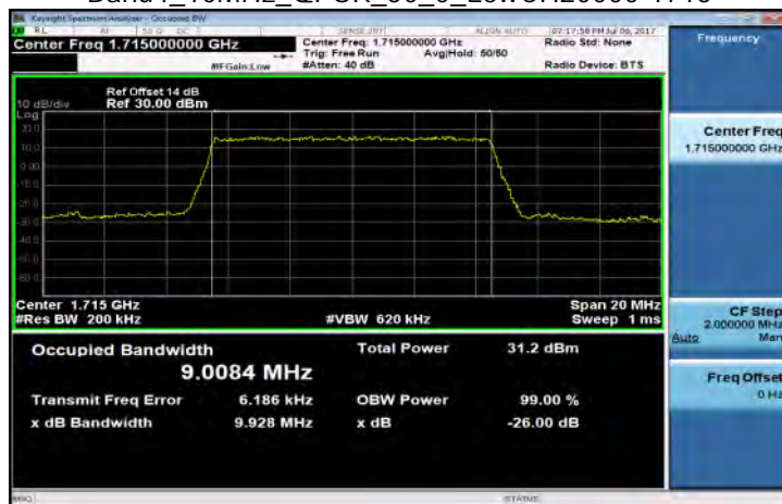
Band4_10MHz_QPSK_50_0_LowCH20000-1715
