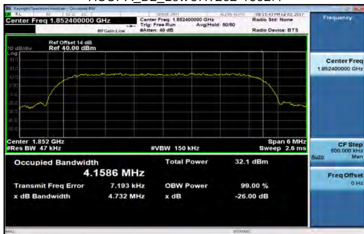
HSUPA_B2_LowCH9262-1852.4
