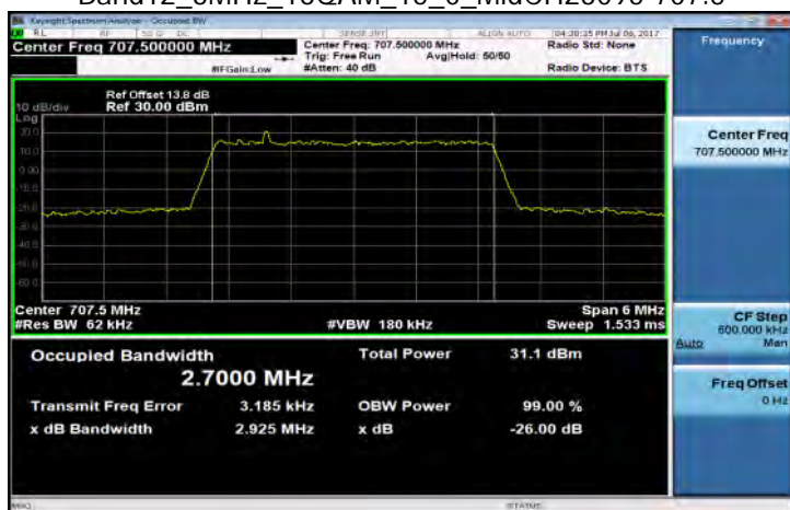
Band12_3MHz_16QAM_15_0_MidCH23095-707.5
