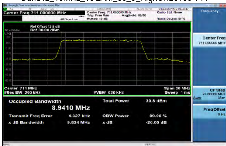
Band12_10MHz_16QAM_50_0_HighCH23130-711
