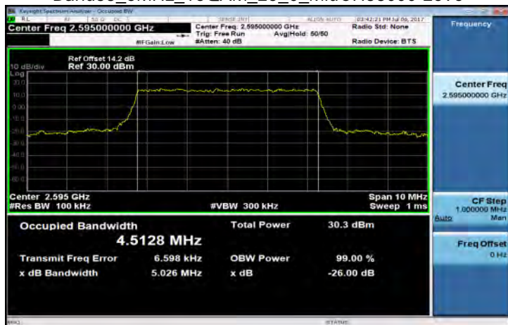
Band38_5MHz_16QAM_25_0_MidCH38000-2595
