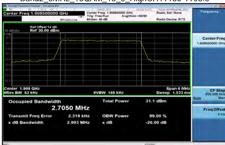
Band2_3MHz_16QAM_15_0_HighCH19185-1908.5
