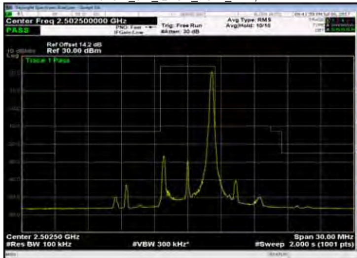
Band 7_5M_QPSK_LOW_RB25,0
