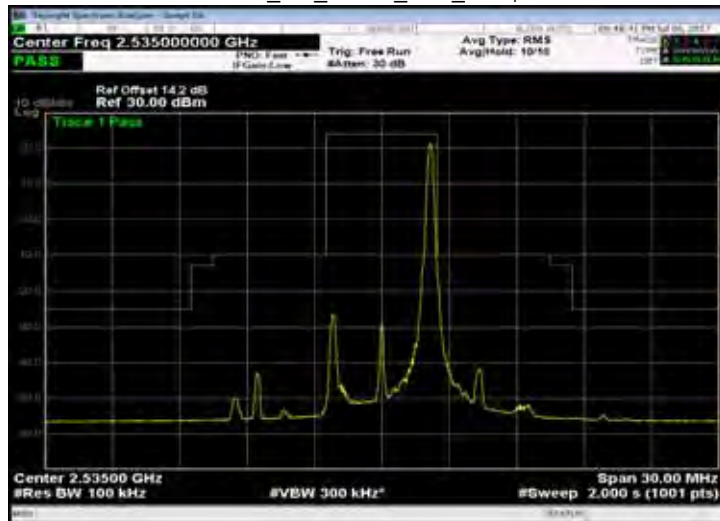
Band 7_5M_QPSK_MID_RB25,0
