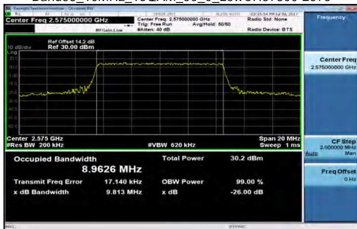
Band38_10MHz_16QAM_50_0_LowCH37800-2575
