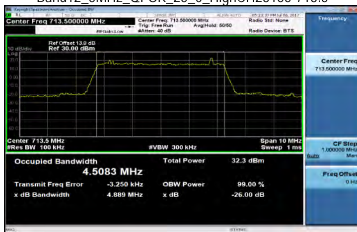
Band12_5MHz_QPSK_25_0_HighCH23155-713.5
