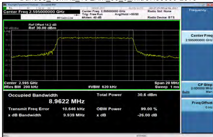
Band38_10MHz_16QAM_50_0_MidCH38000-2595
