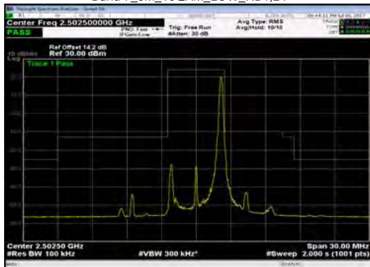
Band 7_5M_16QAM_LOW_RB25,0
