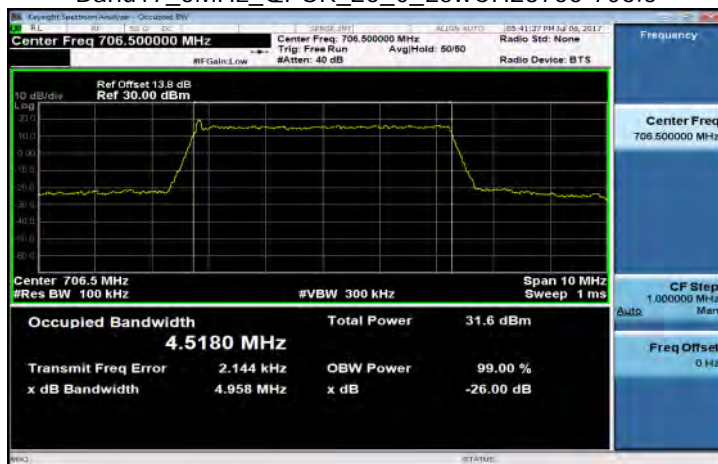
Band17_5MHz_QPSK_25_0_LowCH23755-706.5
