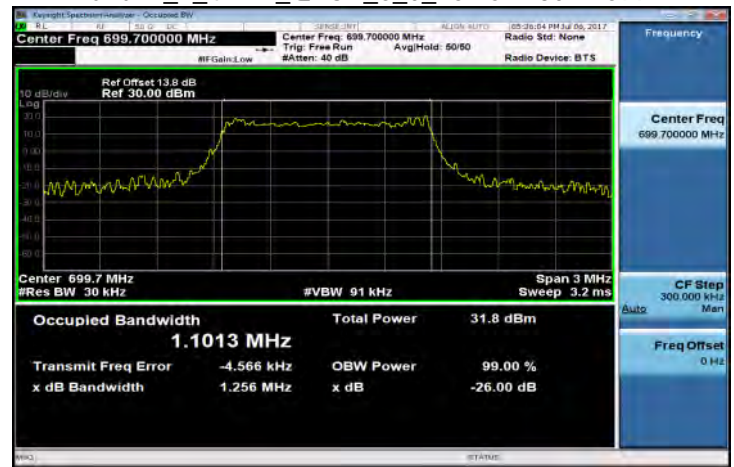
Band12_1_4MHz_QPSK_6_0_LowCH23017-699.7
