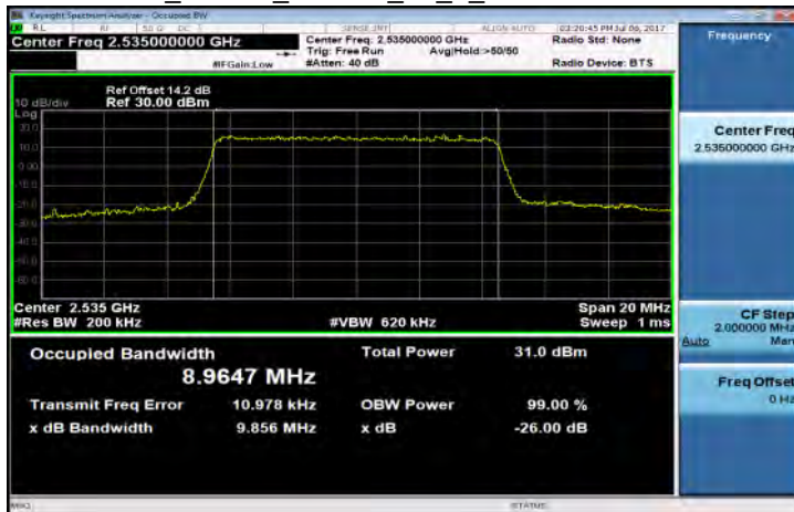
Band7_10MHz_16QAM_50_0_MidCH21100-2535
