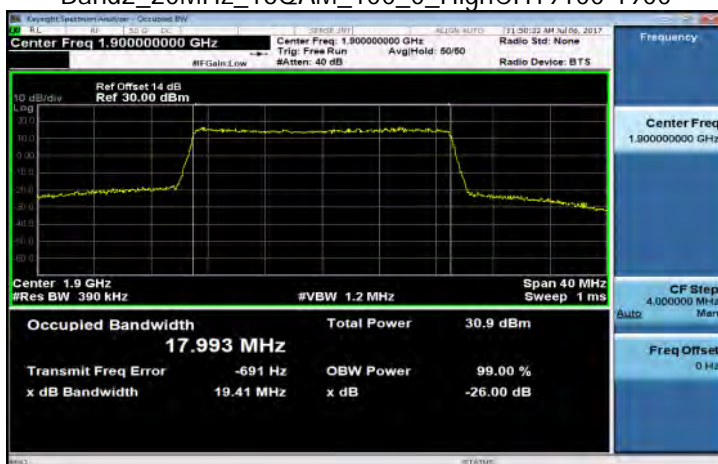
Band2_20MHz_16QAM_100_0_HighCH19100-1900
