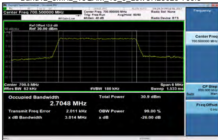
Band12_3MHz_16QAM_15_0_LowCH23025-700.5
