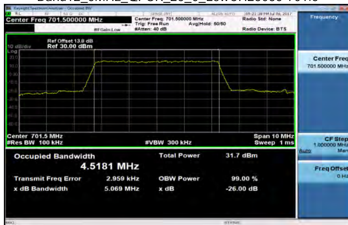
Band12_5MHz_QPSK_25_0_LowCH23035-701.5
