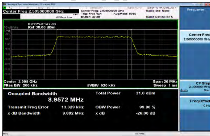
Band7_10MHz_16QAM_50_0_LowCH20800-2505
