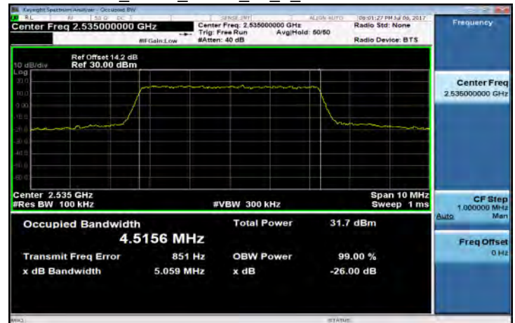
Band7_5MHz_QPSK_25_0_MidCH21100-2535
