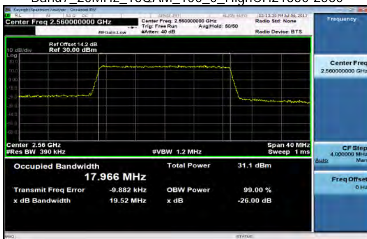
Band7_20MHz_16QAM_100_0_HighCH21350-2560
