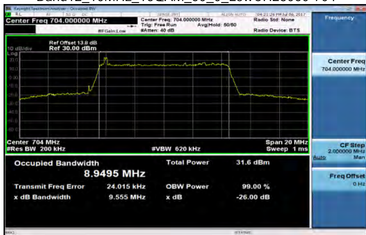
Band12_10MHz_16QAM_50_0_LowCH23060-704
