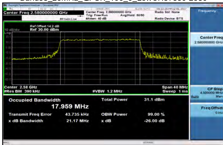
Band38_20MHz_QPSK_100_0_LowCH37850-2580
