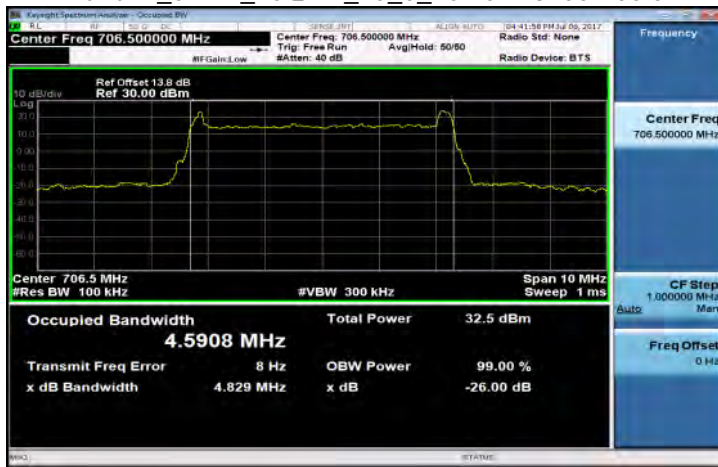
Band17_5MHz_16QAM_25_0_LowCH23755-706.5
