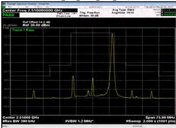
Band 7_20M_QPSK_LOW_RB100,0
