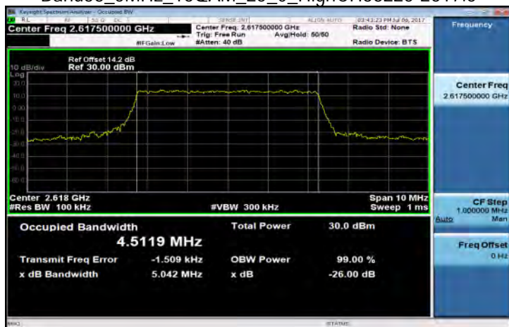
Band38_5MHz_16QAM_25_0_HighCH38225-2617.5
