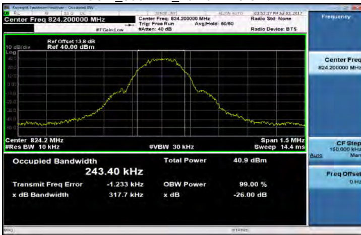
GSM_850MHz_LowCH128-824.2
