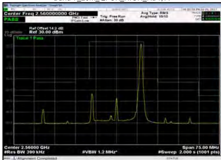
Band 7_20M_QPSK_HIGH_RB100,0
