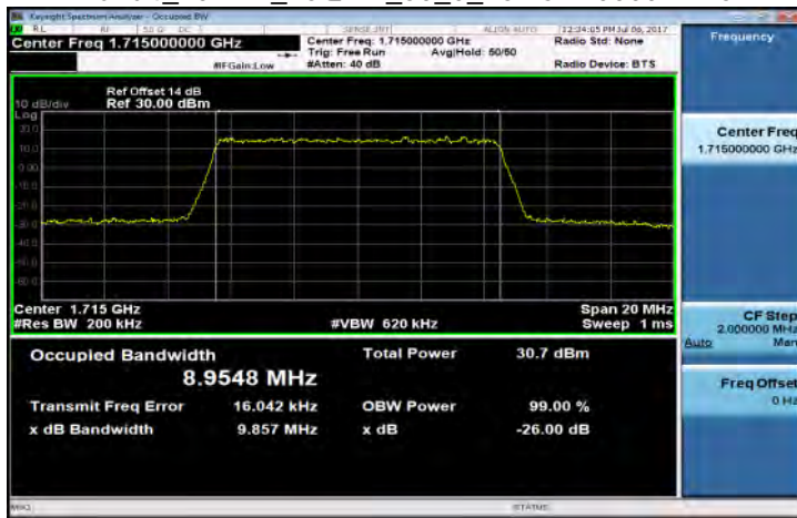
Band4_10MHz_16QAM_50_0_LowCH20000-1715
