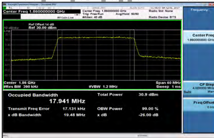
Band2_20MHz_16QAM_100_0_LowCH18700-1860
