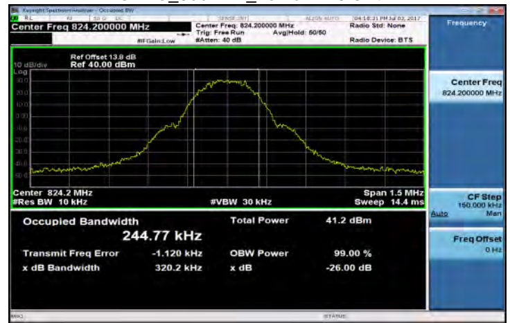
GPRS_850MHz_LowCH128-824.2
