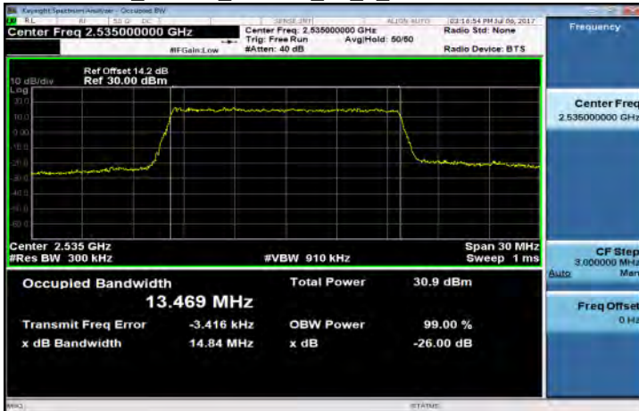
Band7_15MHz_16QAM_75_0_MidCH21100-2535
