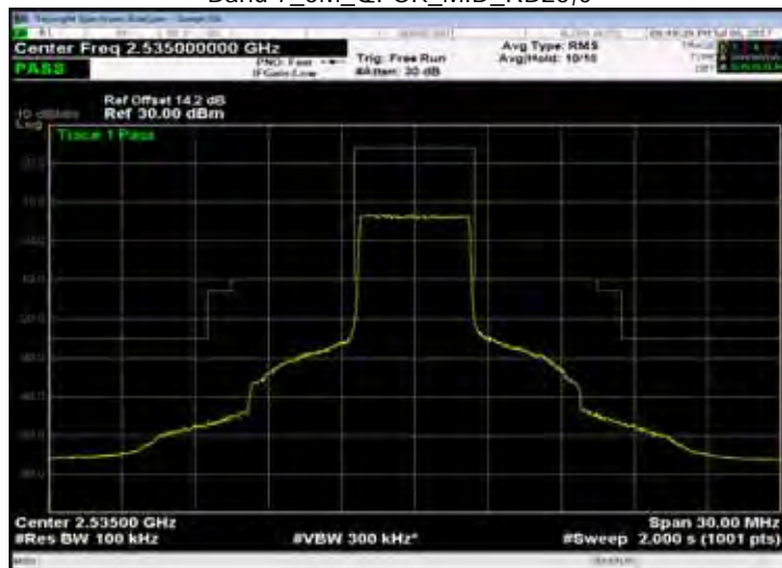
Band 7_5M_QPSK_MID_RB25,0
