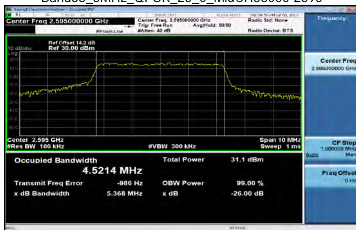
Band38_5MHz_QPSK_25_0_MidCH38000-2595
