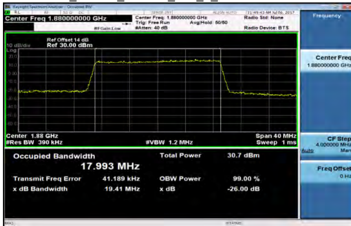
Band2_20MHz_16QAM_100_0_MidCH18900-1880
