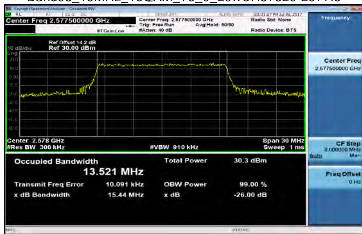
Band38_15MHz_16QAM_75_0_LowCH37825-2577.5
