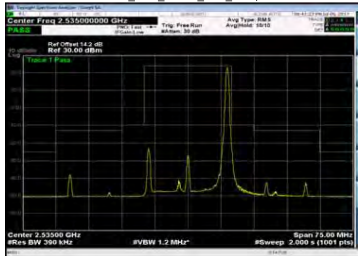
Band 7_20M_QPSK_MID_RB100,0
