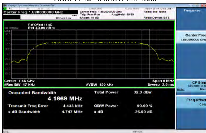
HSDPA_B2_MidCH9400-1880
