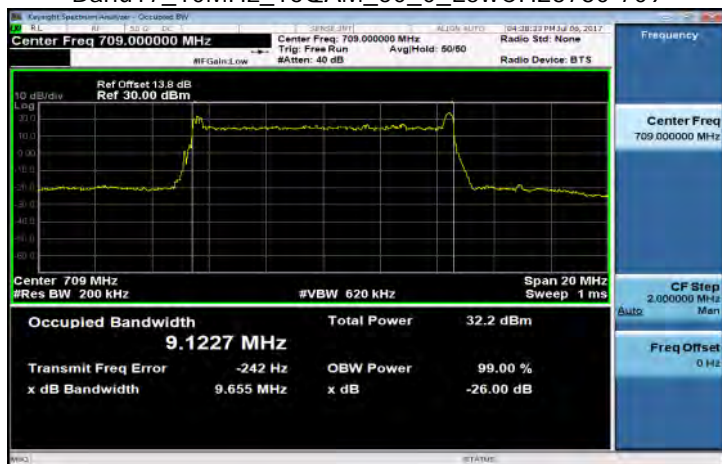
Band17_10MHz_16QAM_50_0_LowCH23780-709
