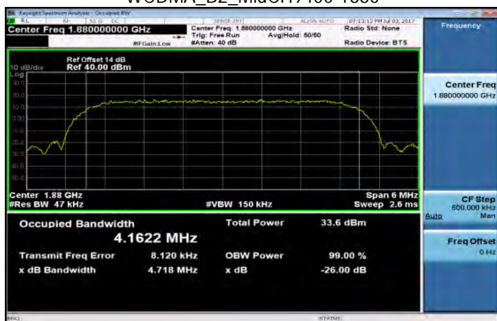
WCDMA_B2_MidCH9400-1880
