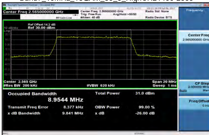
Band7_10MHz_16QAM_50_0_HighCH21400-2565
