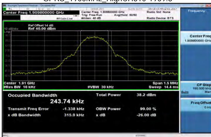
GPRS_1900MHz_HighCH810-1909.8
