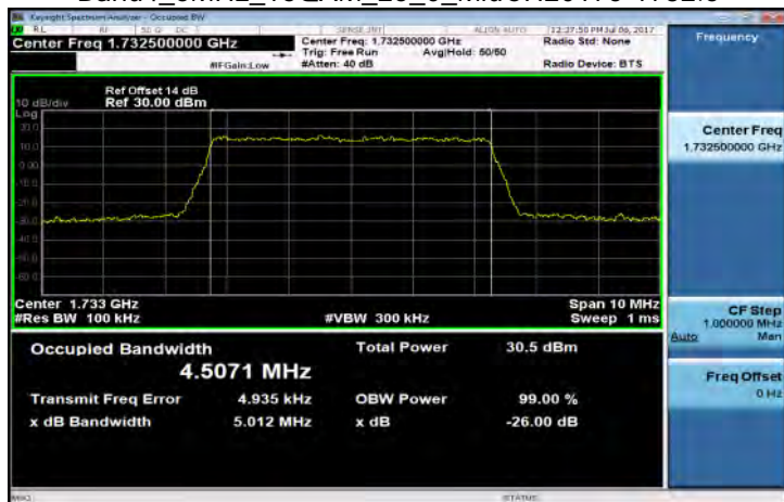
Band4_5MHz_16QAM_25_0_MidCH20175-1732.5
