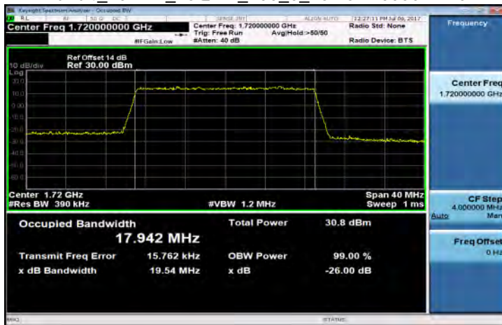
Band4_20MHz_16QAM_100_0_LowCH20050-1720
