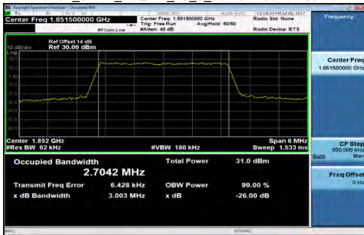
Band2_3MHz_16QAM_15_0_LowCH18615-1851.5
