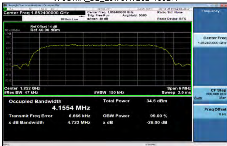
WCDMA_B2_LowCH9262-1852.4
