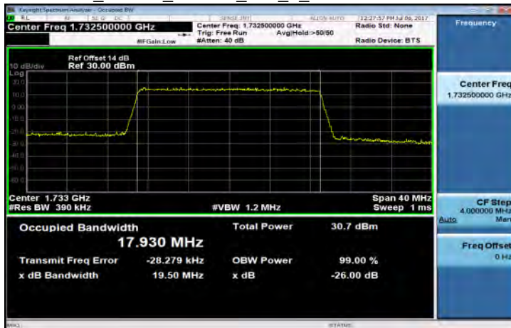
Band4_20MHz_16QAM_100_0_MidCH20175-1732.5
