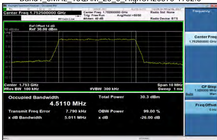
Band4_5MHz_16QAM_25_0_HighCH20375-1752.5
