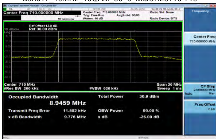
Band17_10MHz_16QAM_50_0_MidCH23790-710
