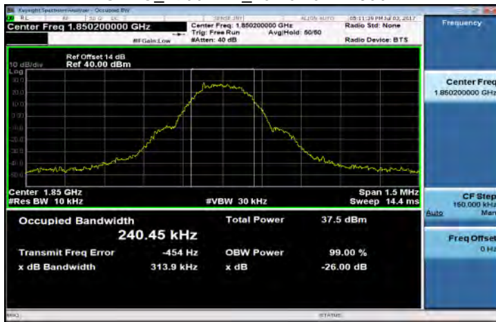
GPRS_1900MHz_LowCH512-1850.2
