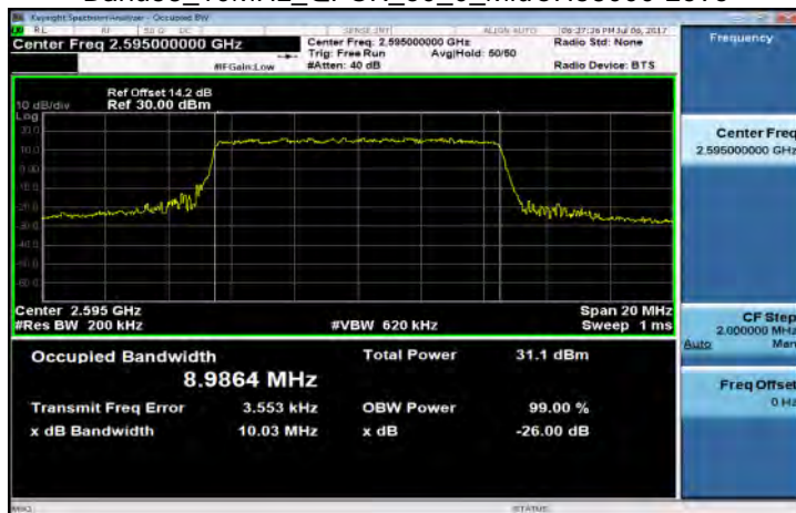
Band38_10MHz_QPSK_50_0_MidCH38000-2595
