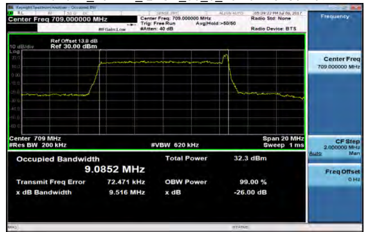
Band17_10MHz_QPSK_50_0_LowCH23780-709
