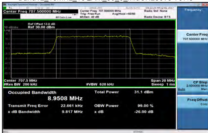
Band12_10MHz_16QAM_50_0_MidCH23095-707.5
