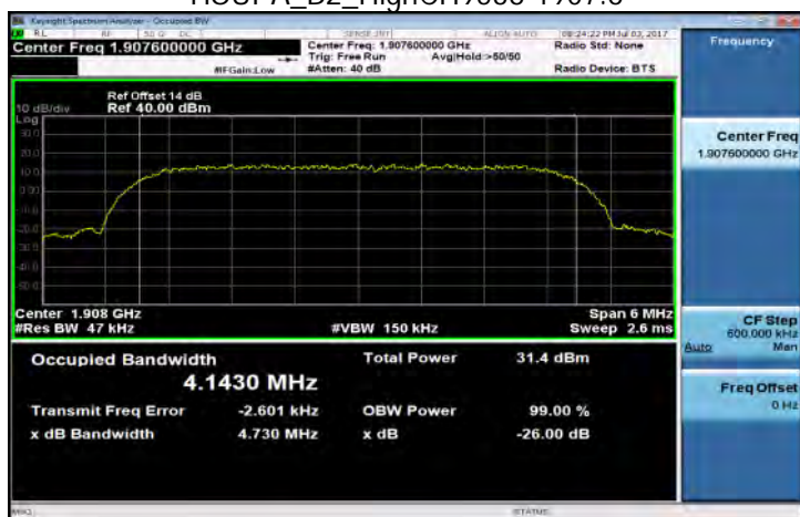
HSUPA_B2_HighCH9538-1907.6
