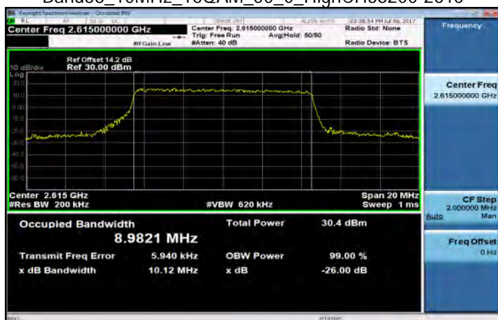
Band38_10MHz_16QAM_50_0_HighCH38200-2615
