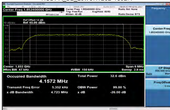
HSDPA_B2_LowCH9262-1852.4
