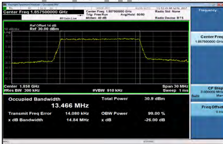
Band2_15MHz_16QAM_75_0_LowCH18675-1857.5
