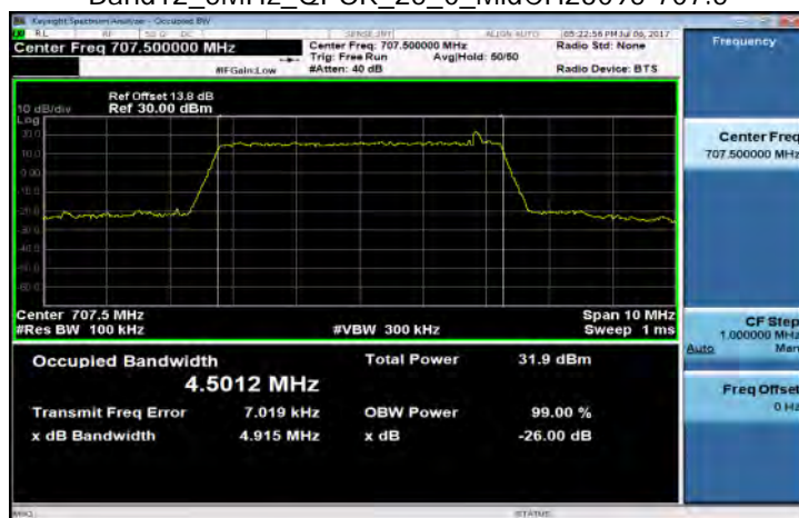
Band12_5MHz_QPSK_25_0_MidCH23095-707.5
