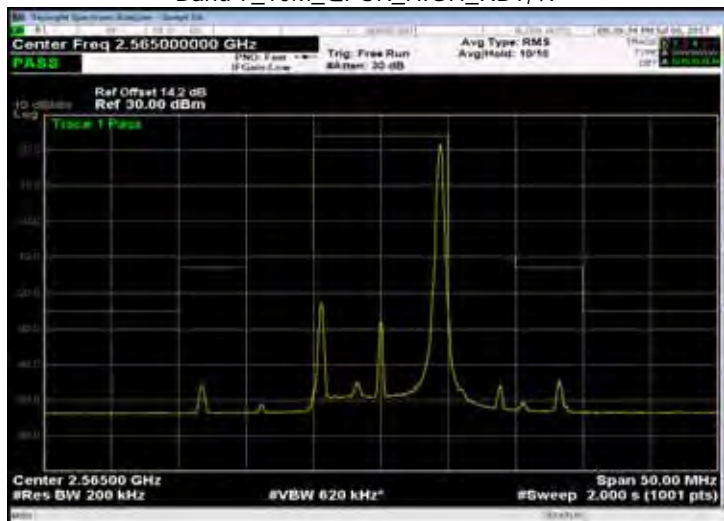
Band 7_10M_QPSK_HIGH_RB50,0
