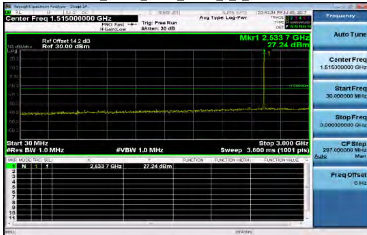
30MHz~3GHz_Band7_5MHz_QPSK_1_0_MidCH21100-2535
