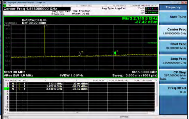
30MHz~3GHz_Band17_5MHz_QPSK_1_0_HighCH23825-713.5
