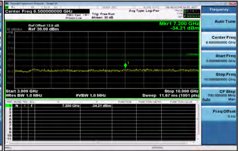
3GHz~10GHz_Band12_10MHz_QPSK_1_0_MidCH23095-707.5
