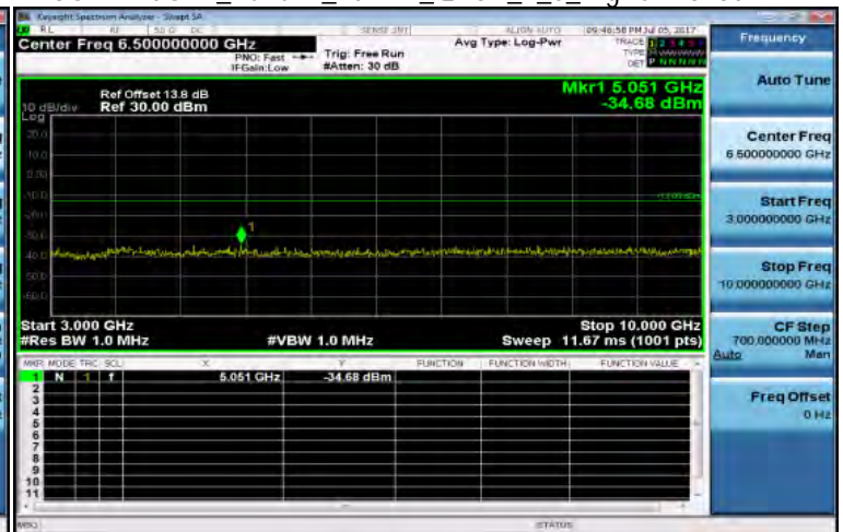
3GHz~10GHz_Band12_10MHz_QPSK_1_0_HighCH23130-711
