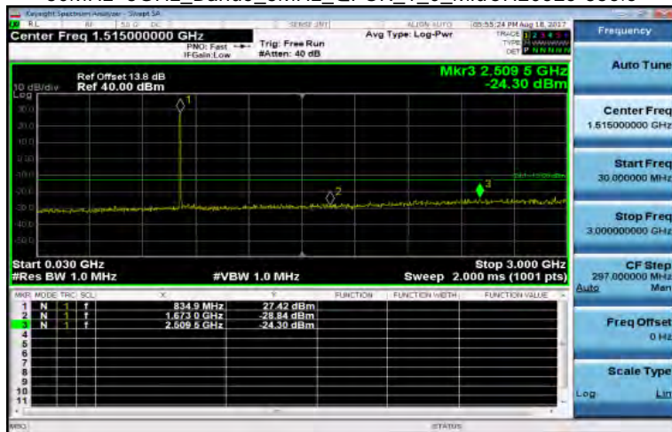
30MHz~3GHz_Band5_3MHz_QPSK_1_0_MidCH20525-836.5
