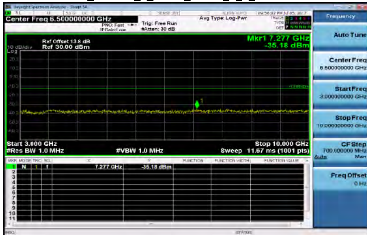
3GHz~10GHz_Band12_1_4MHz_QPSK_1_0_LowCH23017-699.7
