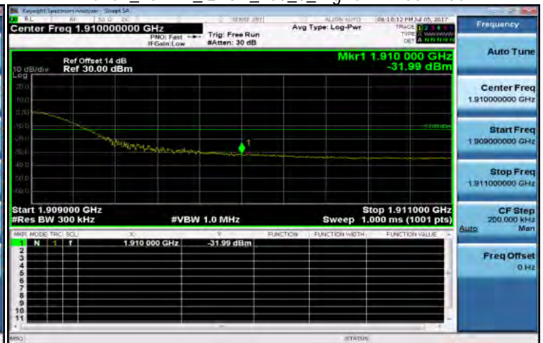
Band2_20MHz_QPSK_100_0_HighCH19100-1900
