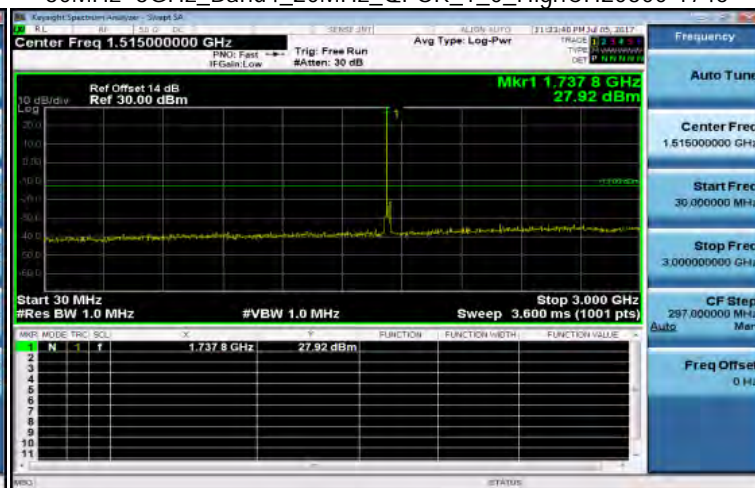
30MHz~3GHz_Band4_20MHz_QPSK_1_0_HighCH20300-1745
