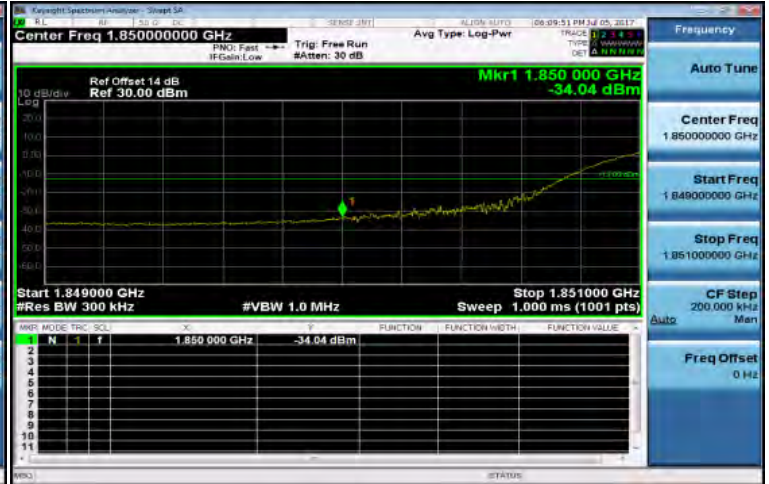
Band2_20MHz_QPSK_100_0_LowCH18700-1860
