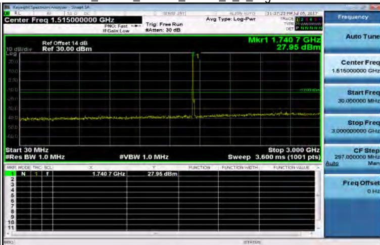
30MHz~3GHz_Band4_15MHz_QPSK_1_0_HighCH20325-1747.5
