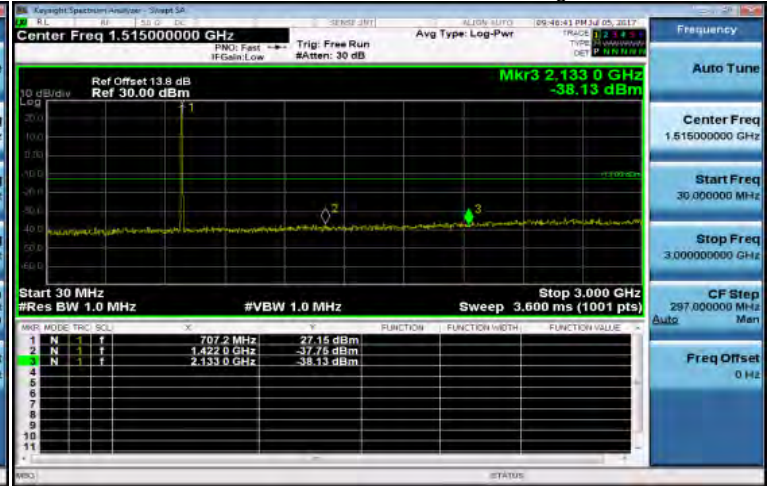
30MHz~3GHz_Band12_10MHz_QPSK_1_0_HighCH23130-711
