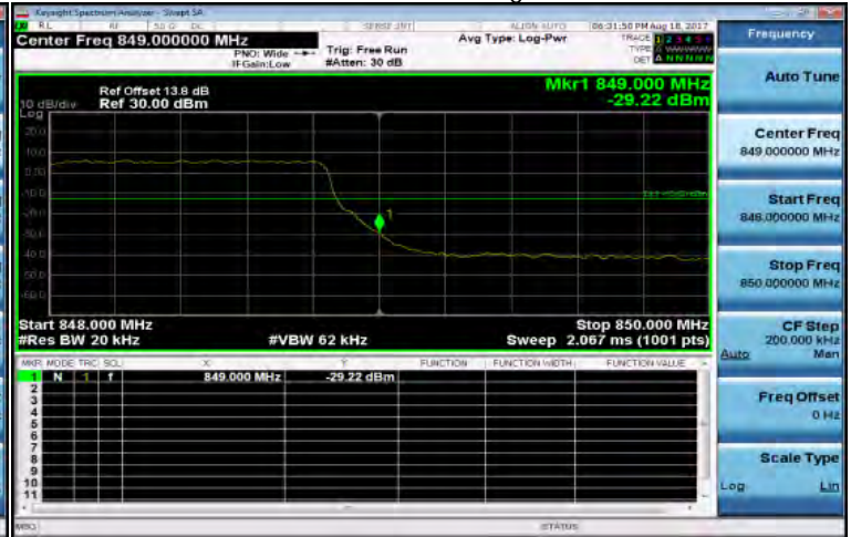
Band5_1_4MHz_QPSK_6_0_HighCH20643-848.3
