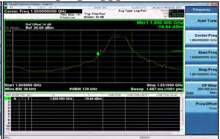
Band2_3MHz_QPSK_1_0_LowCH18615-1851.5
