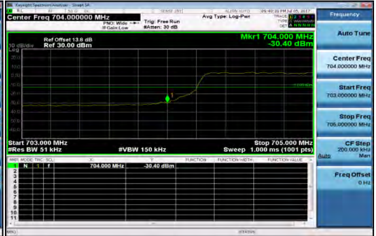
Band17_5MHz_QPSK_25_0_LowCH23755-706.5
