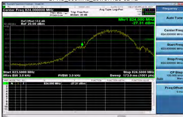
GPRS_850MHz_LowCH128-824.2
