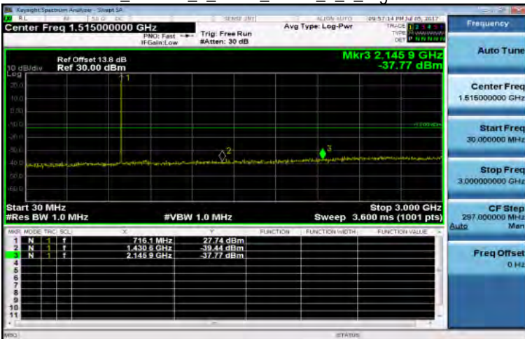
30MHz~3GHz_Band12_1_4MHz_QPSK_1_0_HighCH23173-715.3
