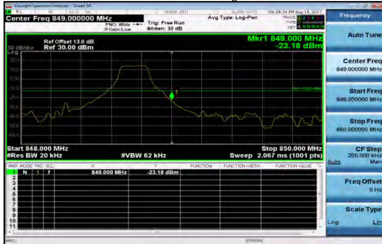
Band5_1_4MHz_QPSK_1_5_HighCH20643-848.3
