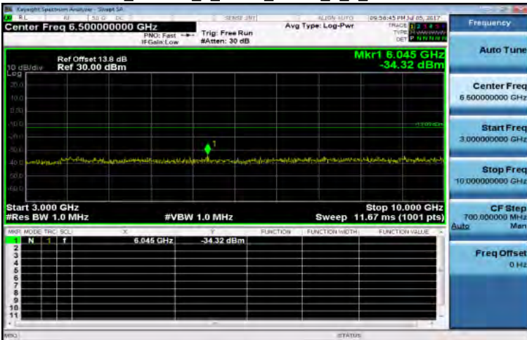
3GHz~10GHz_Band12_1_4MHz_QPSK_1_0_MidCH23095-707.5
