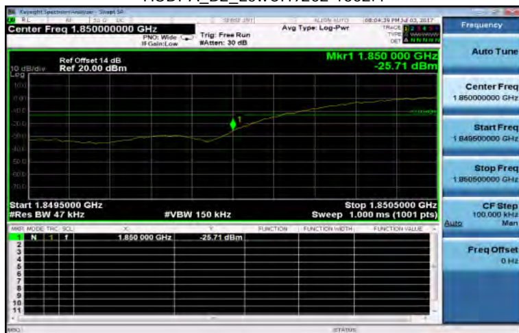
HSDPA_B2_LowCH9262-1852.4
