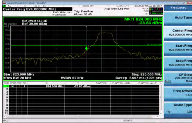
Band5_1_4MHz_QPSK_1_0_LowCH20407-824.7
