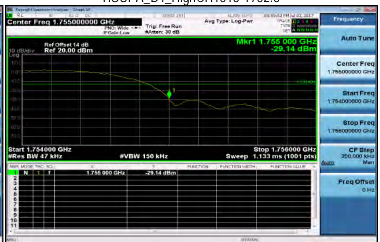
HSUPA_B4_HighCH1513-1752.6
