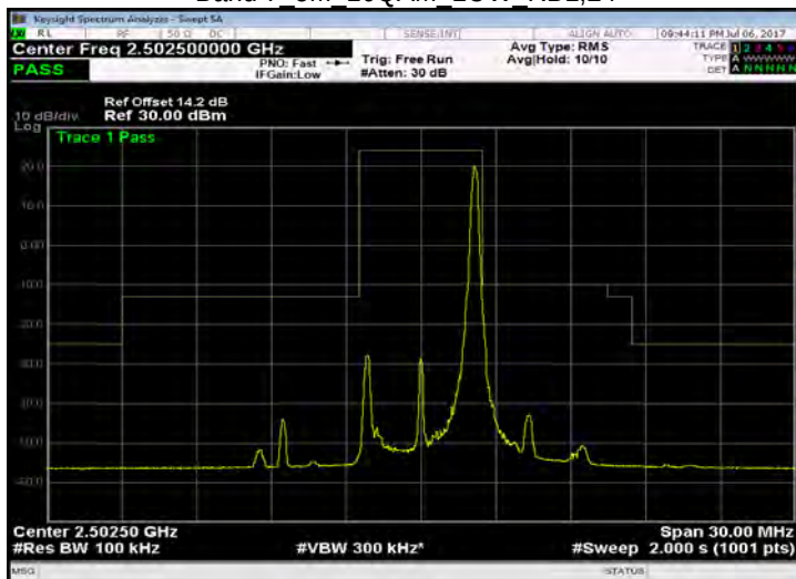
Band 7 5M 16QAM LOW RB25,0
