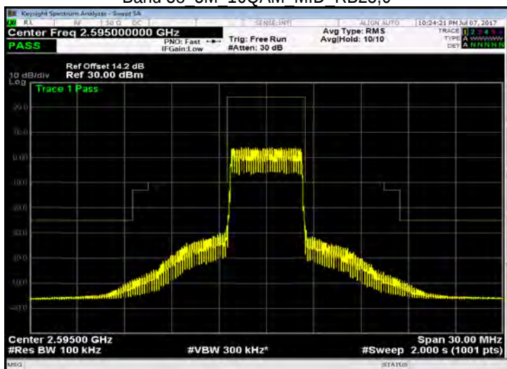
Band 38 5M 16QAM MID RB25,0
