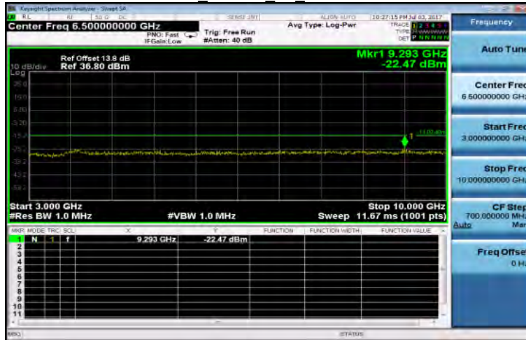
3GHz~10GHz HSUPA B5 LowCH4132-826.4
