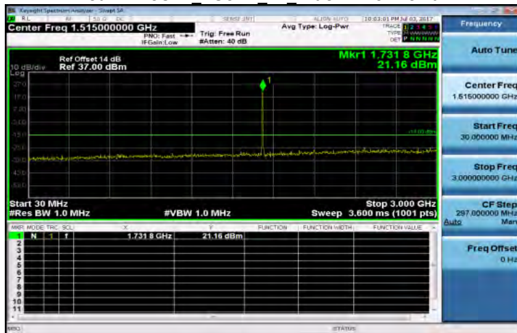
30MHz~3GHz HSUPA B4 MidCH1413-1732.6
