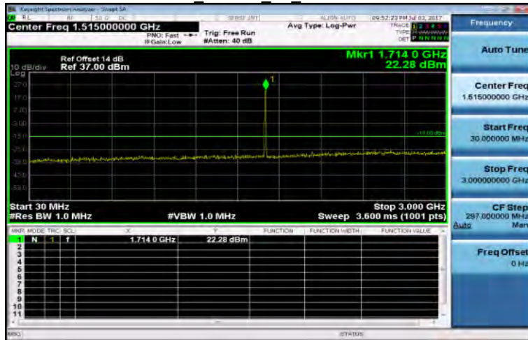
30MHz~3GHz HSDPA B4 LowCH1312-1712.4
