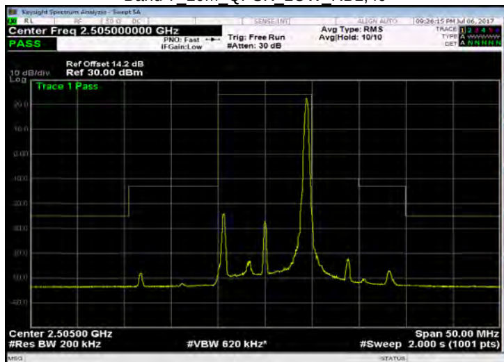
Band 7 10M QPSK LOW RB50,0
