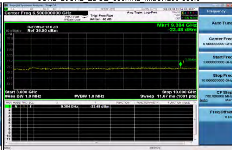
3GHz~10GHz EDGE 850MHz MidCH190-836.6
