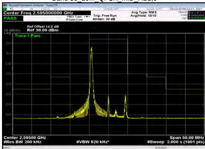
Band 38 10M QPSK MID RB1,49
