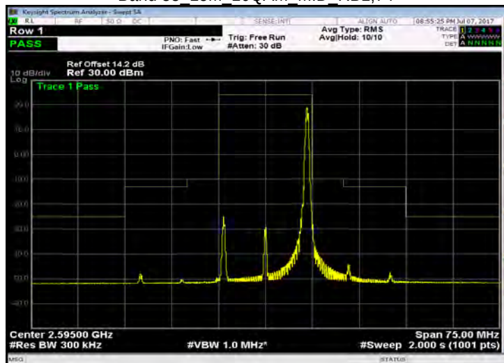
Band 38 15M 16QAM MID RB75,0
