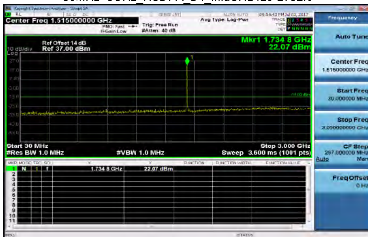
30MHz~3GHz HSDPA B4 MidCH1413-1732.6
