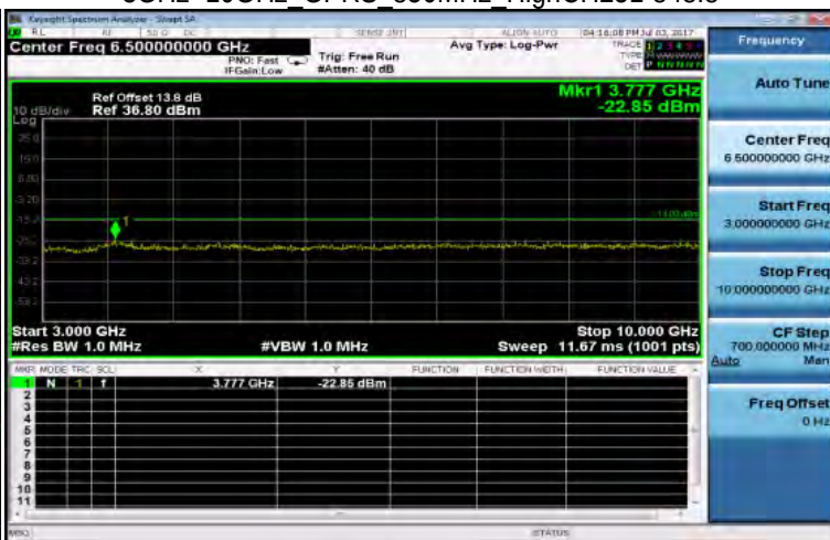
3GHz~10GHz GPRS 850MHz HighCH251-848.8
