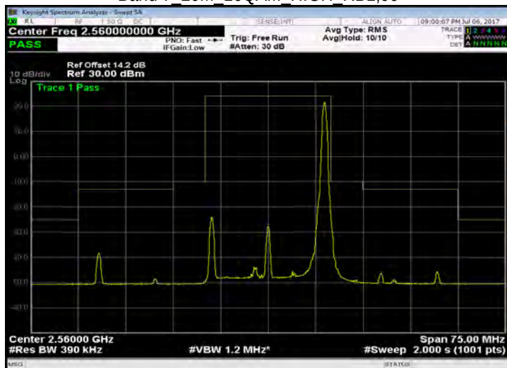
Band 7 20M 16QAM HIGH RB100,0
