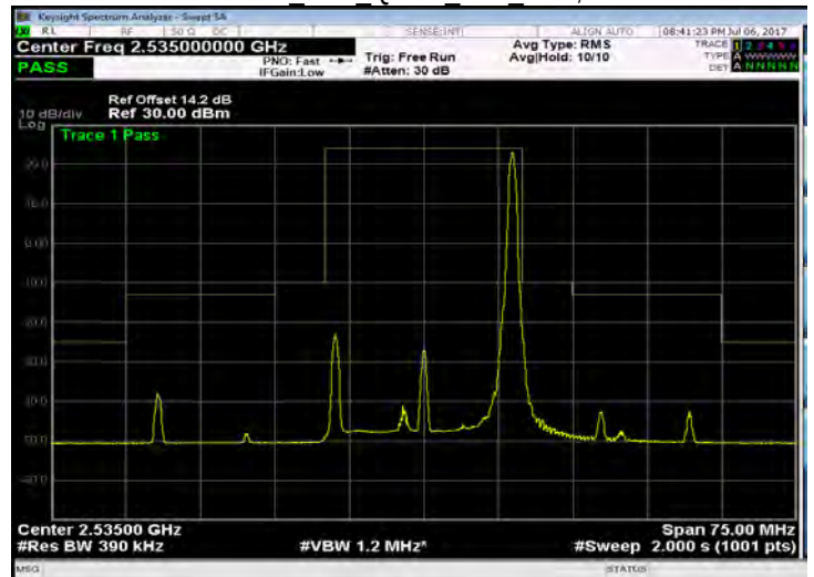
Band 7 20M QPSK MID RB100,0
