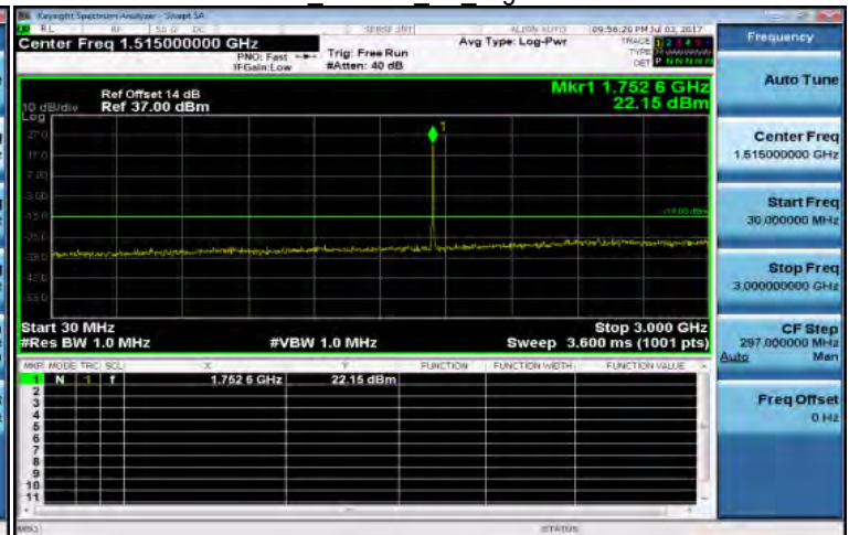
30MHz~3GHz HSDPA B4 HighCH1513-1752.6
