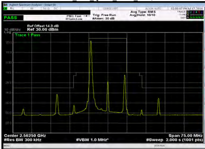
Band 7 15M QPSK HIGH RB1,74
