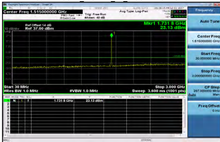
30MHz~3GHz WCDMA B4 MidCH1413-1732.6
