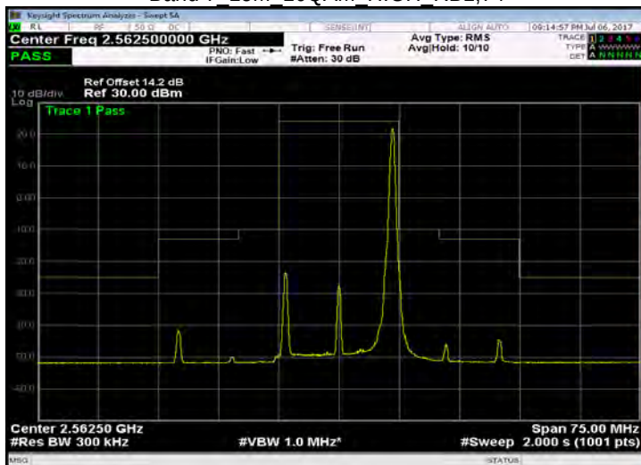
Band 7 15M 16QAM HIGH RB75,0
