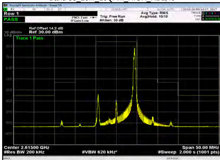
Band 38 10M 16QAM HIGH RB50,0
