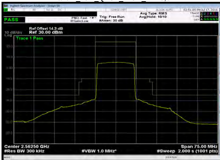
Band 7 15M QPSK HIGH RB75,0
