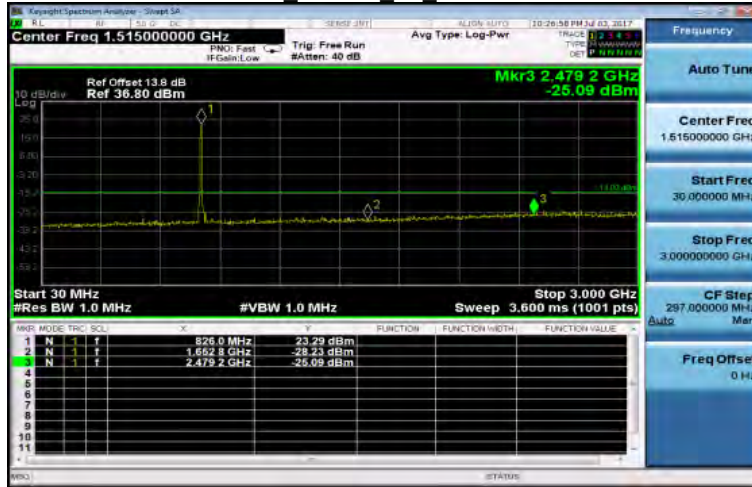
30MHz~3GHz HSUPA B5 LowCH4132-826.4
