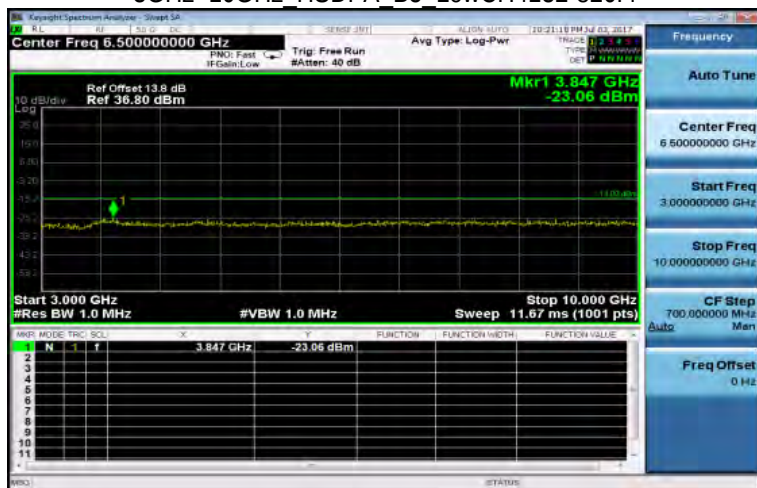
3GHz~10GHz HSDPA B5 LowCH4132-826.4
