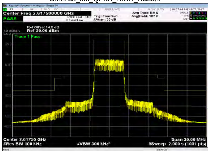
Band 38 5M QPSK HIGH RB25,0
