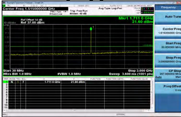
30MHz~3GHz HSUPA B4 LowCH1312-1712.4
