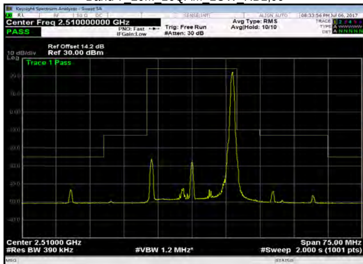
Band 7 20M 16QAM LOW RB100,0
