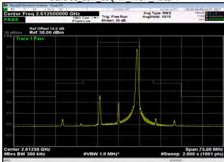
Band 38 15M 16QAM HIGH RB75,0
