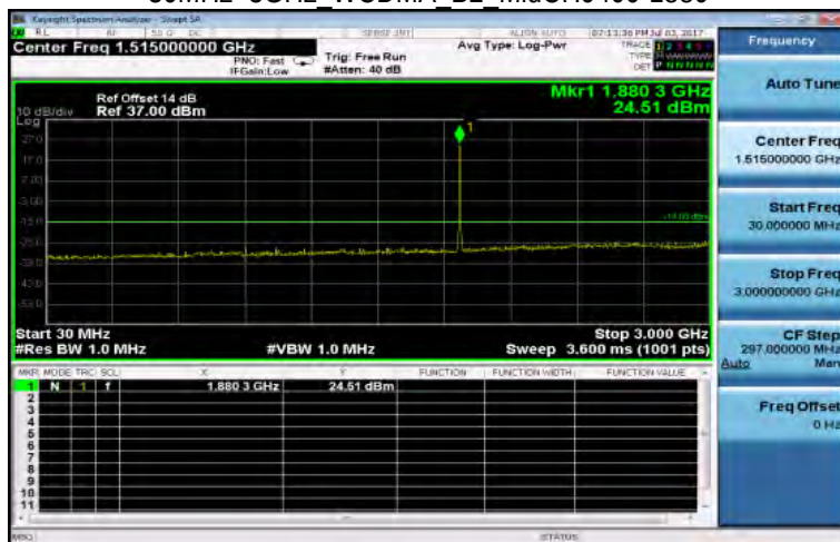
30MHz~3GHz WCDMA B2 MidCH9400-1880
