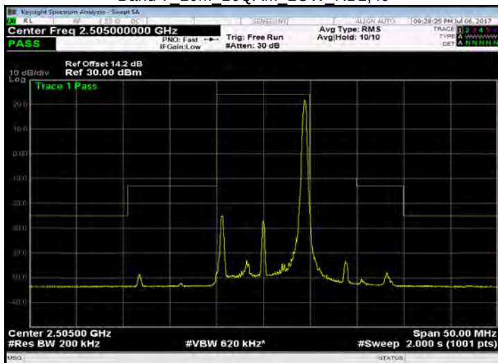
Band 7 10M 16QAM LOW RB50,0
