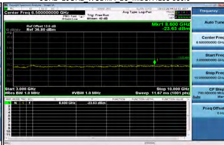
3GHz~10GHz WCDMA B5 MidCH4183-836.6
