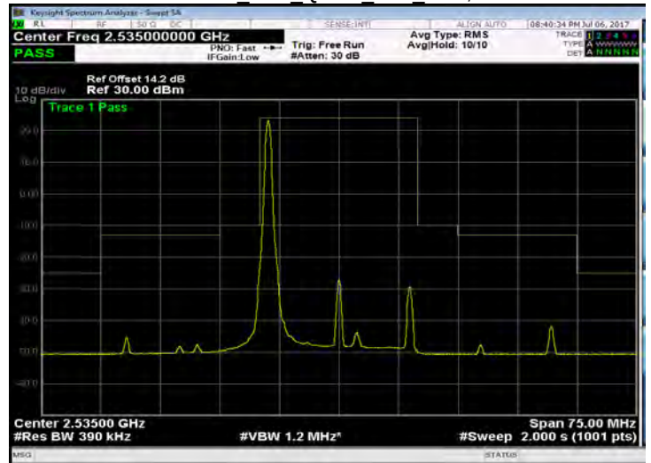
Band 7 20M QPSK MID RB1,99
