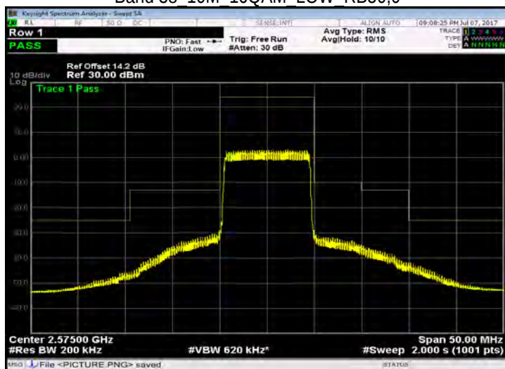
Band 38 10M 16QAM LOW RB50,0
