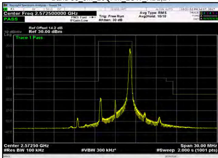
Band 38 5M 16QAM LOW RB25,0
