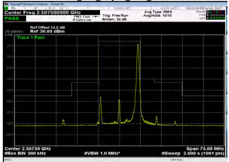
Band 7 15M 16QAM LOW RB75,0
