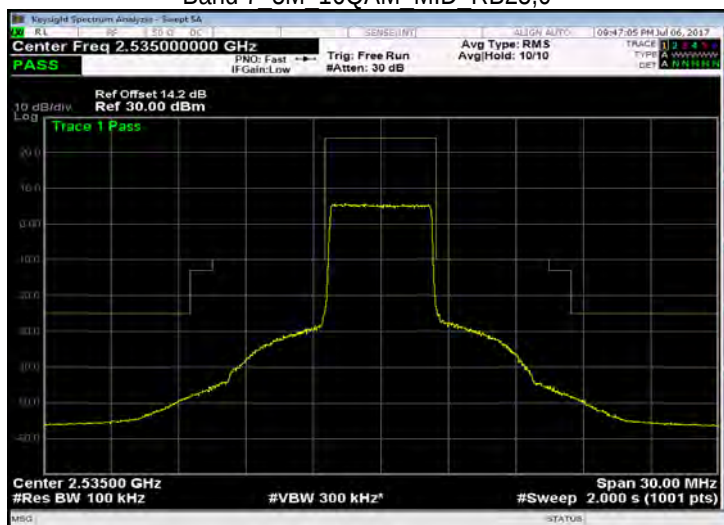
Band 7 5M 16QAM MID RB25,0
