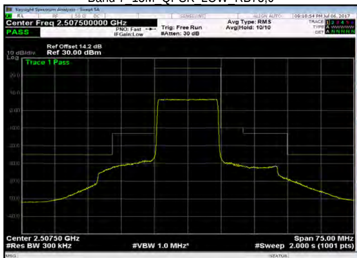
Band 7 15M QPSK LOW RB75,0
