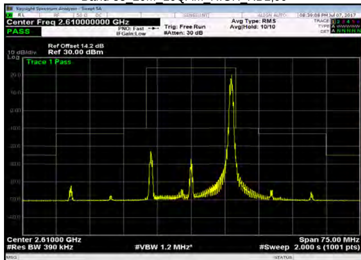
Band 38 20M 16QAM HIGH RB100,0
