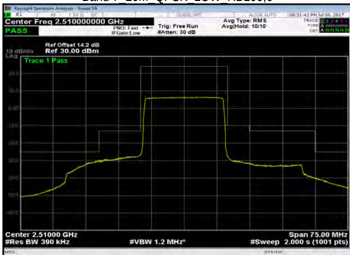
Band 7 20M QPSK LOW RB100,0
