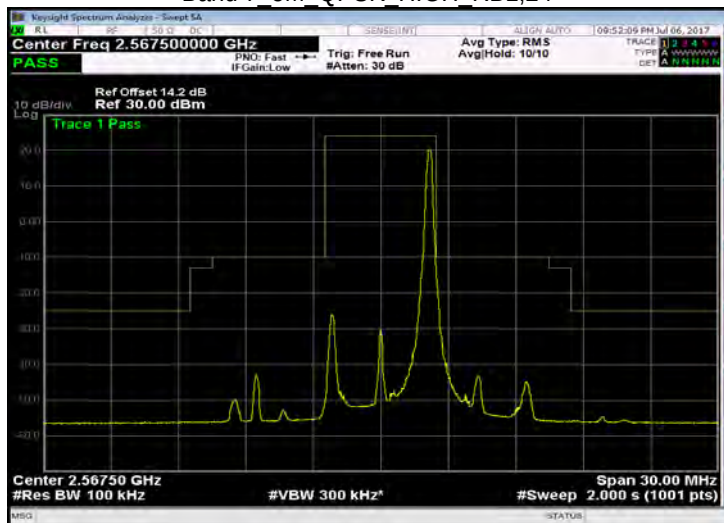
Band 7 5M QPSK HIGH RB25,0
