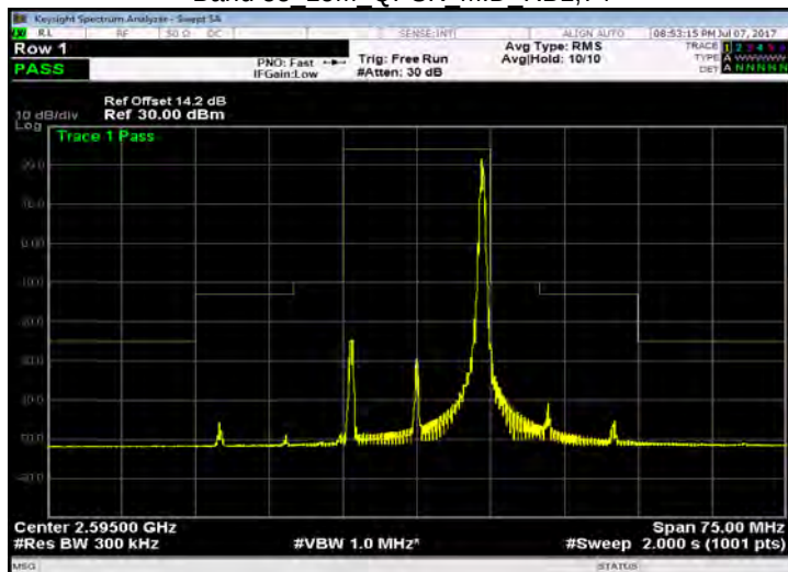
Band 38 15M QPSK MID RB75,0
