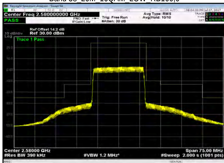
Band 38 20M 16QAM LOW RB100,0
