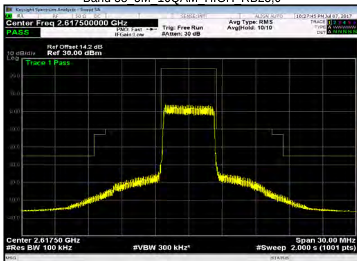
Band 38 5M 16QAM HIGH RB25,0
