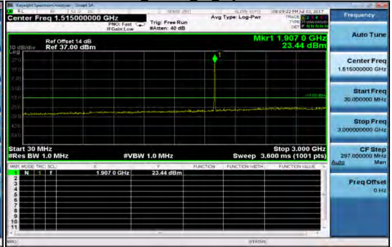
30MHz~3GHz HSDPA B2 HighCH9538-1907.6
