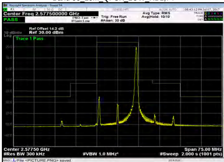
Band 38 15M QPSK LOW RB75,0
