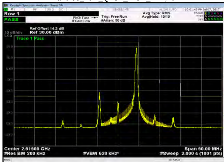
Band 38 10M QPSK HIGH RB50,0
