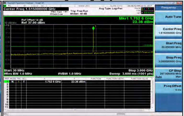
30MHz~3GHz WCDMA B4 HighCH1513-1752.6
