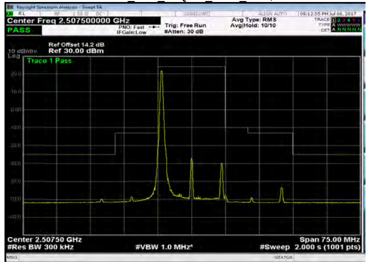
Band 7 15M 16QAM LOW RB1,74
