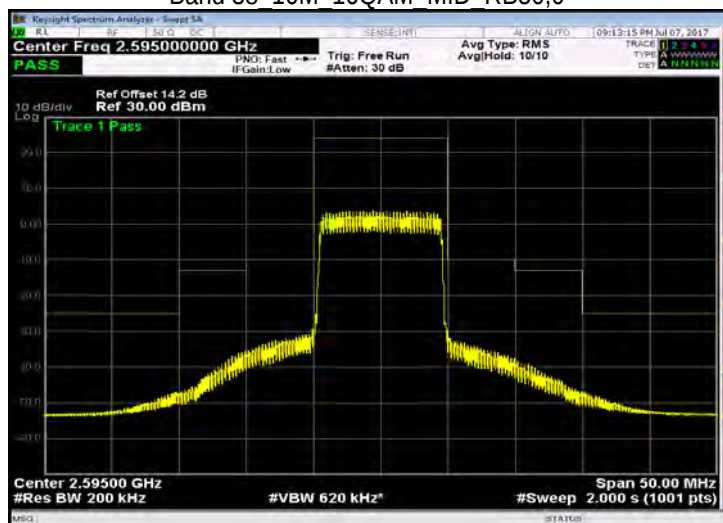
Band 38 10M 16QAM MID RB50,0
