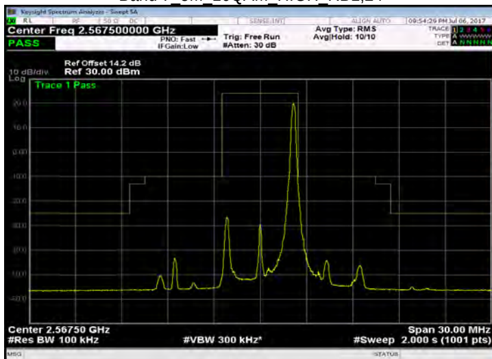
Band 7 5M 16QAM HIGH RB25,0
