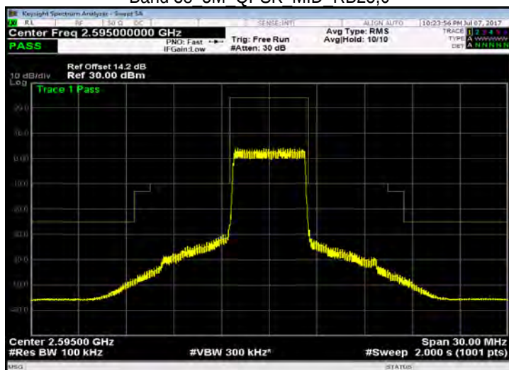
Band 38 5M QPSK MID RB25,0
