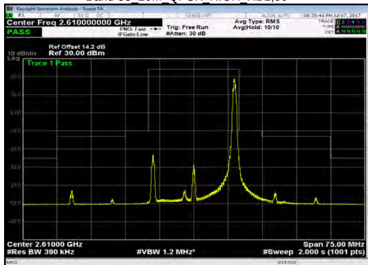
Band 38 20M QPSK HIGH RB100,0
