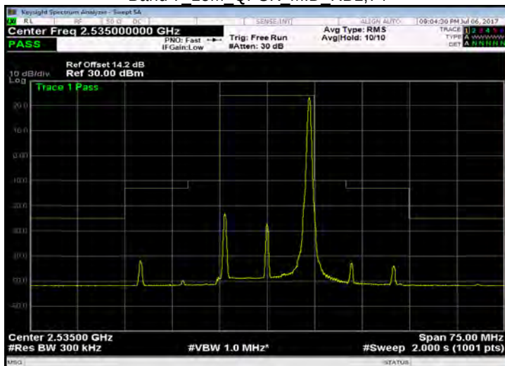
Band 7 15M QPSK MID RB75,0
