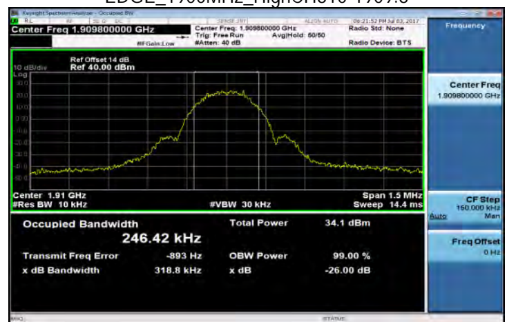
EDGE_1900MHz_HighCH810-1909.8
