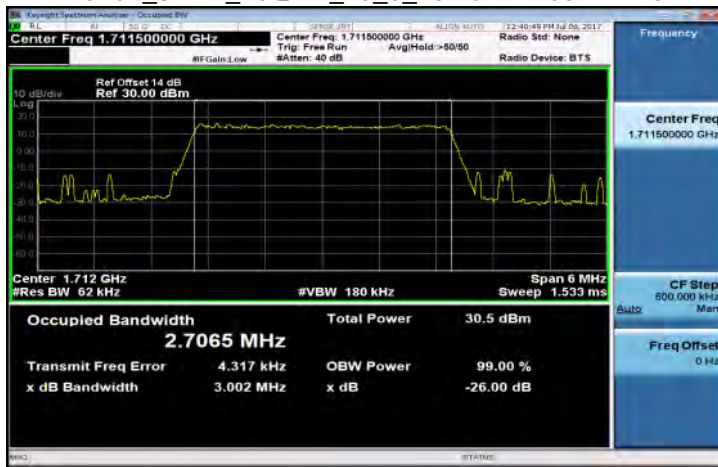
Band4_3MHz_16QAM_15_0_LowCH19965-1711.5
