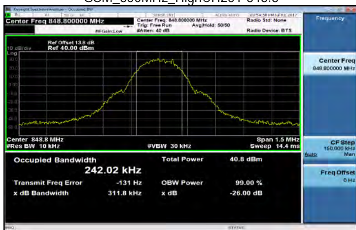
GSM_850MHz_HighCH251-848.8
