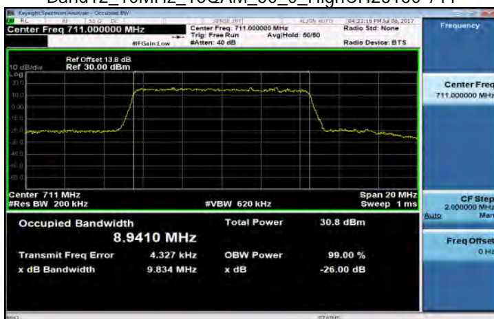
Band12_10MHz_16QAM_50_0_HighCH23130-711
