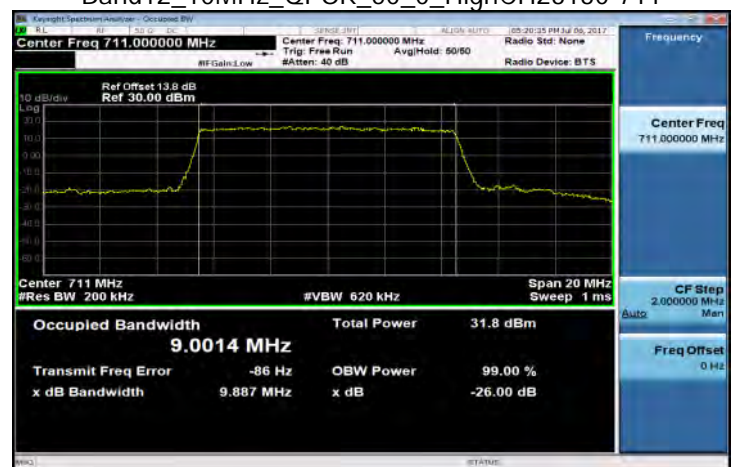
Band12_10MHz_QPSK_50_0_HighCH23130-711
