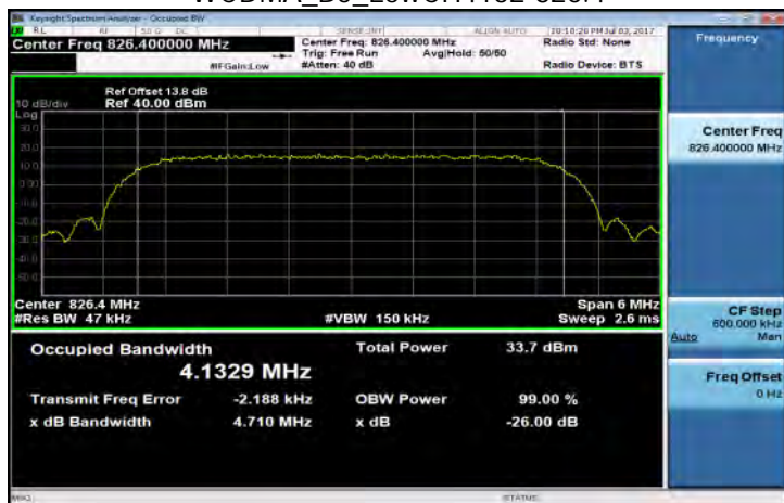
WCDMA_B5_LowCH4132-826.4
