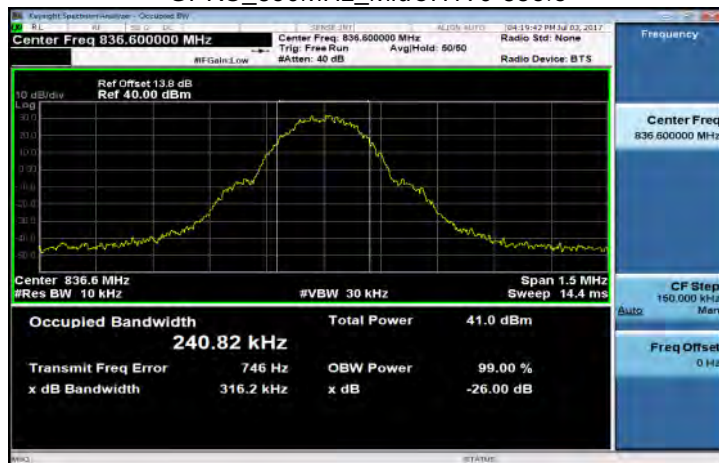
GPRS_850MHz_MidCH190-836.6
