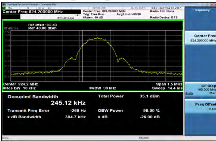
EDGE_850MHz_LowCH128-824.2
