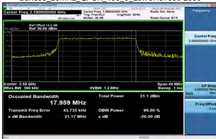
Band38_20MHz_QPSK_100_0_LowCH37850-2580
