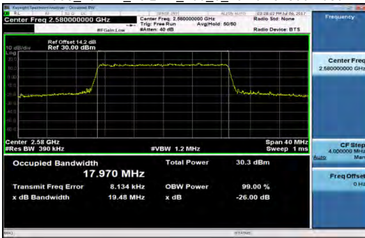
Band38_20MHz_16QAM_100_0_LowCH37850-2580
