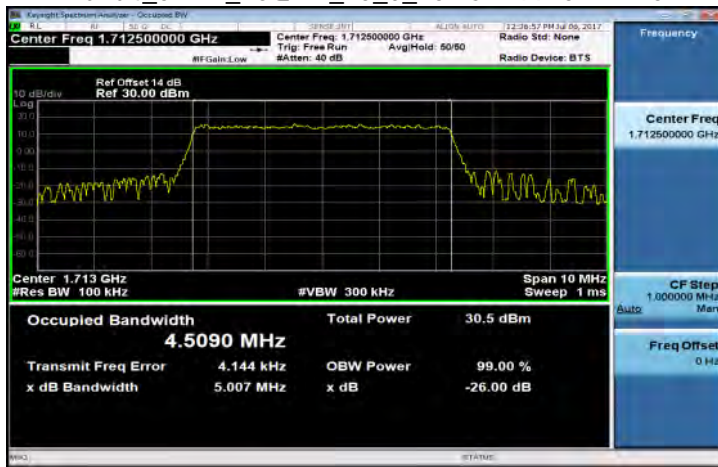
Band4_5MHz_16QAM_25_0_LowCH19975-1712.5
