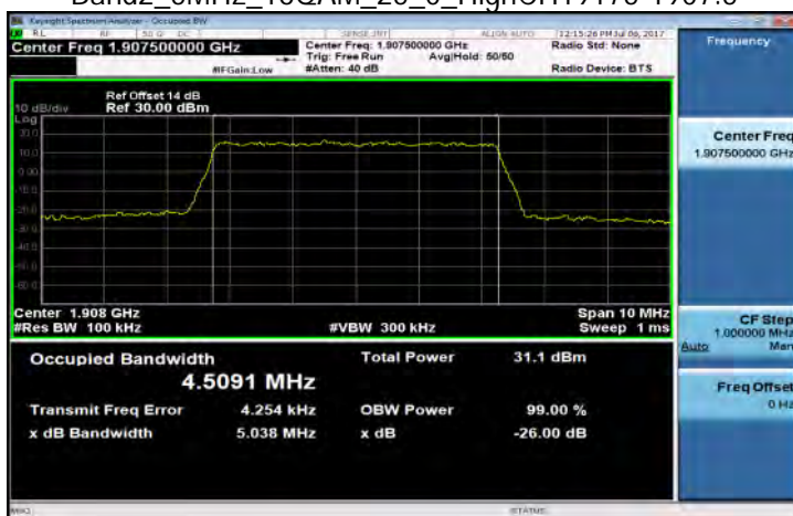
Band2_5MHz_16QAM_25_0_HighCH19175-1907.5
