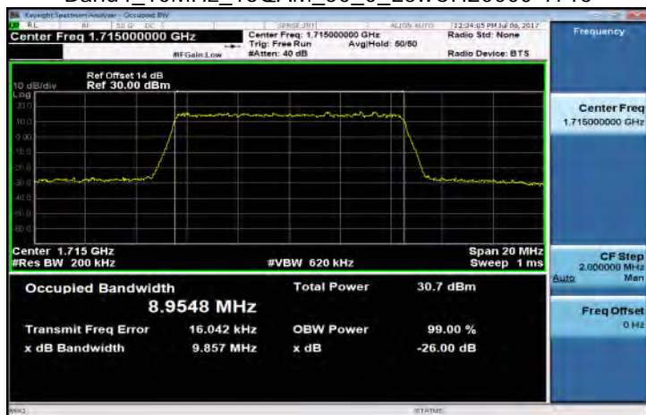
Band4_10MHz_16QAM_50_0_LowCH20000-1715
