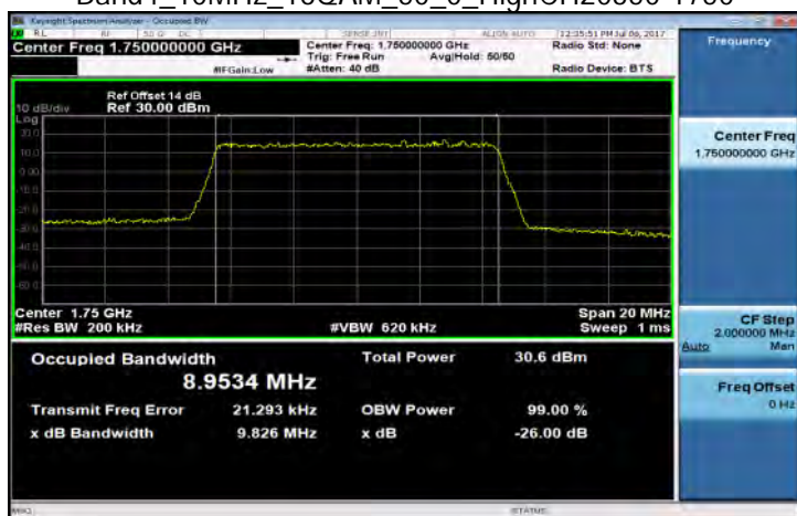
Band4_10MHz_16QAM_50_0_HighCH20350-1750
