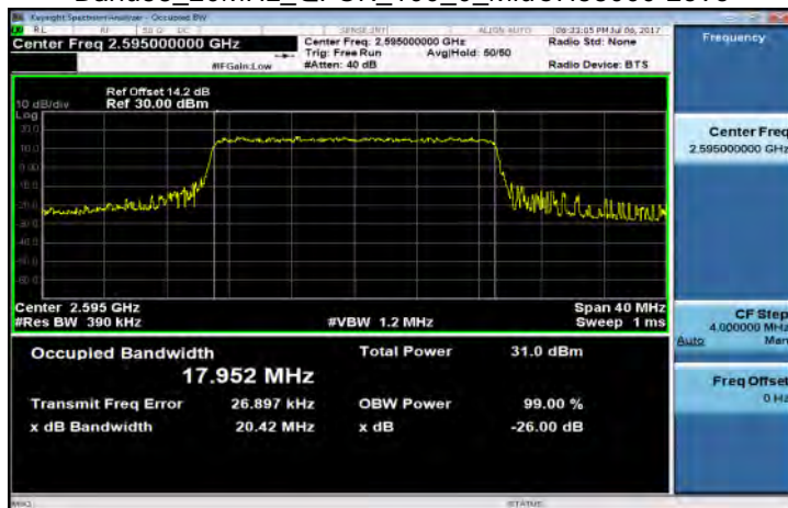
Band38_20MHz_QPSK_100_0_MidCH38000-2595
