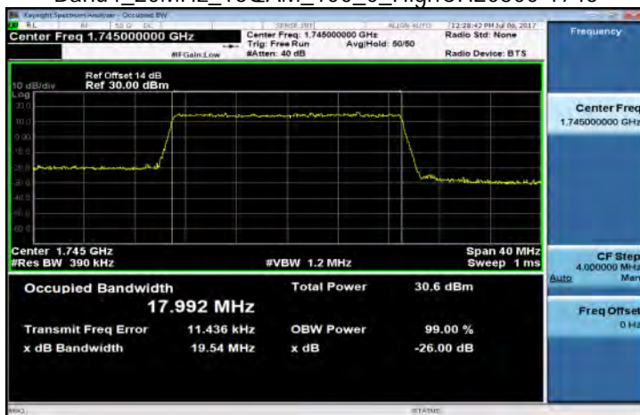
Band4_20MHz_16QAM_100_0_HighCH20300-1745
