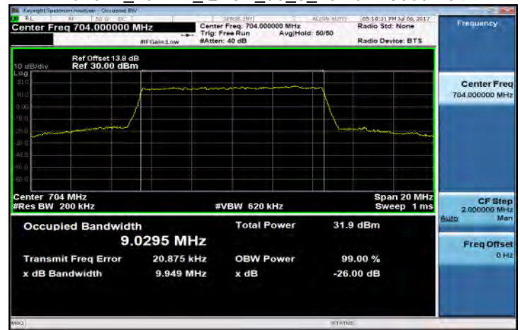
Band12_10MHz_QPSK_50_0_LowCH23060-704
