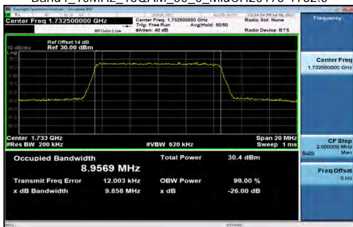
Band4_10MHz_16QAM_50_0_MidCH20175-1732.5
