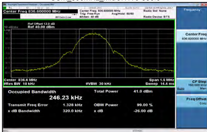
GSM_850MHz_MidCH190-836.6
