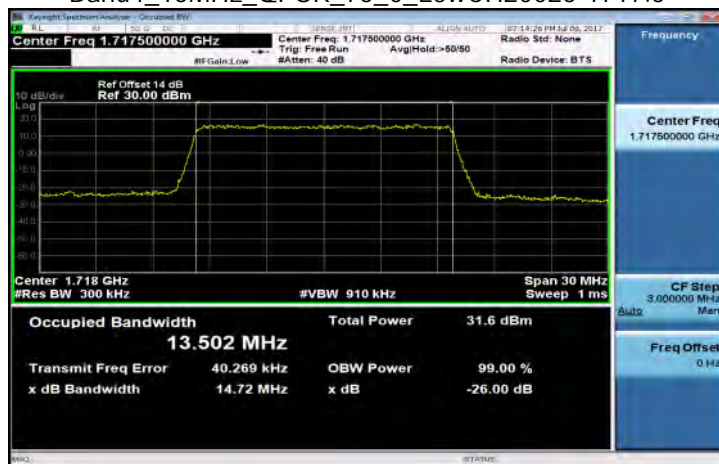
Band4_15MHz_QPSK_75_0_LowCH20025-1717.5
