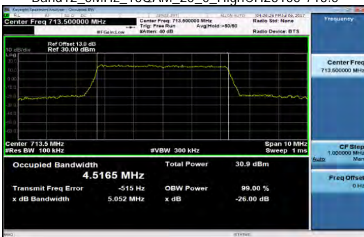
Band12_5MHz_16QAM_25_0_HighCH23155-713.5
