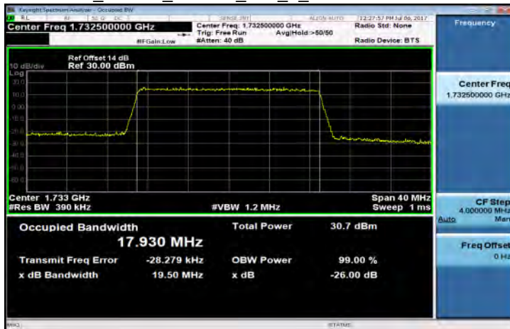
Band4_20MHz_16QAM_100_0_MidCH20175-1732.5
