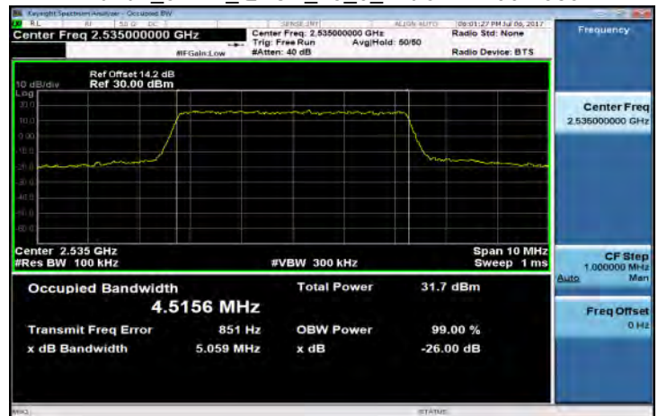
Band7_5MHz_QPSK_25_0_MidCH21100-2535
