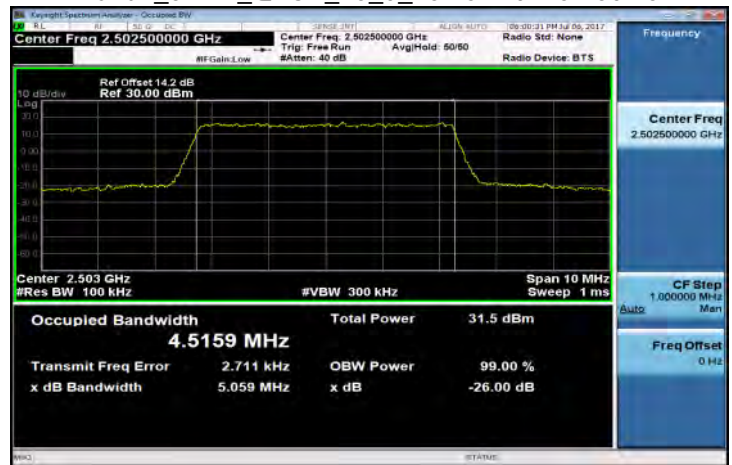
Band7_5MHz_QPSK_25_0_LowCH20775-2502.5
