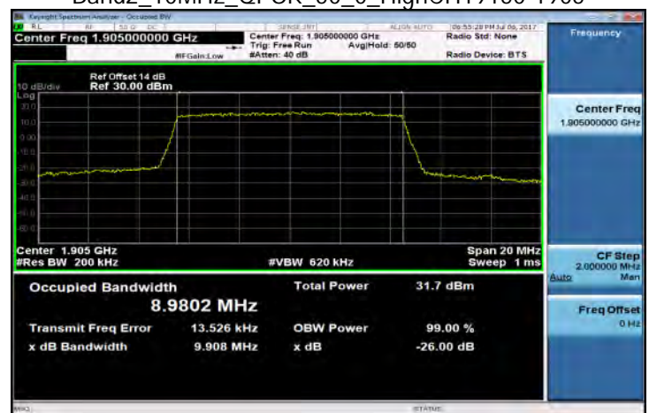
Band2_10MHz_QPSK_50_0_HighCH19150-1905
