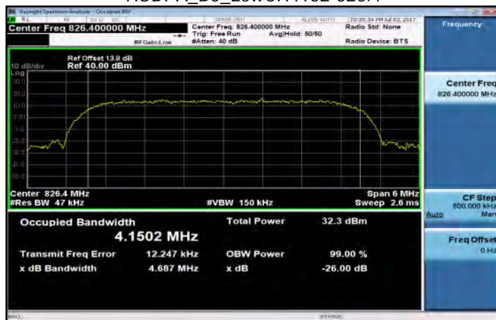
HSDPA_B5_LowCH4132-826.4
