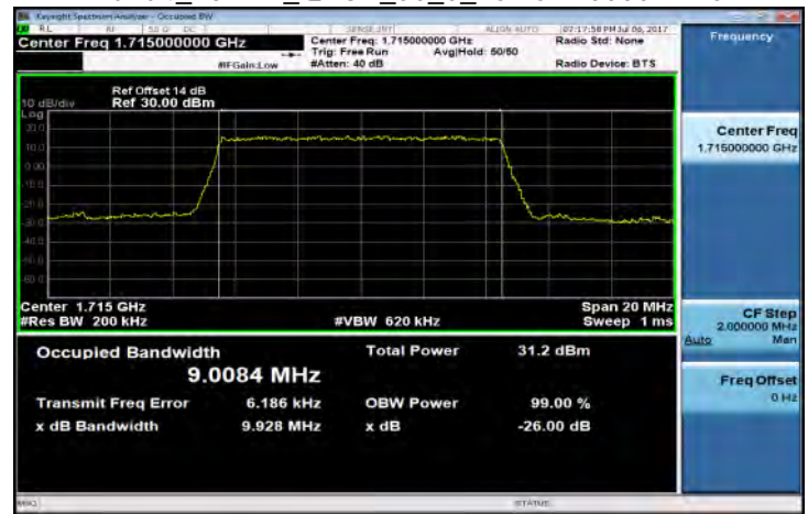
Band4_10MHz_QPSK_50_0_LowCH20000-1715
