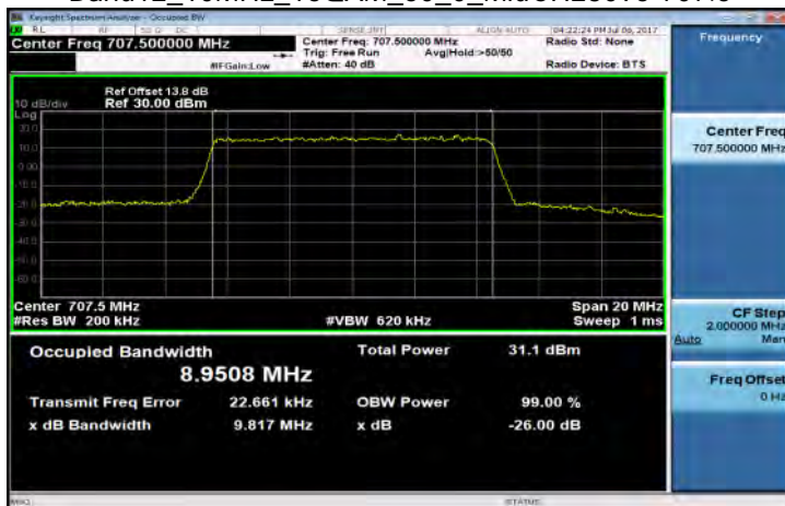
Band12_10MHz_16QAM_50_0_MidCH23095-707.5
