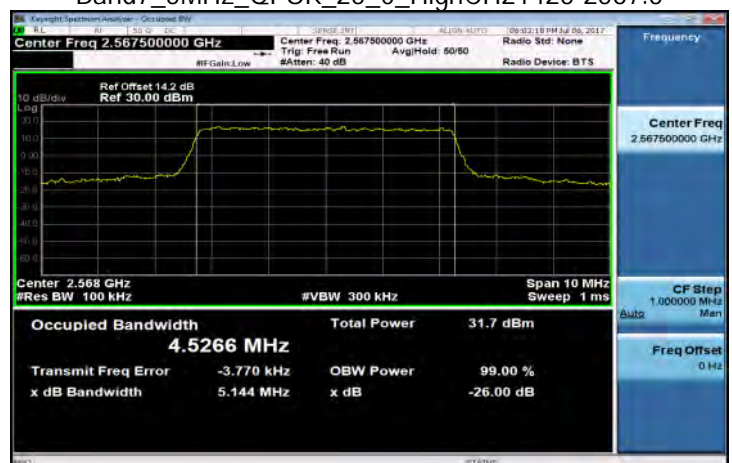
Band7_5MHz_QPSK_25_0_HighCH21425-2567.5
