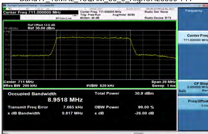
Band17_10MHz_16QAM_50_0_HighCH23800-711
