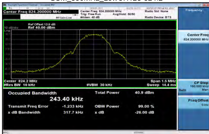
GSM_850MHz_LowCH128-824.2
