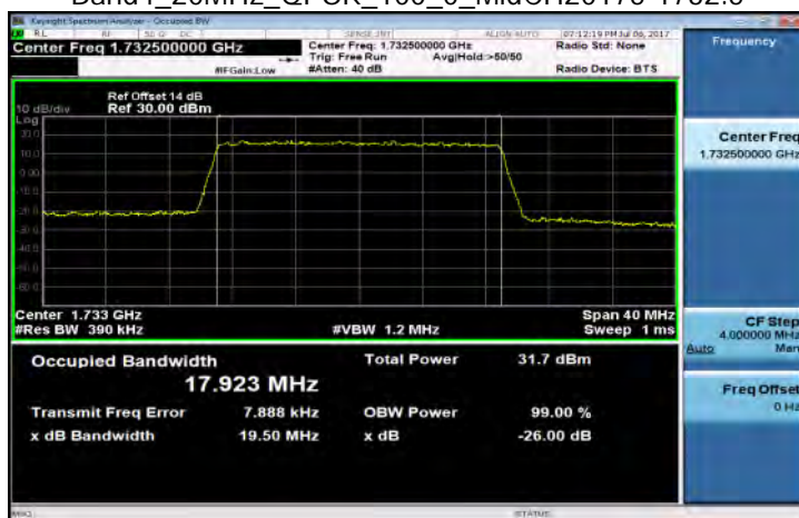
Band4_20MHz_QPSK_100_0_MidCH20175-1732.5
