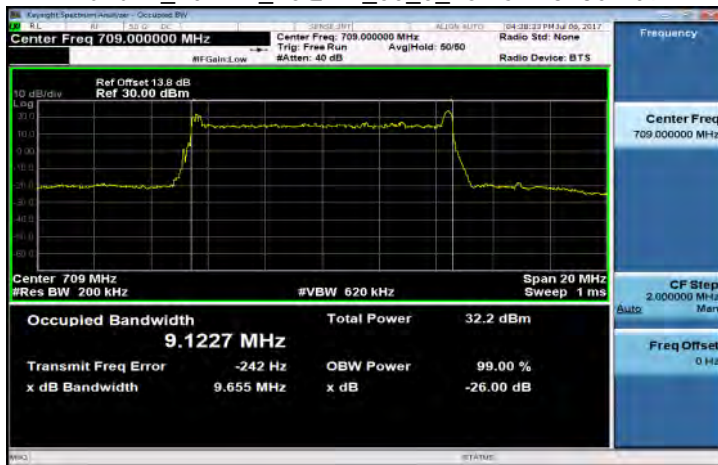
Band17_10MHz_16QAM_50_0_LowCH23780-709
