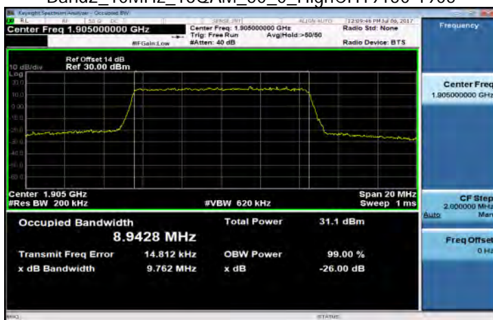
Band2_10MHz_16QAM_50_0_HighCH19150-1905
