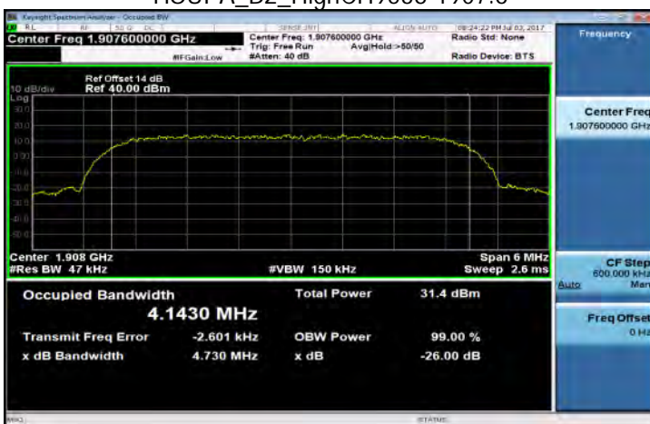
HSUPA_B2_HighCH9538-1907.6
