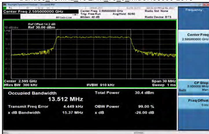
Band38_15MHz_16QAM_75_0_MidCH38000-2595
