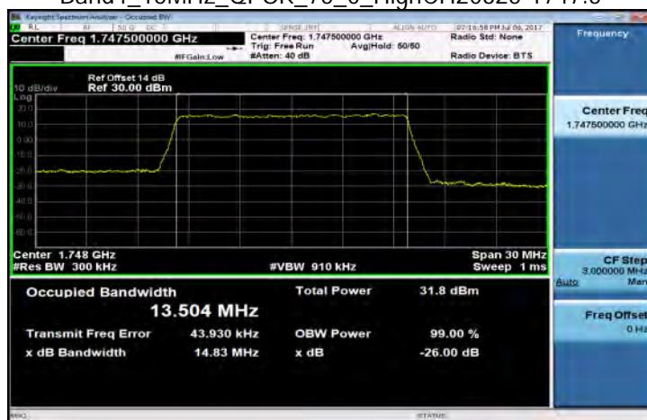
Band4_15MHz_QPSK_75_0_HighCH20325-1747.5
