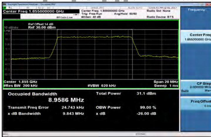
Band2_10MHz_16QAM_50_0_LowCH18650-1855
