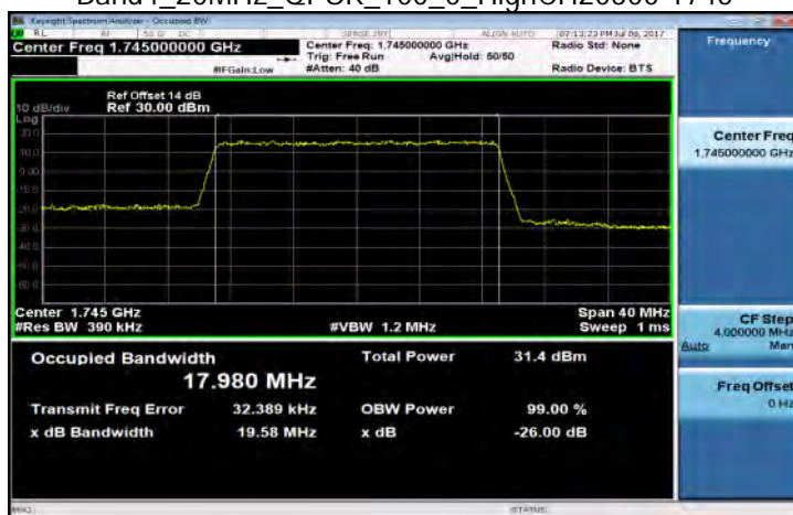
Band4_20MHz_QPSK_100_0_HighCH20300-1745
