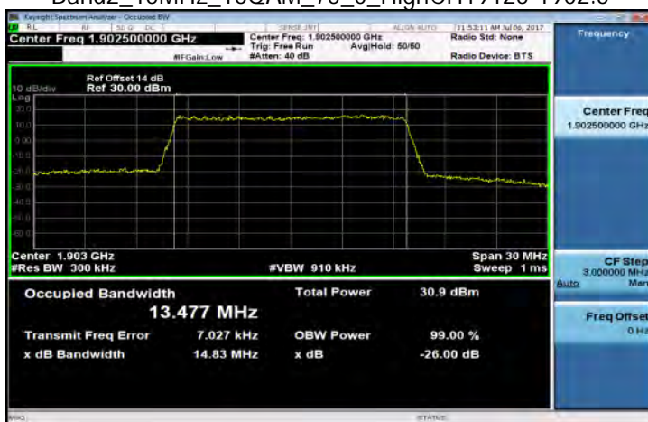
Band2_15MHz_16QAM_75_0_HighCH19125-1902.5
