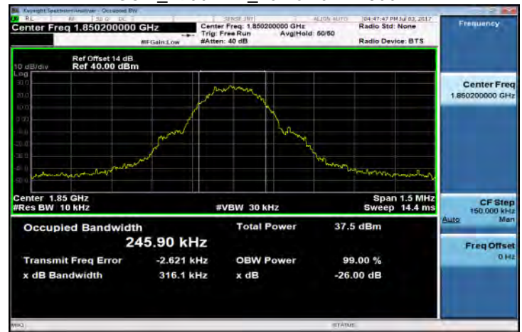
GSM_1900MHz_LowCH512-1850.2
