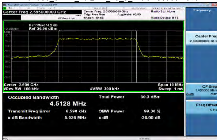
Band38_5MHz_16QAM_25_0_MidCH38000-2595
