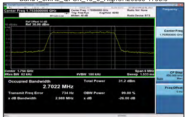
Band4_3MHz_QPSK_15_0_HighCH20385-1753.5
