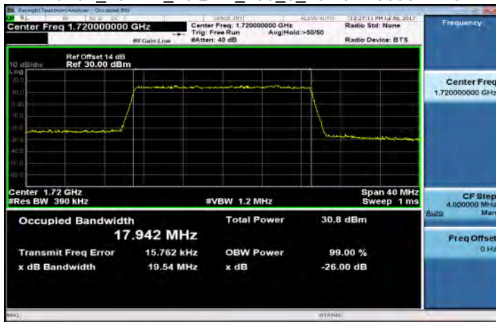
Band4_20MHz_16QAM_100_0_LowCH20050-1720
