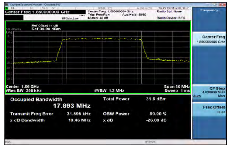
Band2_20MHz_QPSK_100_0_LowCH18700-1860
