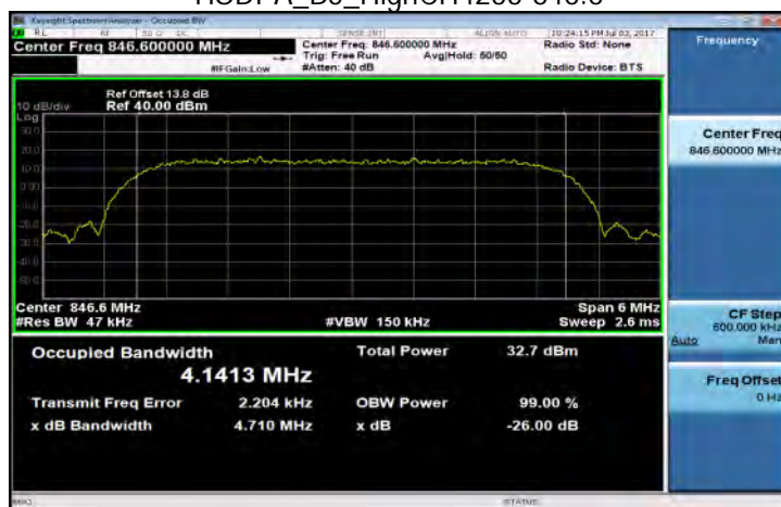
HSDPA_B5_HighCH4233-846.6
