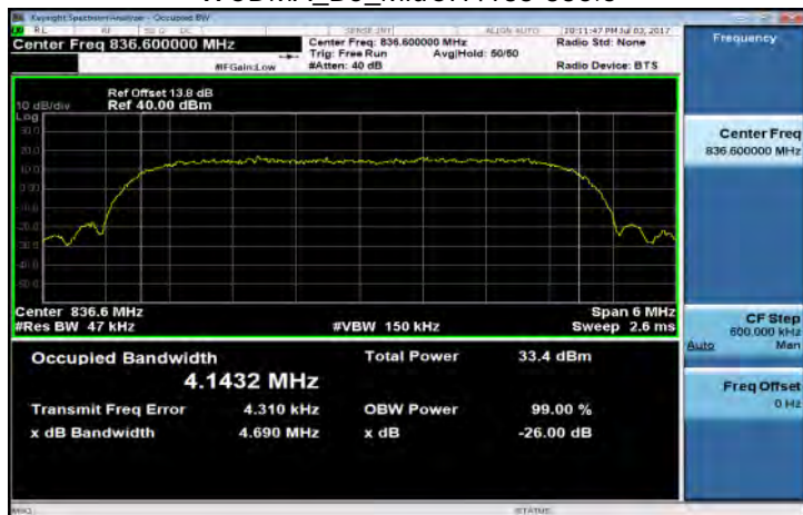
WCDMA_B5_MidCH4183-836.6
