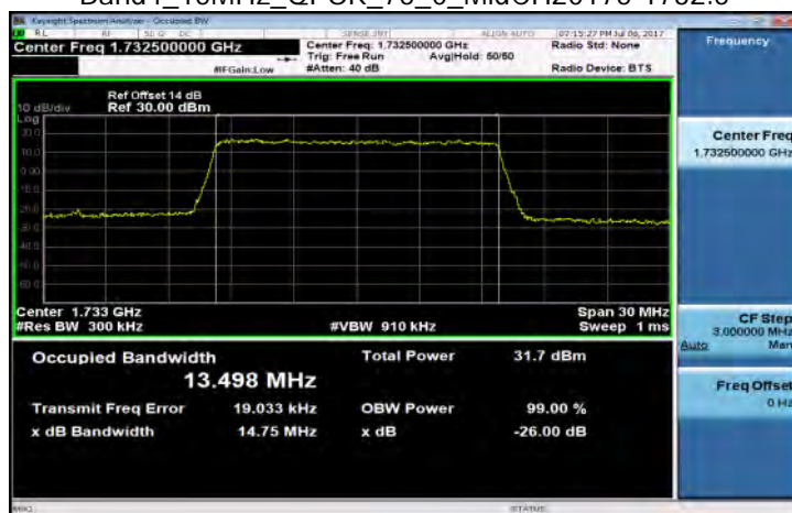
Band4_15MHz_QPSK_75_0_MidCH20175-1732.5
