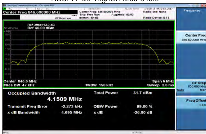
HSUPA_B5_HighCH4233-846.6
