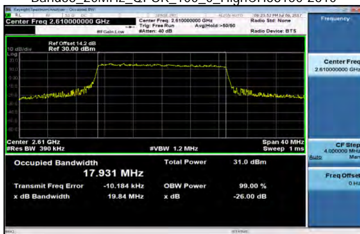
Band38_20MHz_QPSK_100_0_HighCH38150-2610
