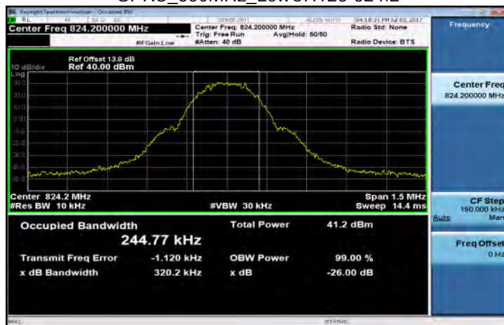
GPRS_850MHz_LowCH128-824.2
