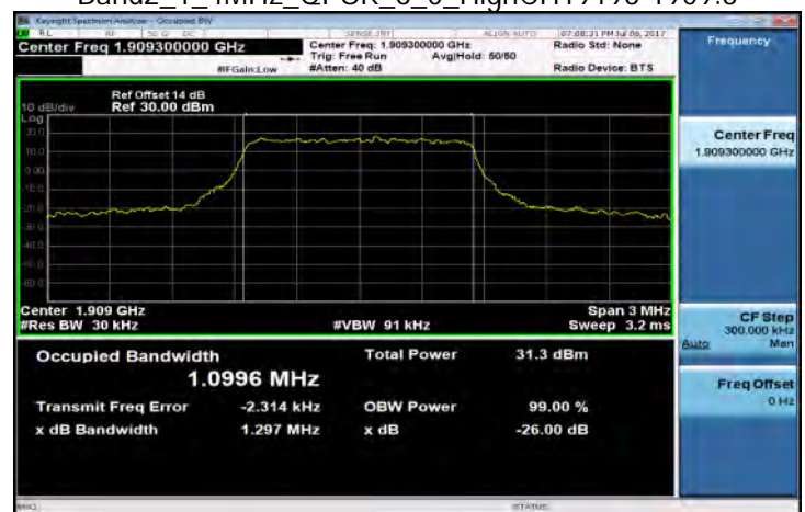
Band2_1_4MHz_QPSK_6_0_HighCH19193-1909.3
