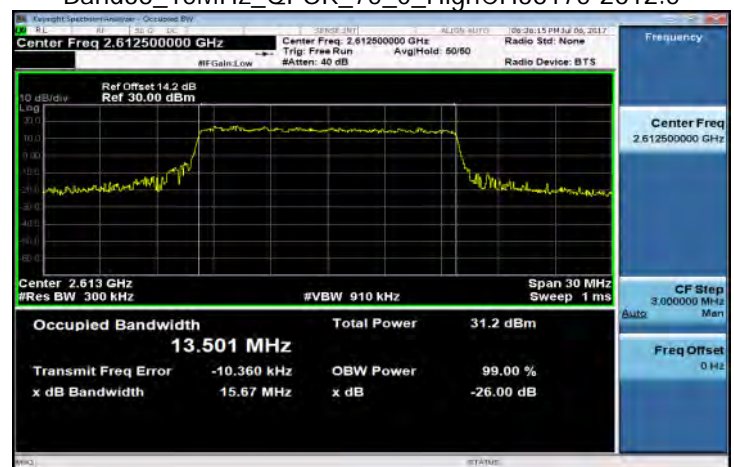
Band38_15MHz_QPSK_75_0_HighCH38175-2612.5
