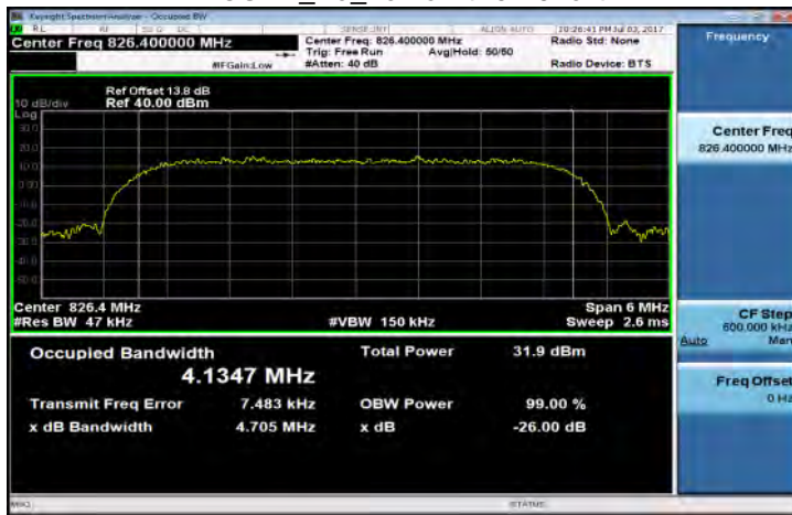
HSUPA_B5_LowCH4132-826.4
