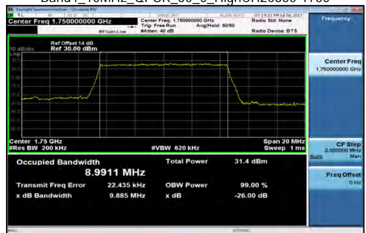
Band4_10MHz_QPSK_50_0_HighCH20350-1750
