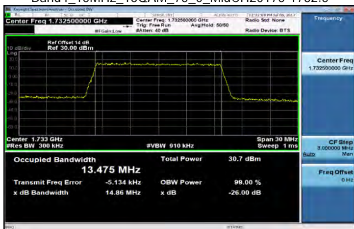
Band4_15MHz_16QAM_75_0_MidCH20175-1732.5
