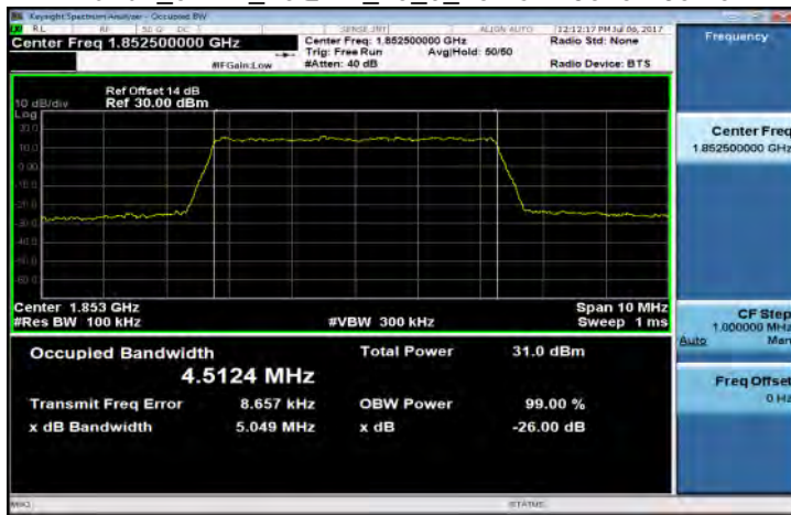
Band2_5MHz_16QAM_25_0_LowCH18625-1852.5
