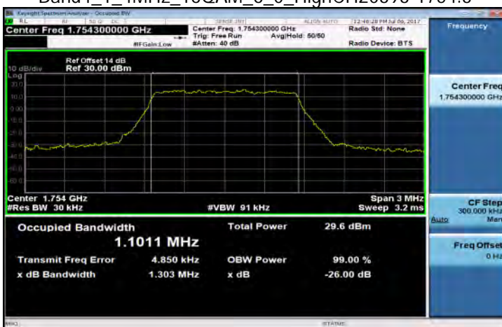
Band4_1_4MHz_16QAM_6_0_HighCH20393-1754.3
