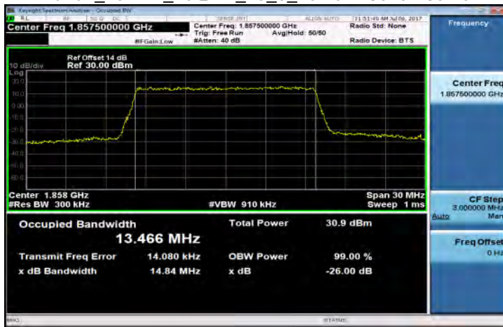
Band2_15MHz_16QAM_75_0_LowCH18675-1857.5
