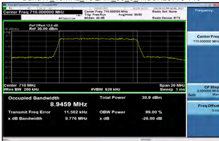
Band17_10MHz_16QAM_50_0_MidCH23790-710
