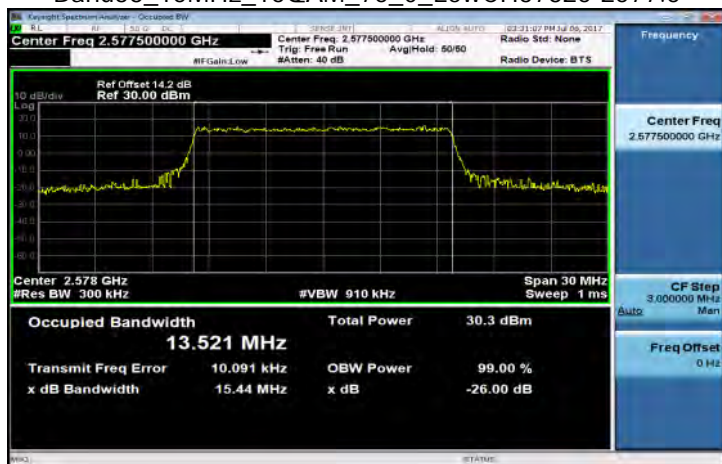
Band38_15MHz_16QAM_75_0_LowCH37825-2577.5
