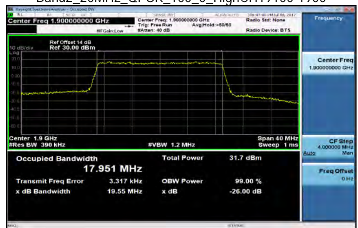
Band2_20MHz_QPSK_100_0_HighCH19100-1900
