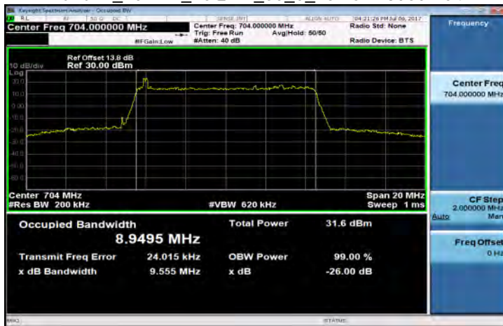
Band12_10MHz_16QAM_50_0_LowCH23060-704
