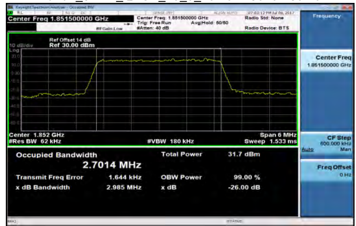
Band2_3MHz_QPSK_15_0_LowCH18615-1851.5
