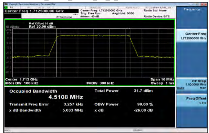
Band4_5MHz_QPSK_25_0_LowCH19975-1712.5
