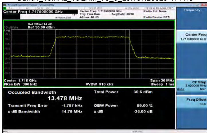
Band4_15MHz_16QAM_75_0_LowCH20025-1717.5
