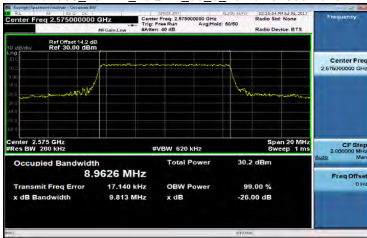
Band38_10MHz_16QAM_50_0_LowCH37800-2575
