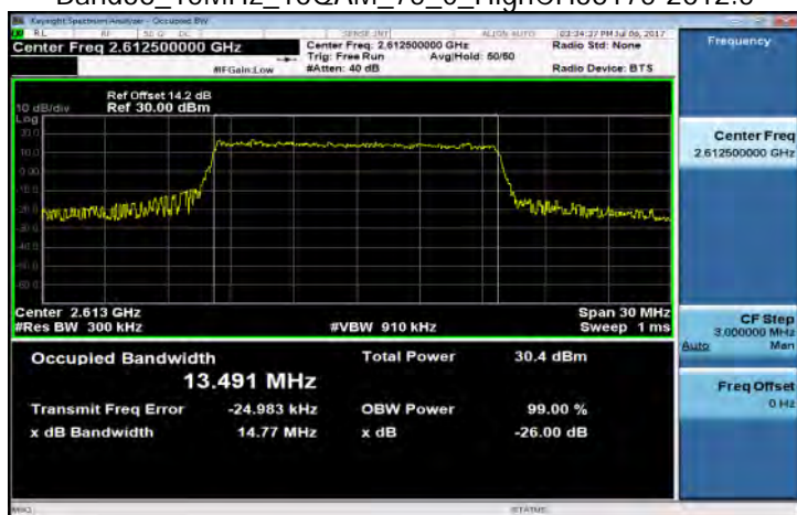
Band38_15MHz_16QAM_75_0_HighCH38175-2612.5
