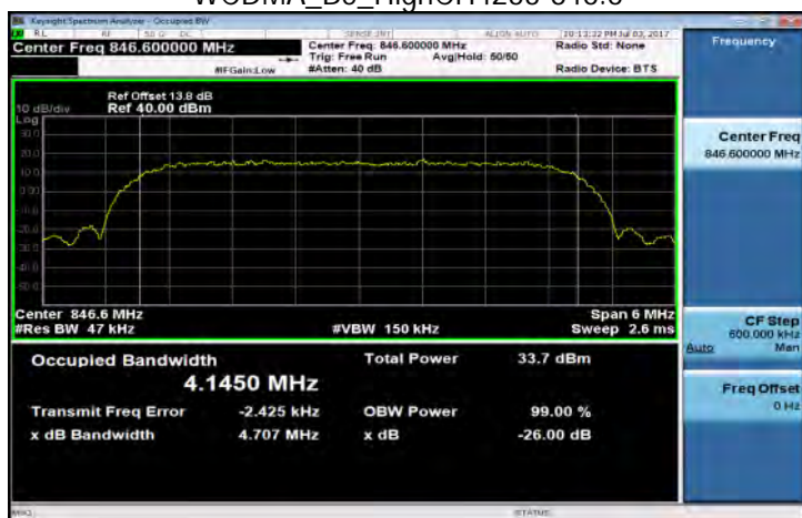
WCDMA_B5_HighCH4233-846.6
