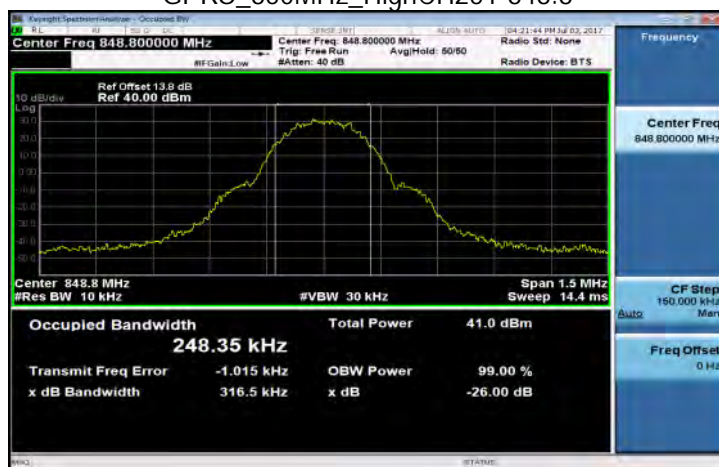
GPRS_850MHz_HighCH251-848.8
