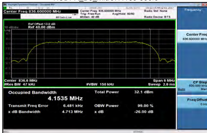
HSDPA_B5_MidCH4183-836.6
