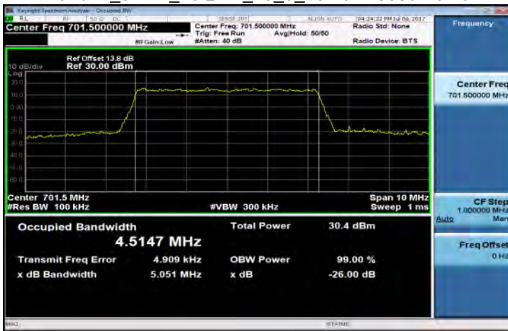
Band12_5MHz_16QAM_25_0_LowCH23035-701.5
