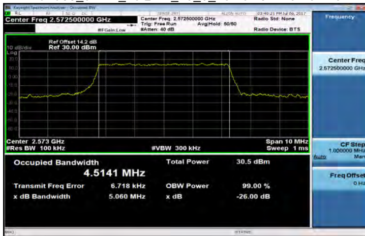
Band38_5MHz_16QAM_25_0_LowCH37775-2572.5
