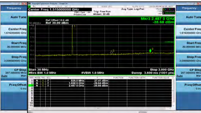
Out of Band Emission Low_Band5 10MHz_QPSK 1 0_MidCH20525-836.5
