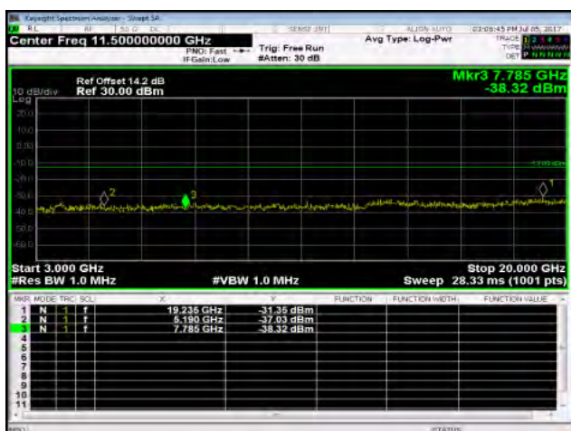
Out of Band Emission High Band38 5MHz QPSK 1 0 HighCH38225-2617.5
