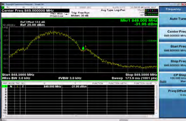
Band Edge_GPRS_850MHz_HighCH251-848.8
