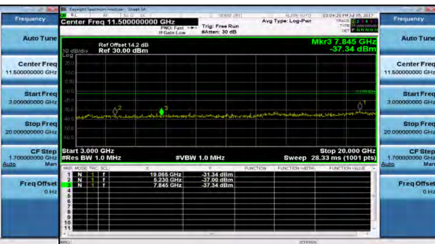
Out of Band Emission High Band38 10MHz QPSK 1 0 HighCH38200-2615
