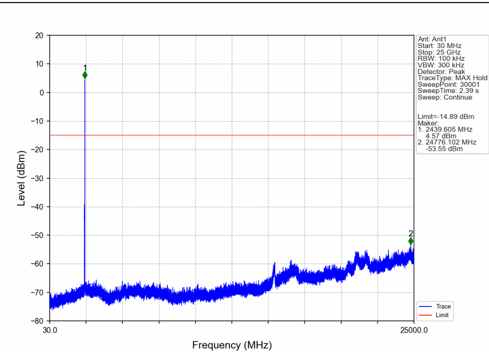
1M_MCH_2440MHz_Ant1_NTNV
