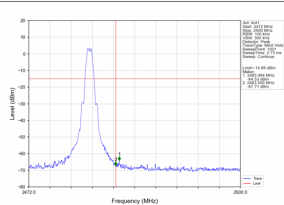
1M_HCH_2480MHz_Ant1_NTNV
